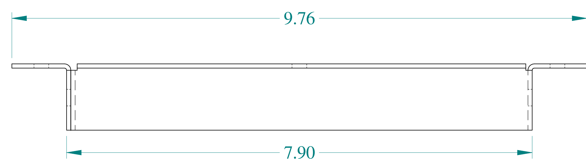
TOP VIEW
