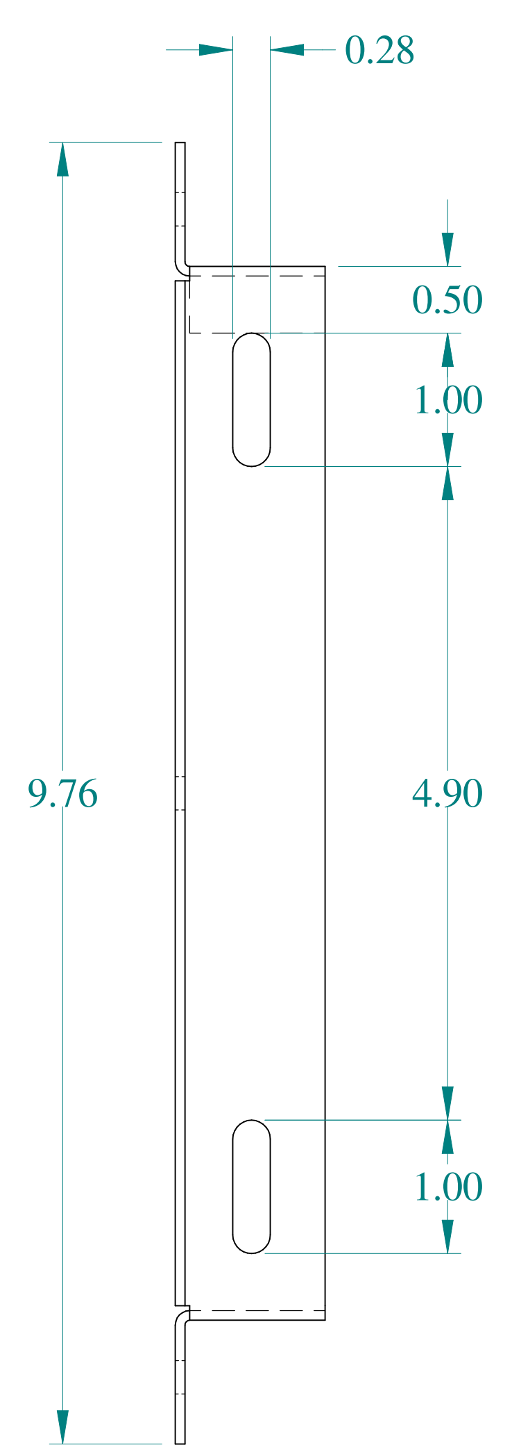
SIDE VIEW
