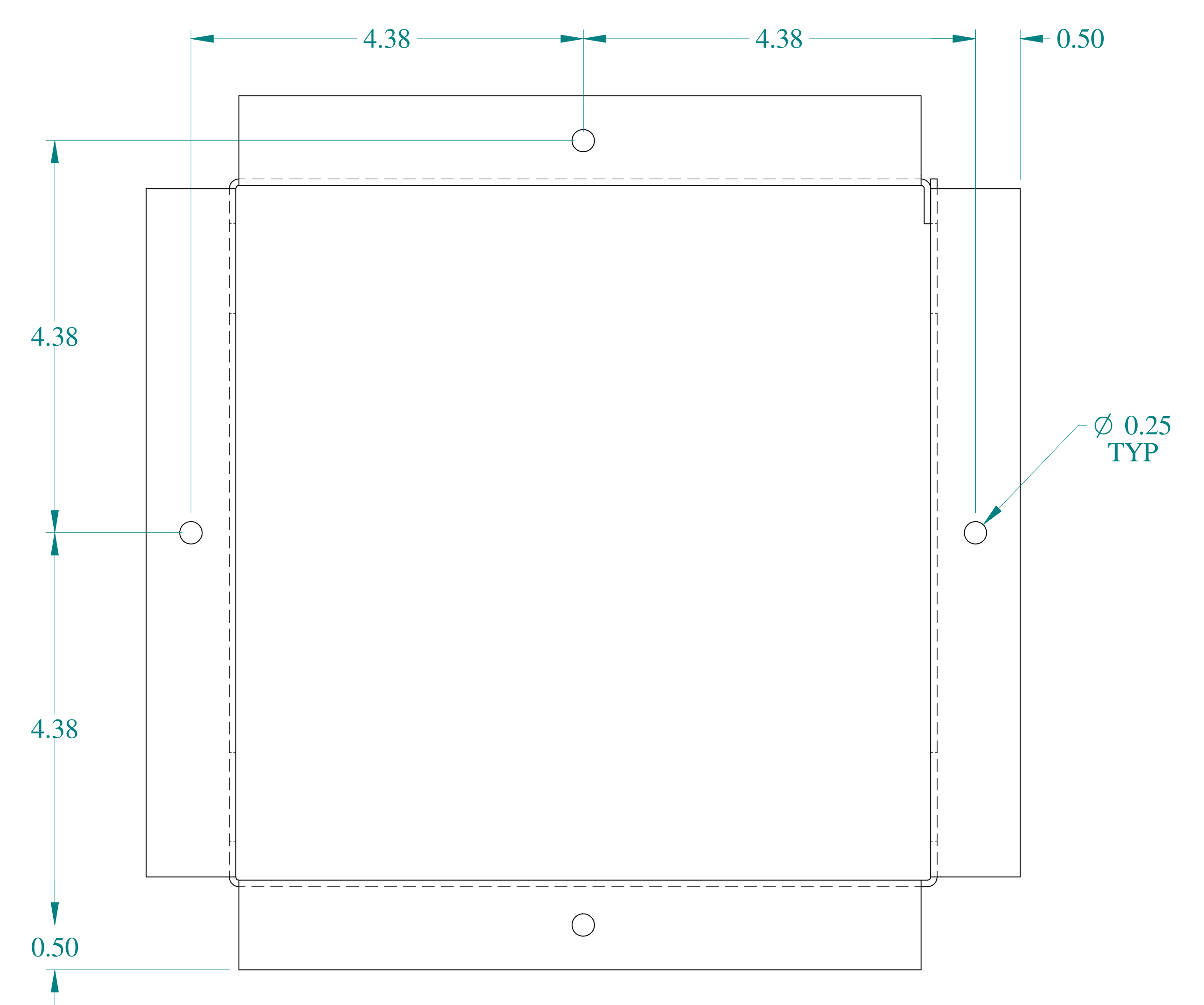
BACK VIEW
