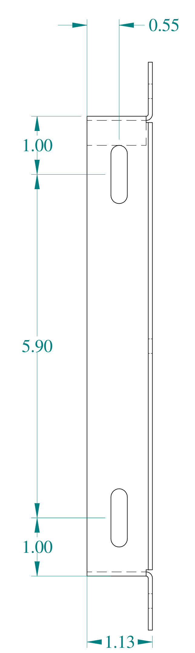
SIDE VIEW
