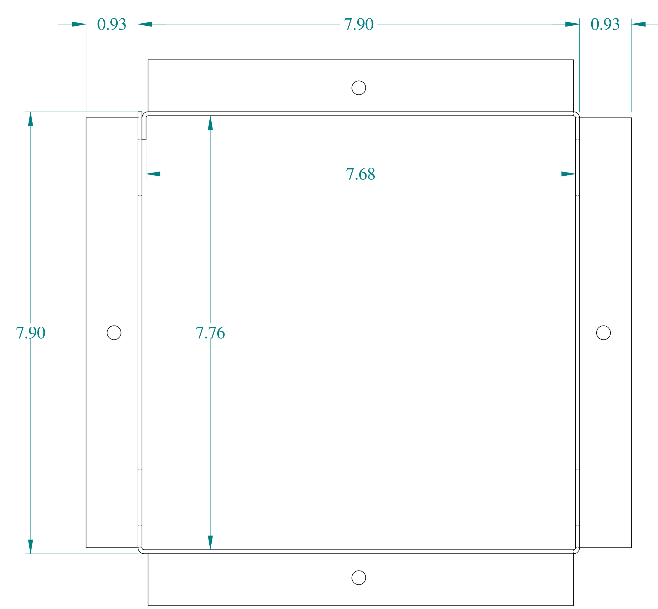
FRONT VIEW
