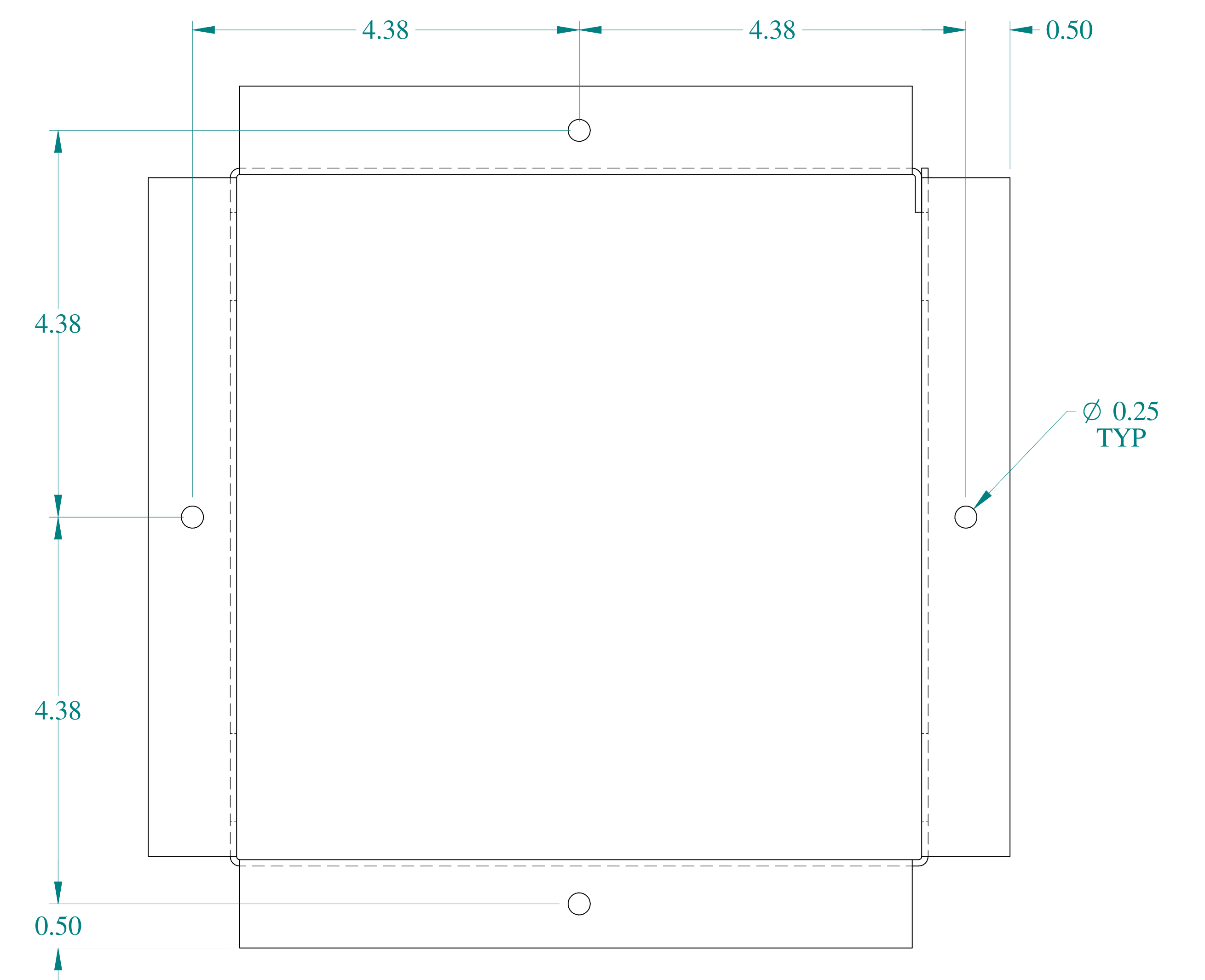
BACK VIEW
