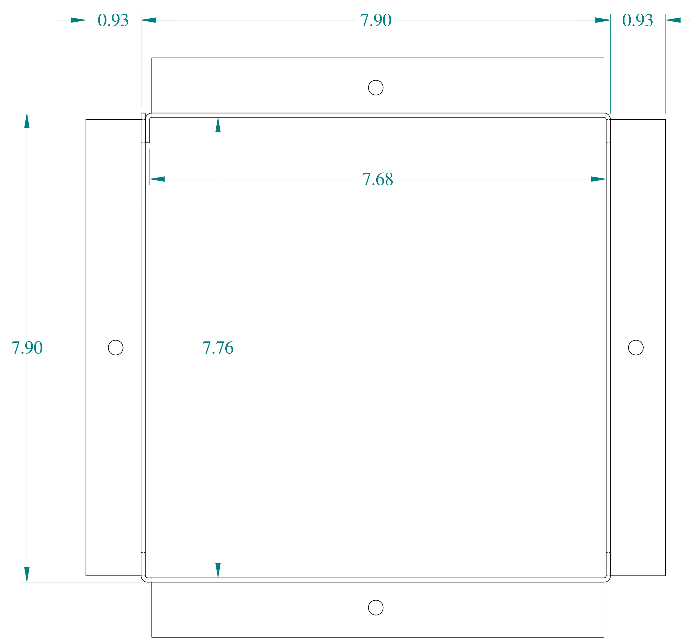
FRONT VIEW
