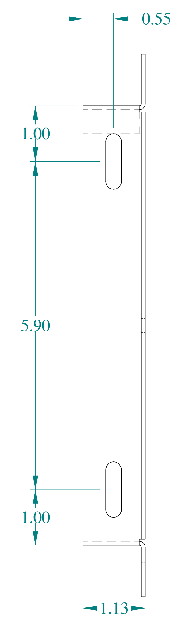
SIDE VIEW
