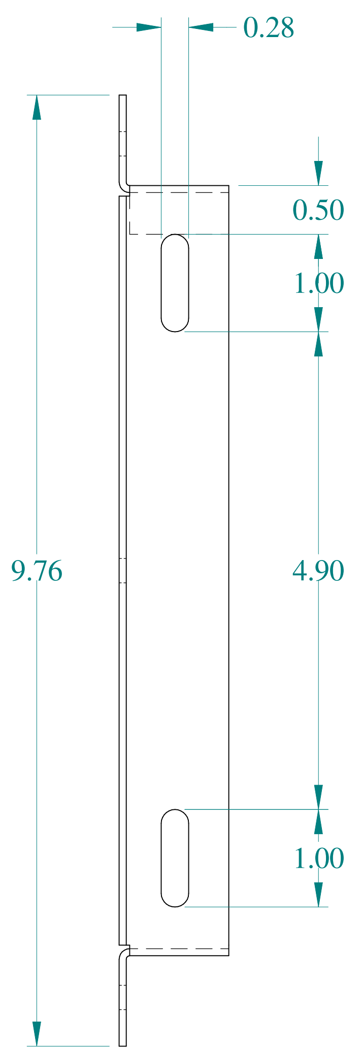
SIDE VIEW
