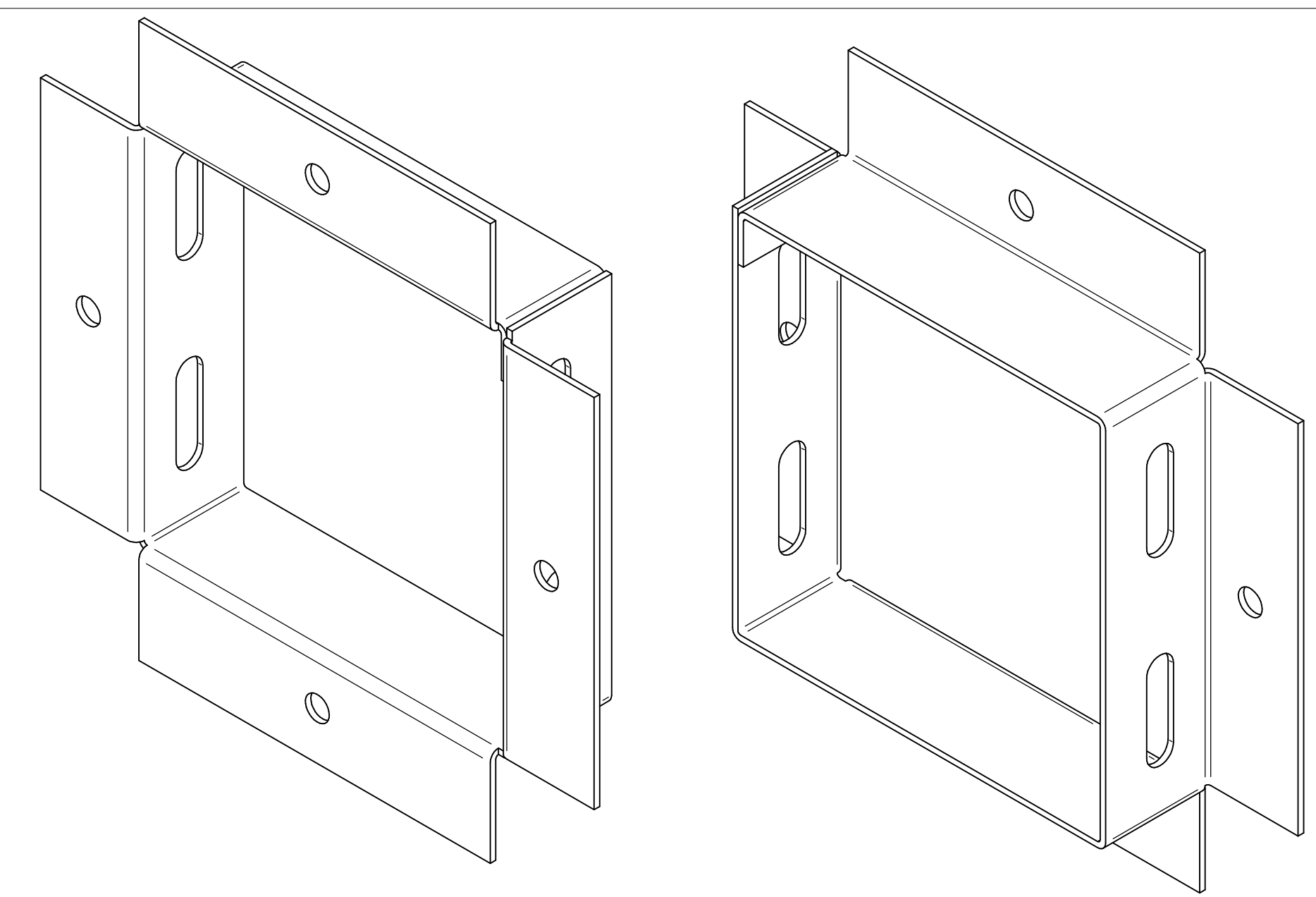
ISOMETRIC VIEWS
