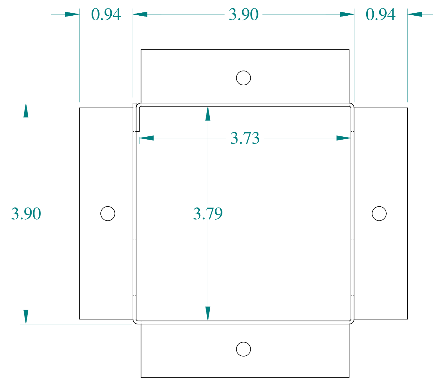
FRONT VIEW
