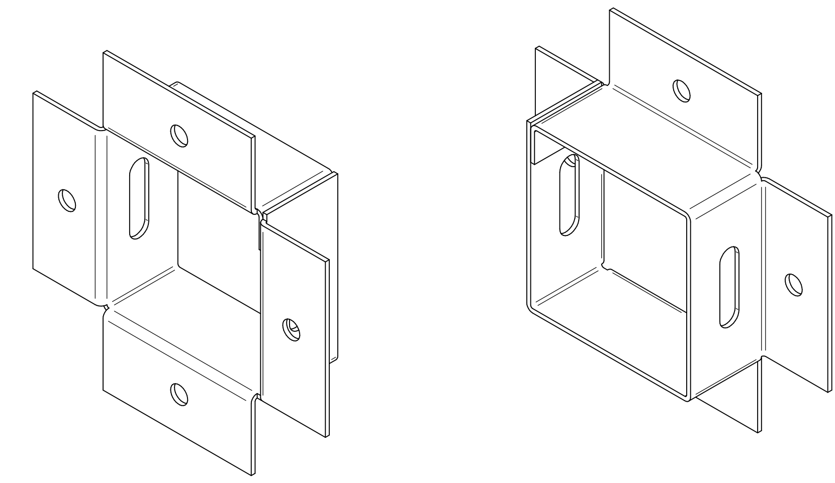
ISOMETRIC VIEWS
