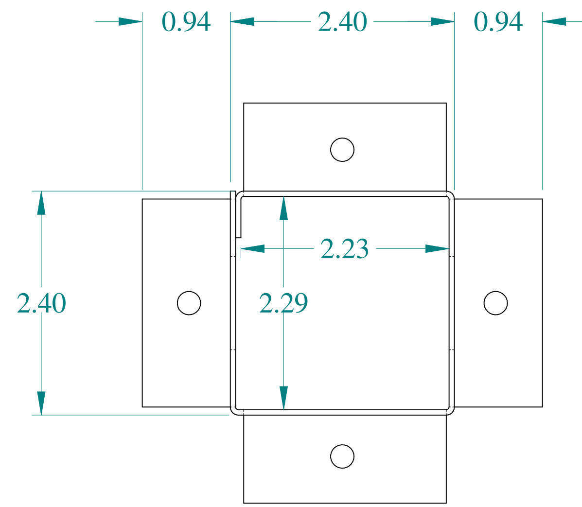
FRONT VIEW
