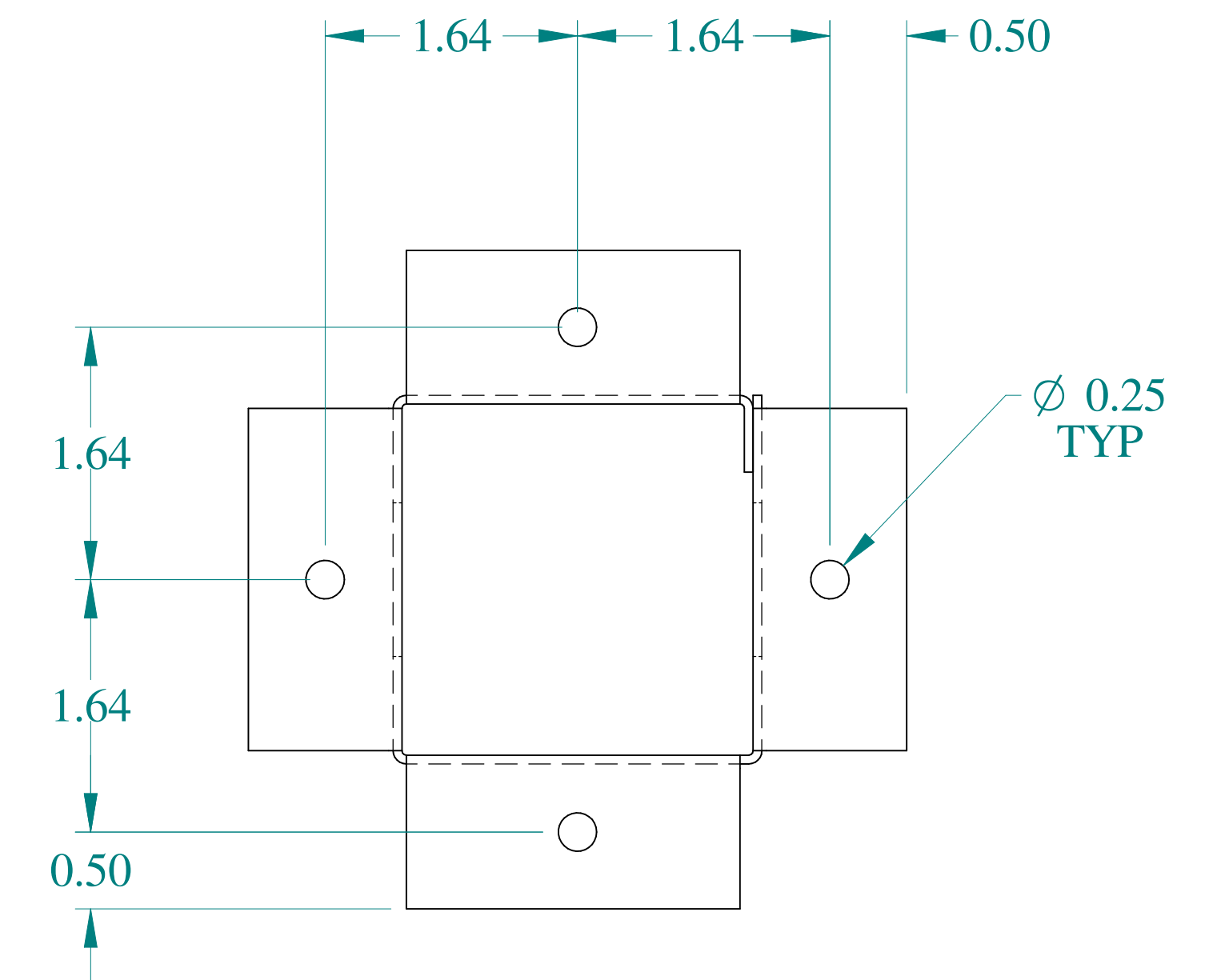
BACK VIEW
