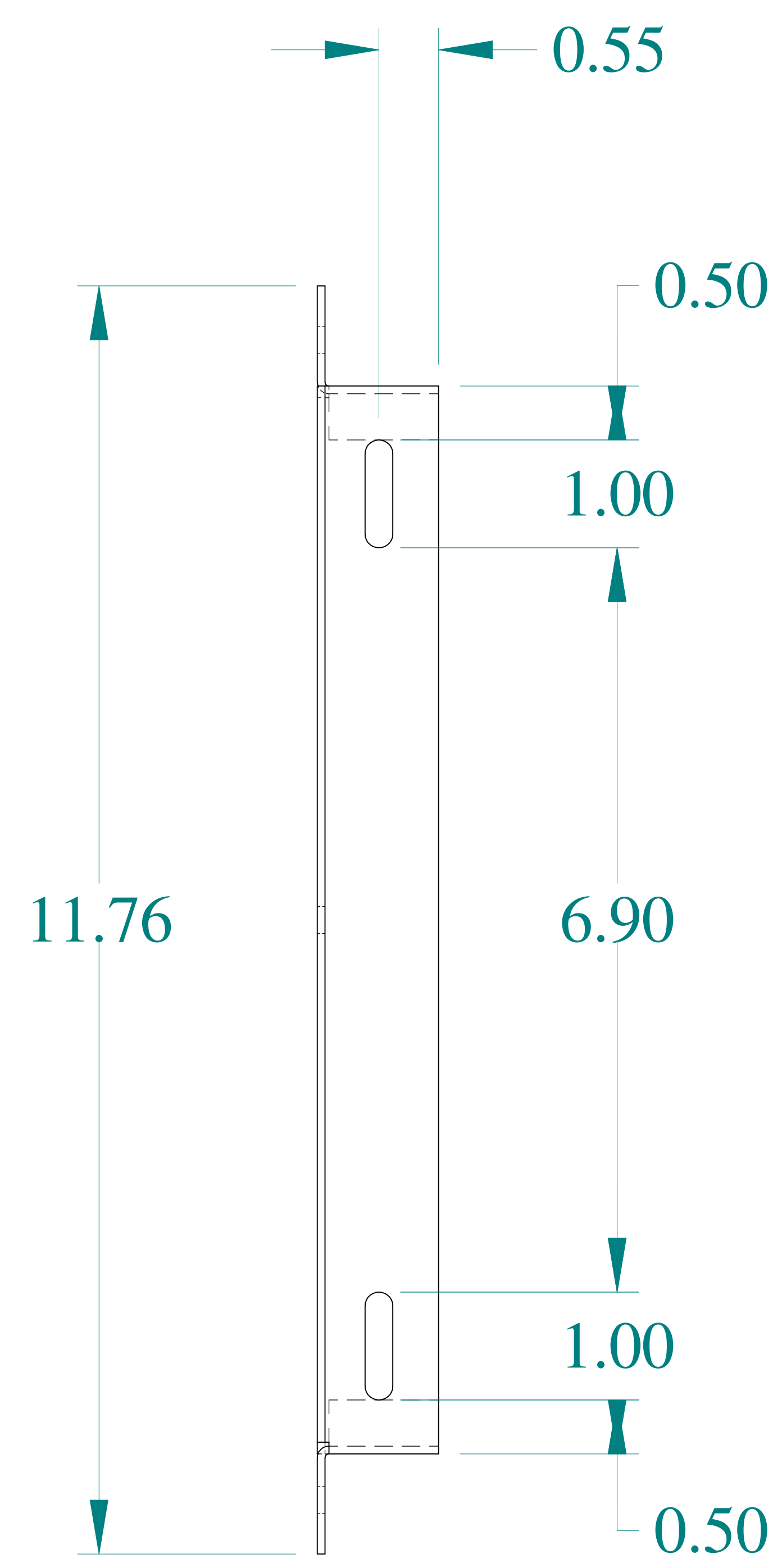
SIDE VIEW
