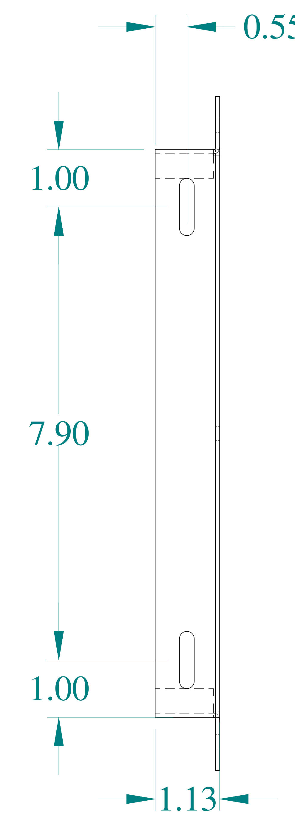
SIDE VIEW
