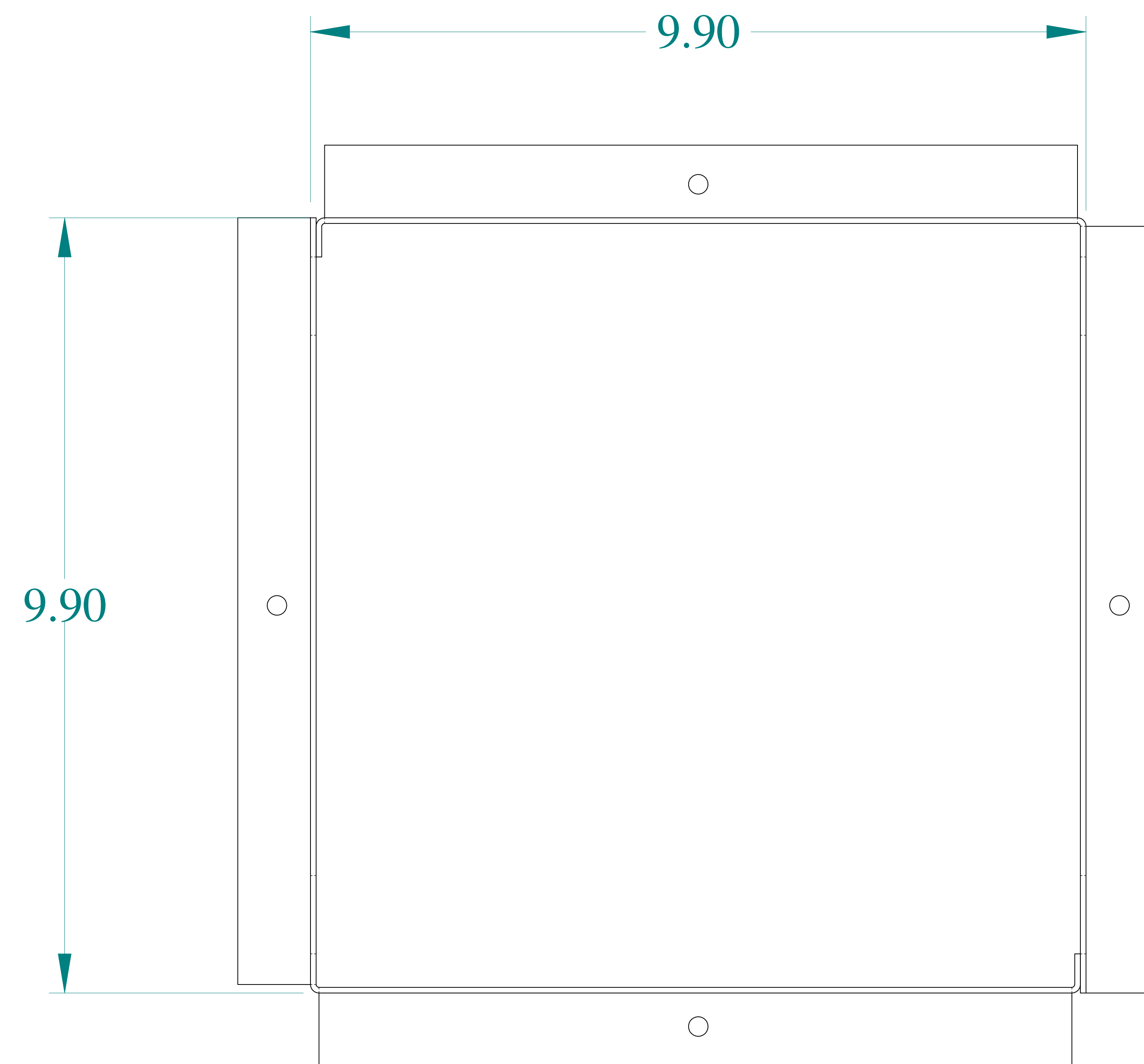
FRONT VIEW
