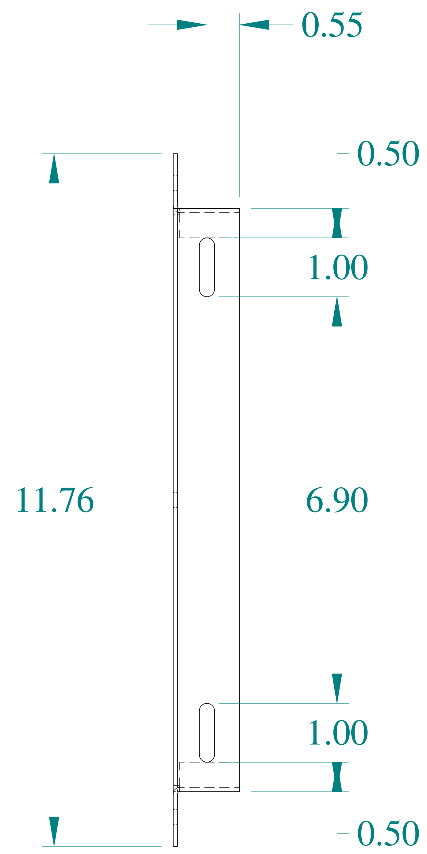
SIDE VIEW
