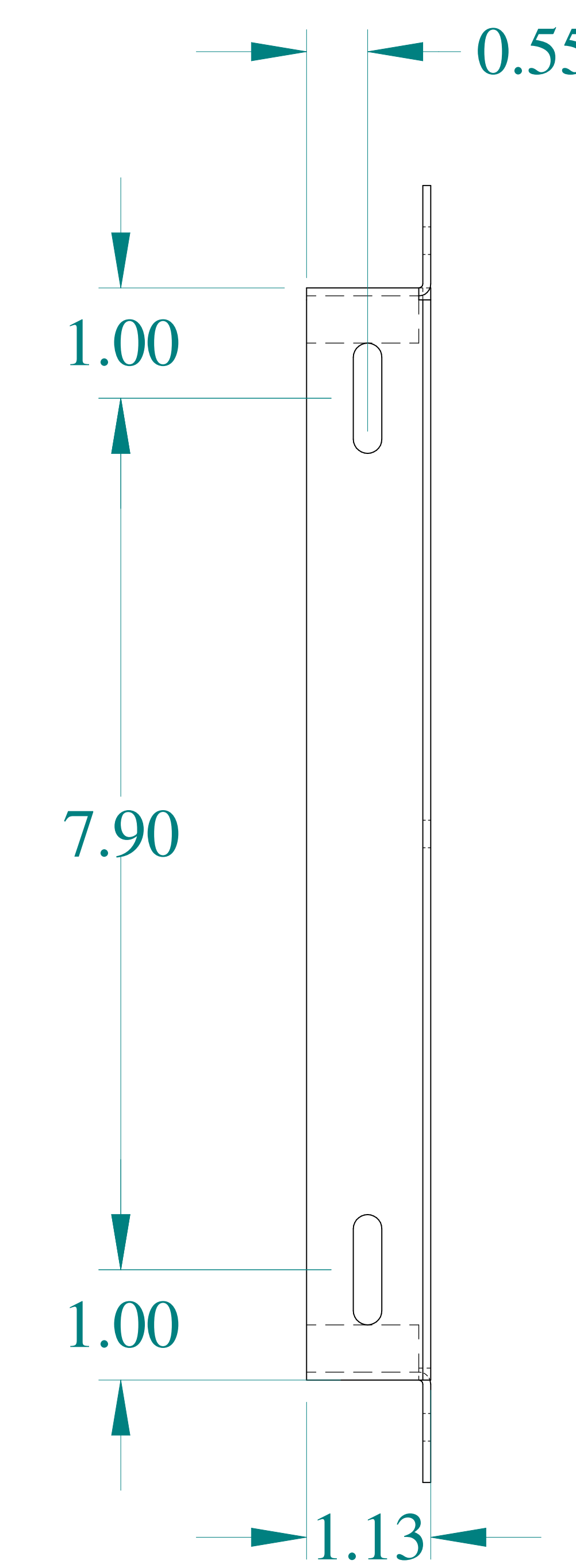
SIDE VIEW
