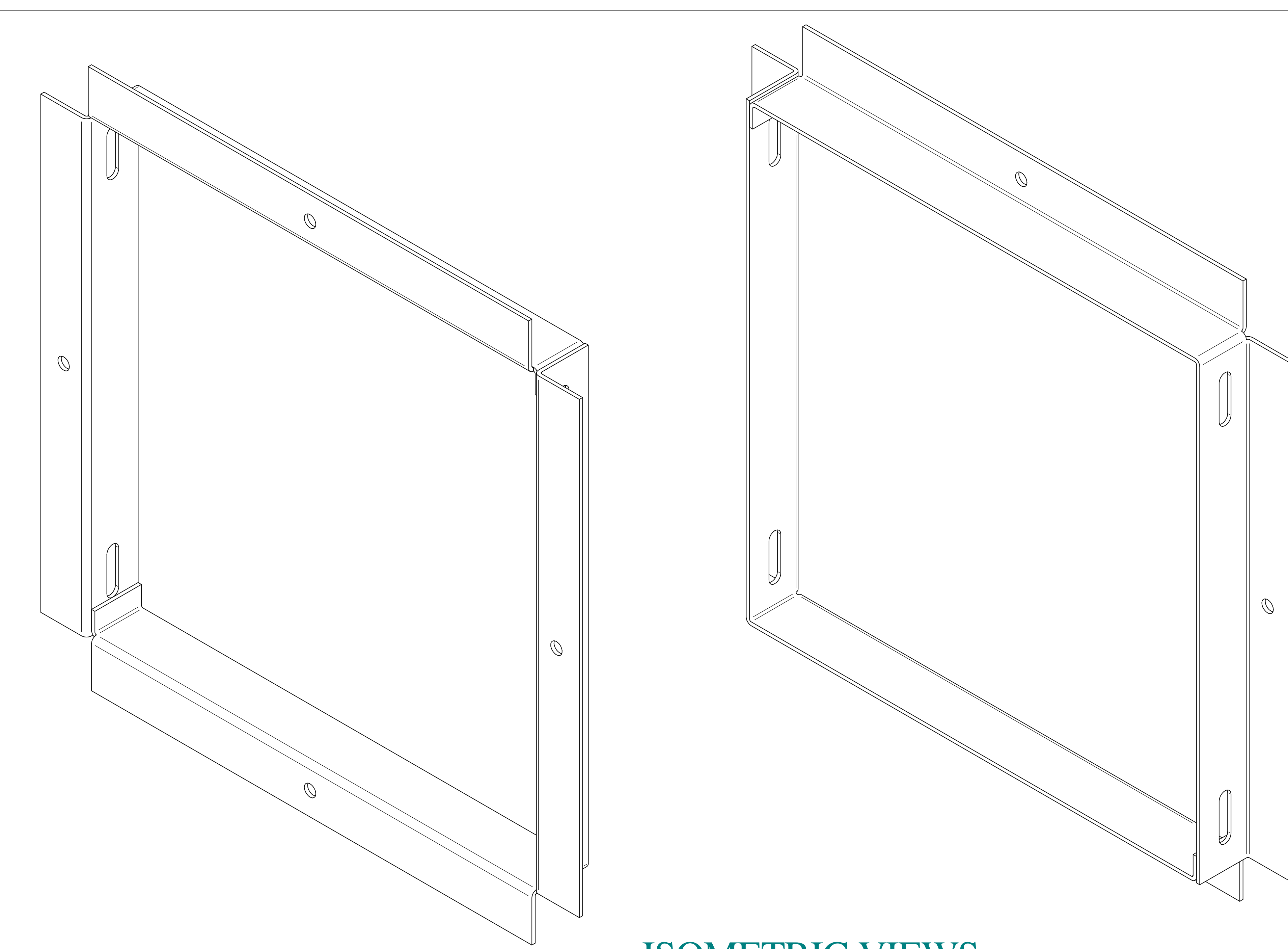
ISOMETRIC VIEWS
