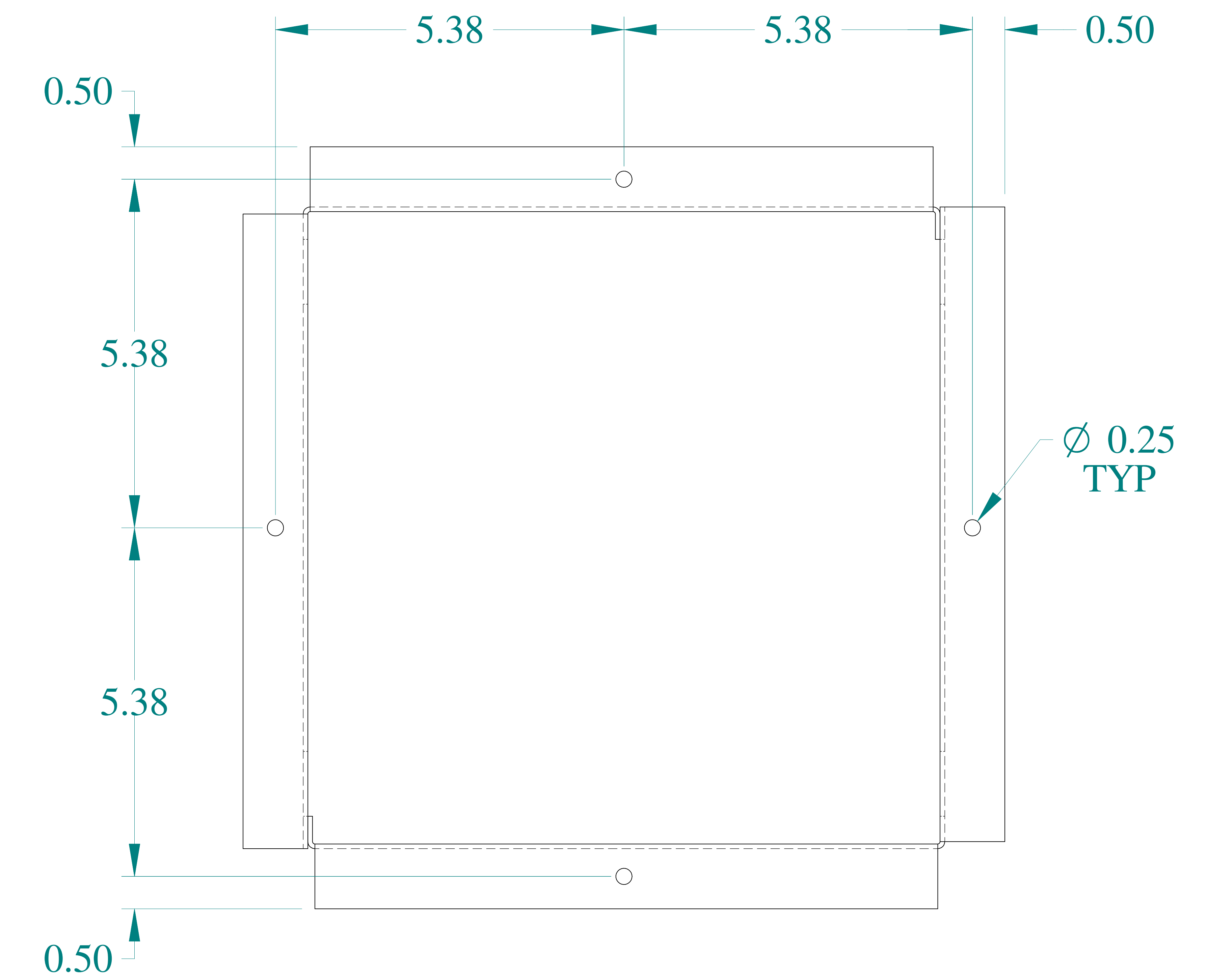
BACK VIEW
