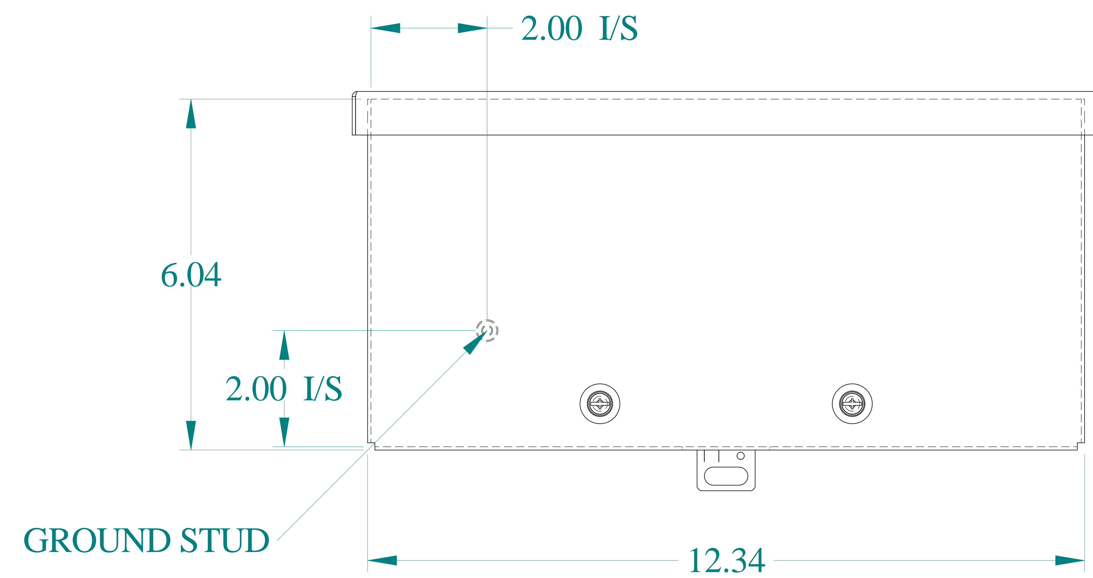
FRONT VIEW
