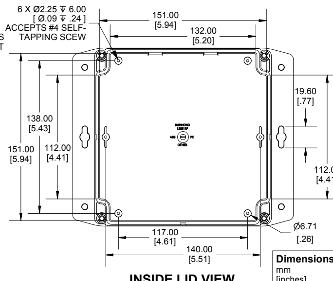
INSIDE LID VIEW
