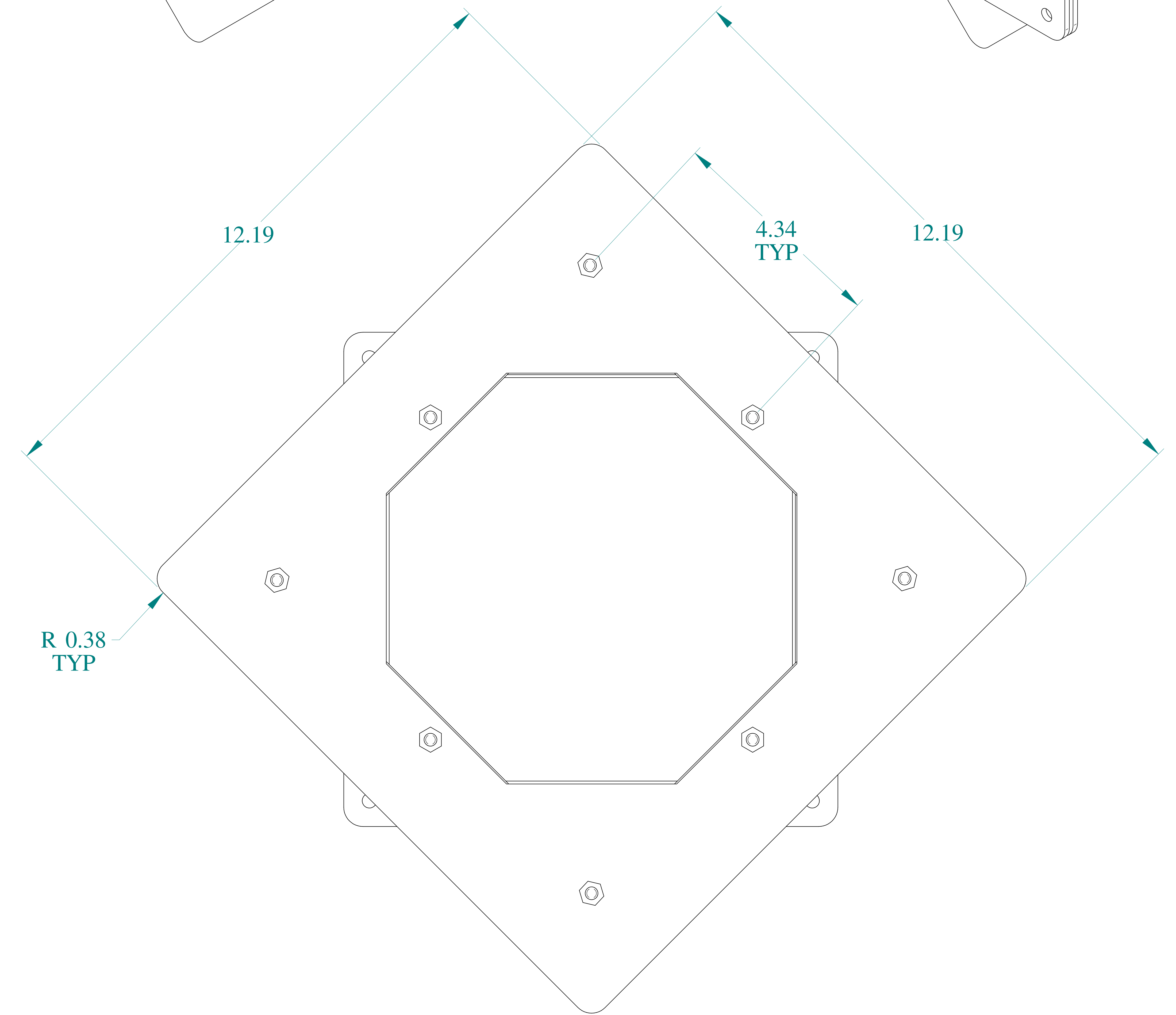
BACK VIEW
