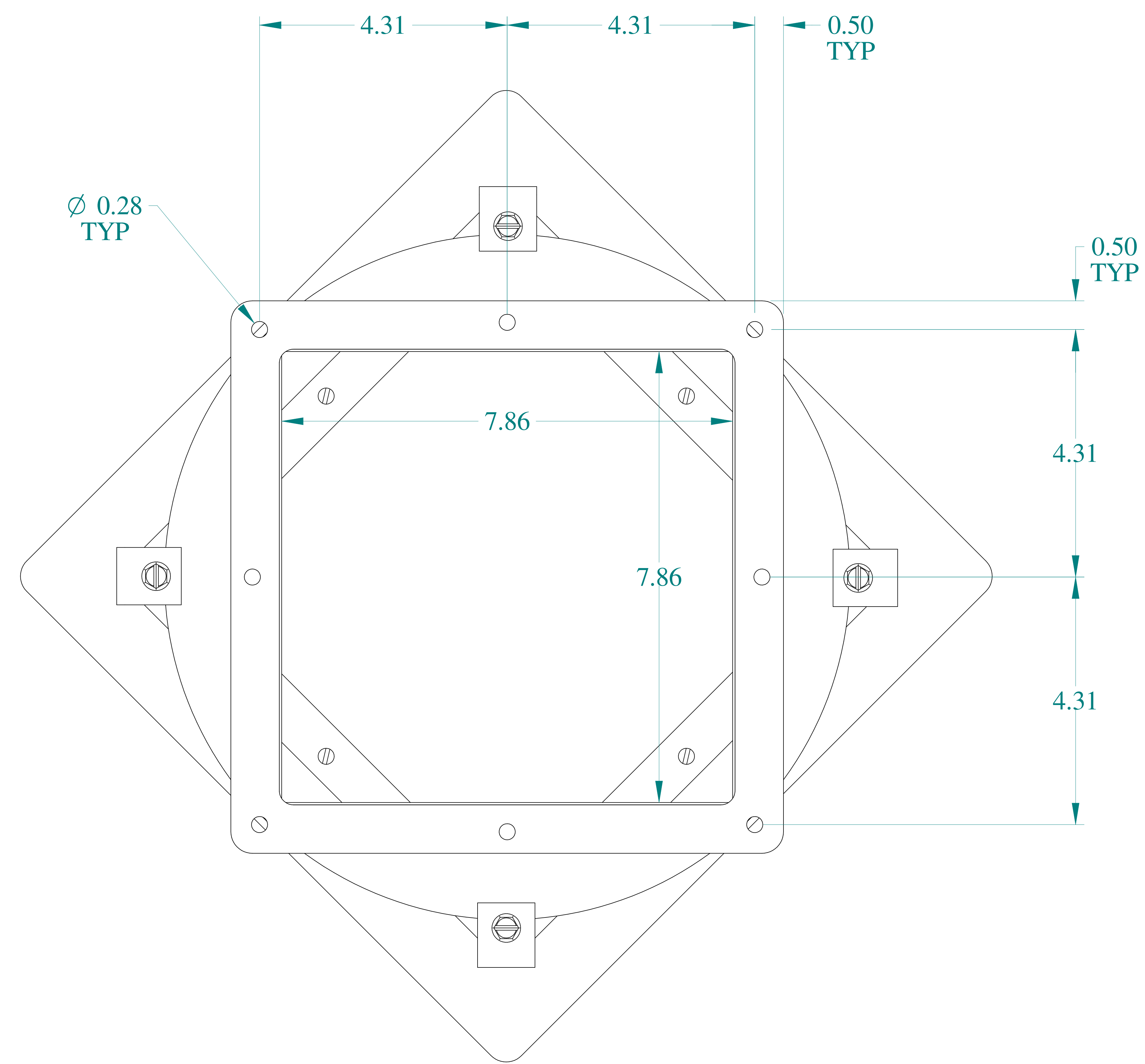
FRONT VIEW
