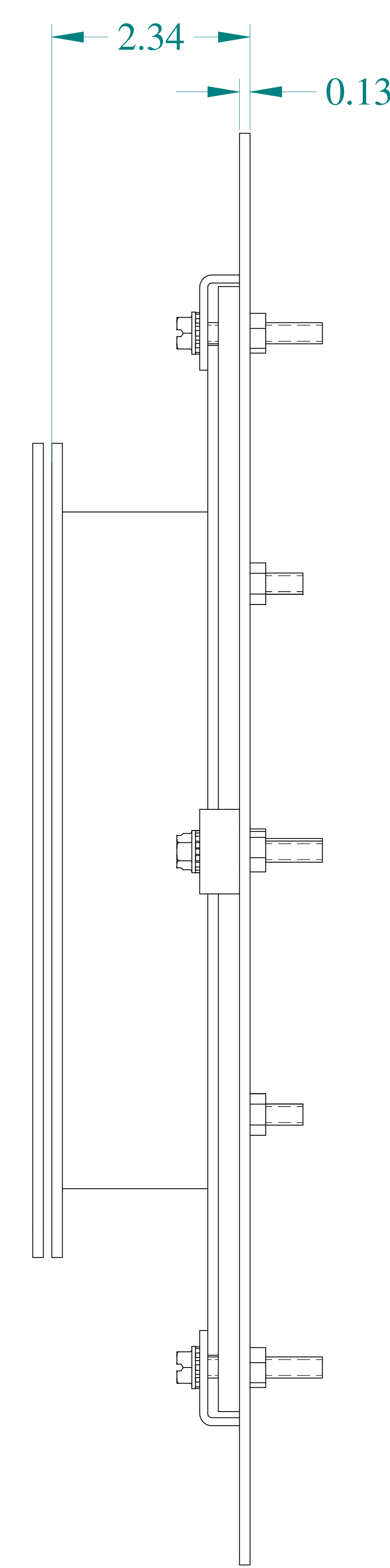
SIDE VIEW
