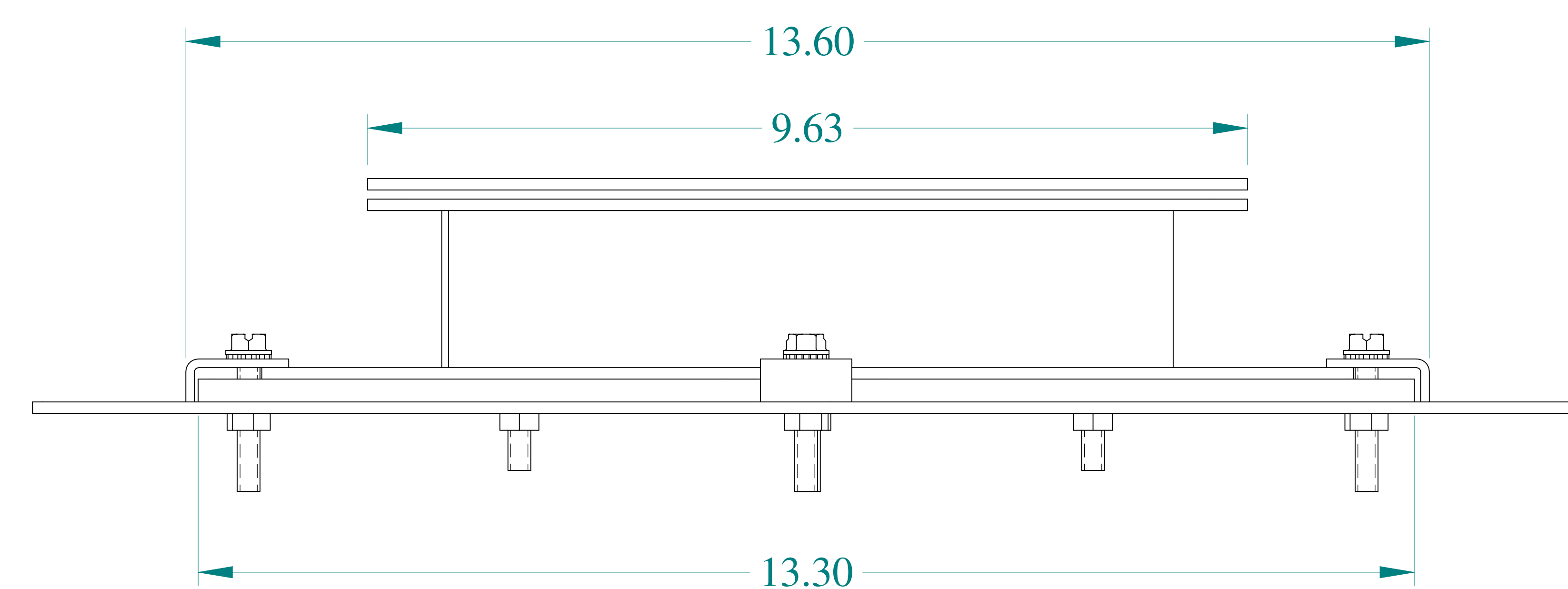
BOTTOM VIEW
