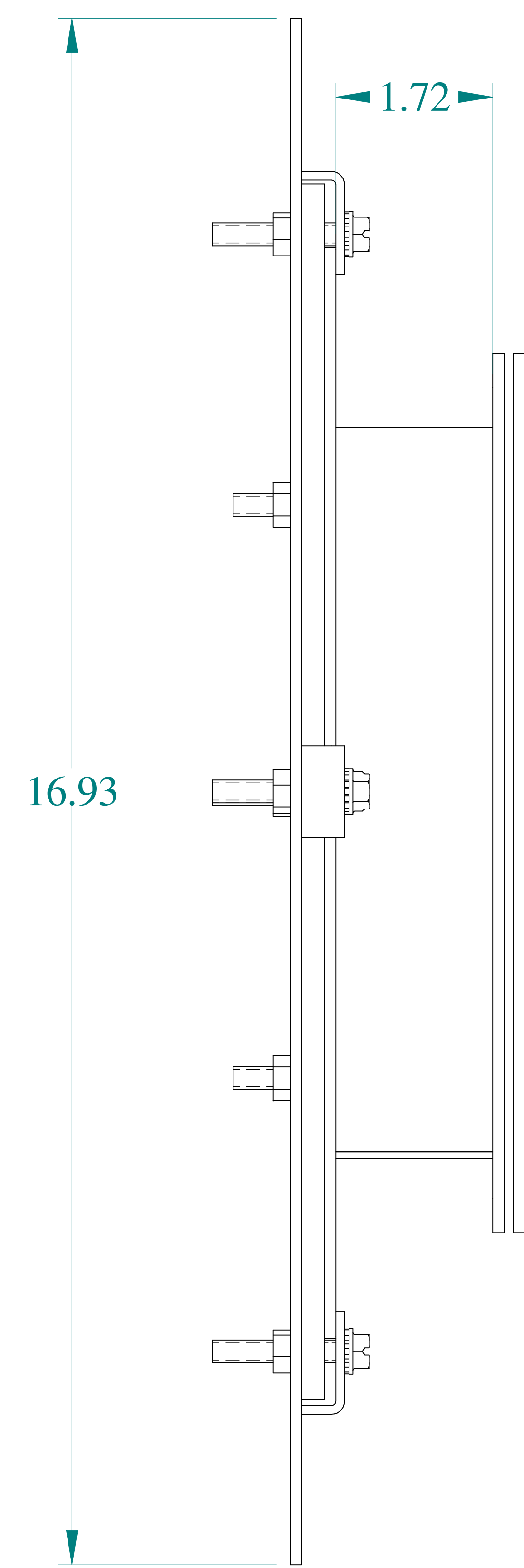
SIDE VIEW
