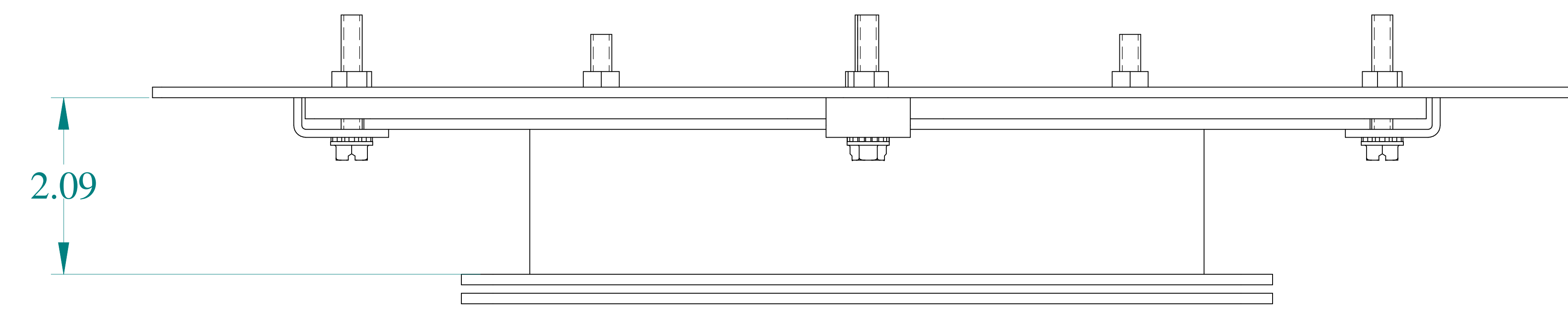
TOP VIEW
