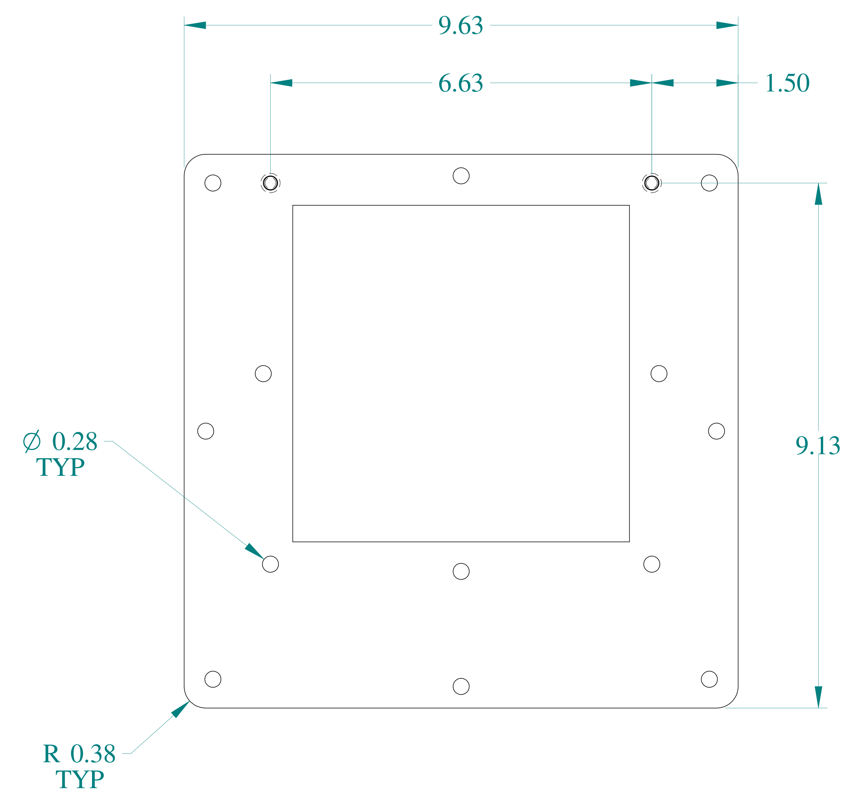
FRONT VIEW
