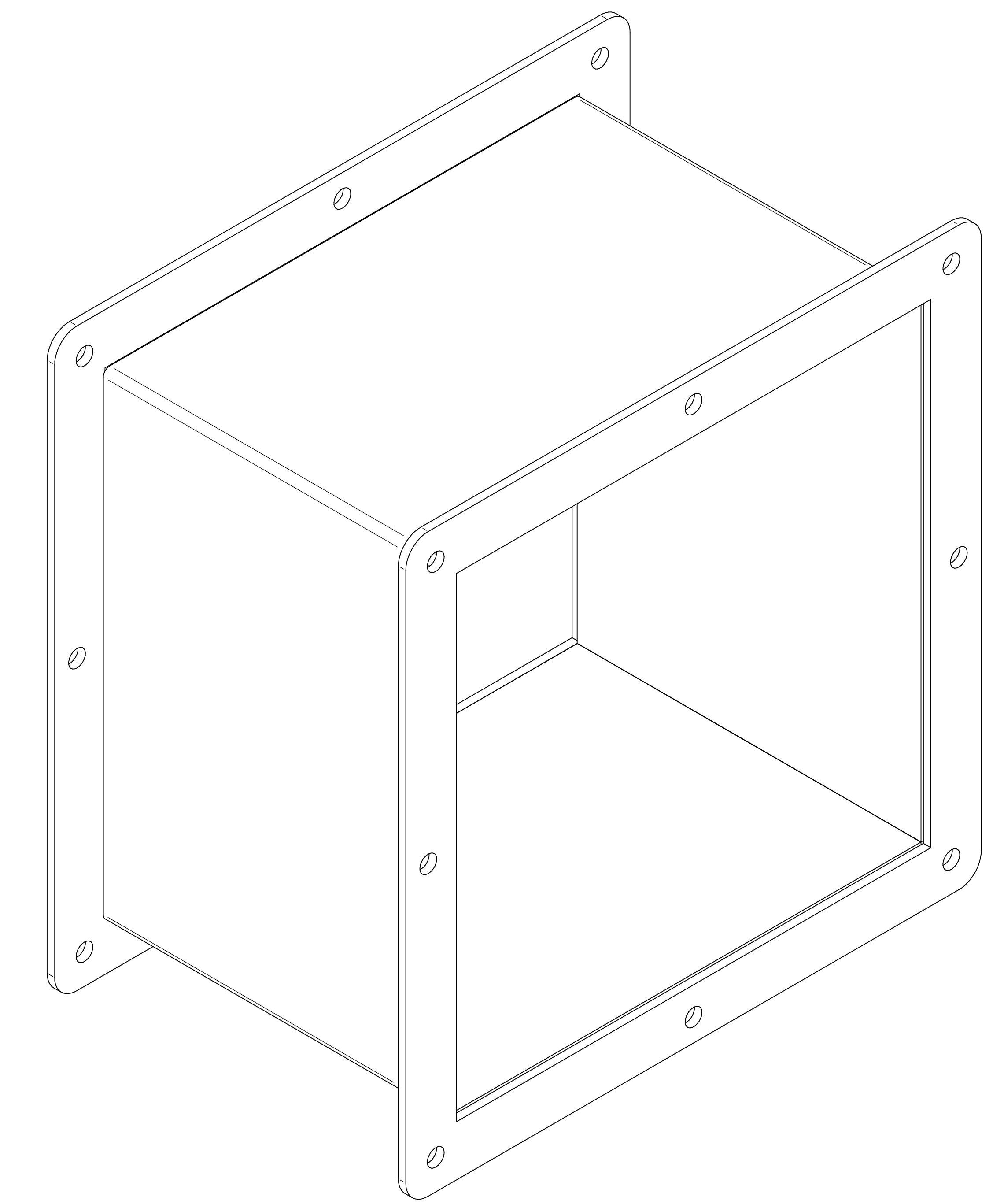
ISOMETRIC VIEWS
