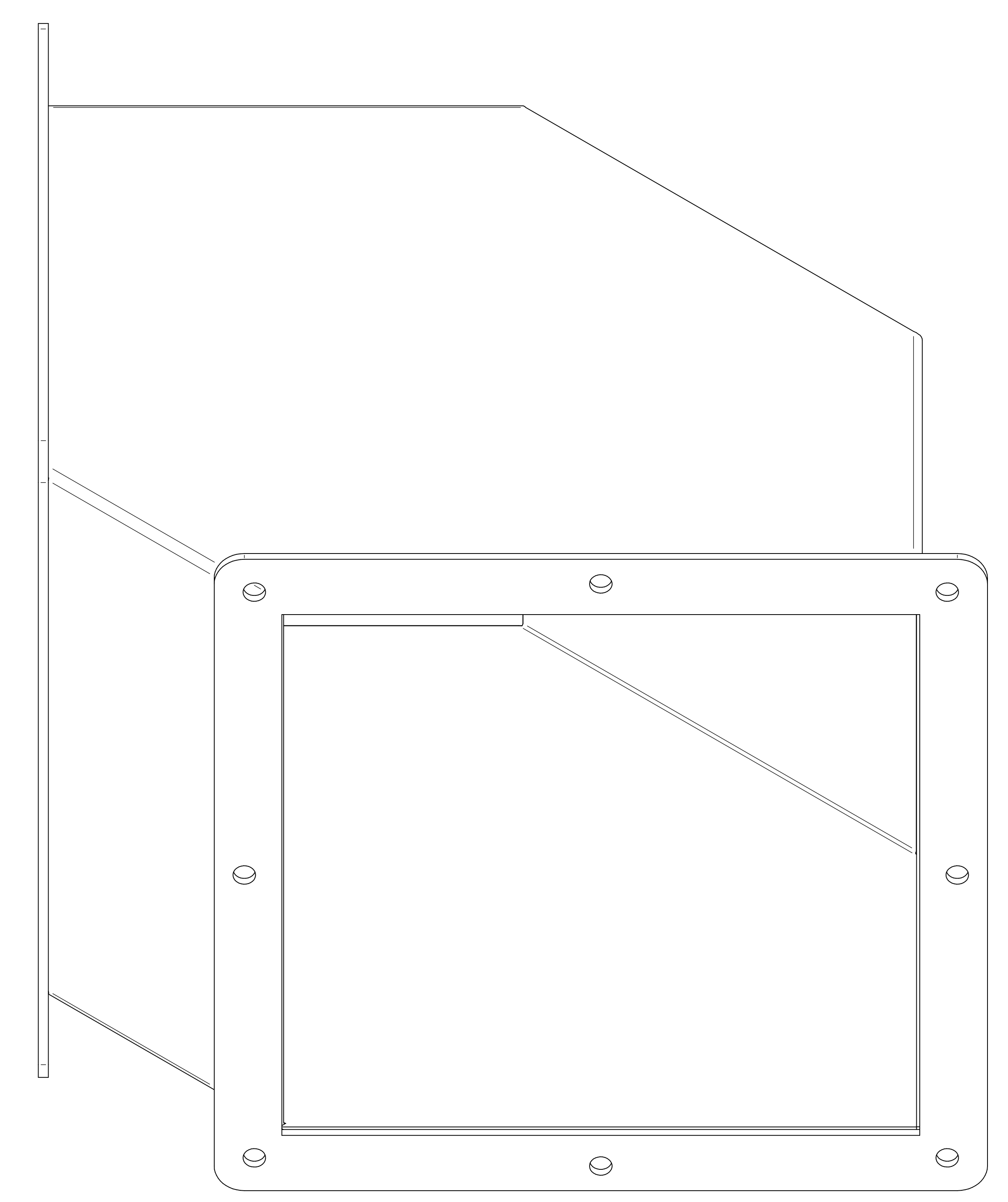
ISOMETRIC VIEWS
