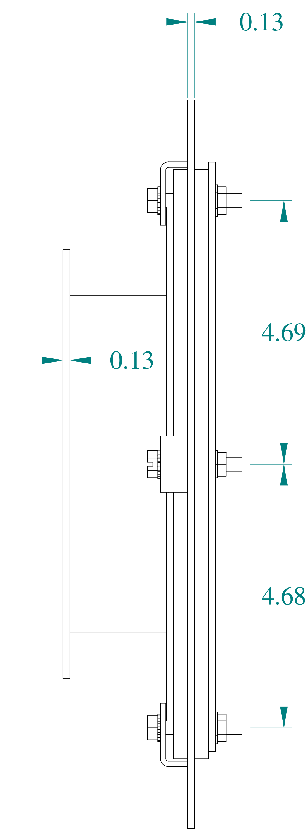
SIDE VIEW
