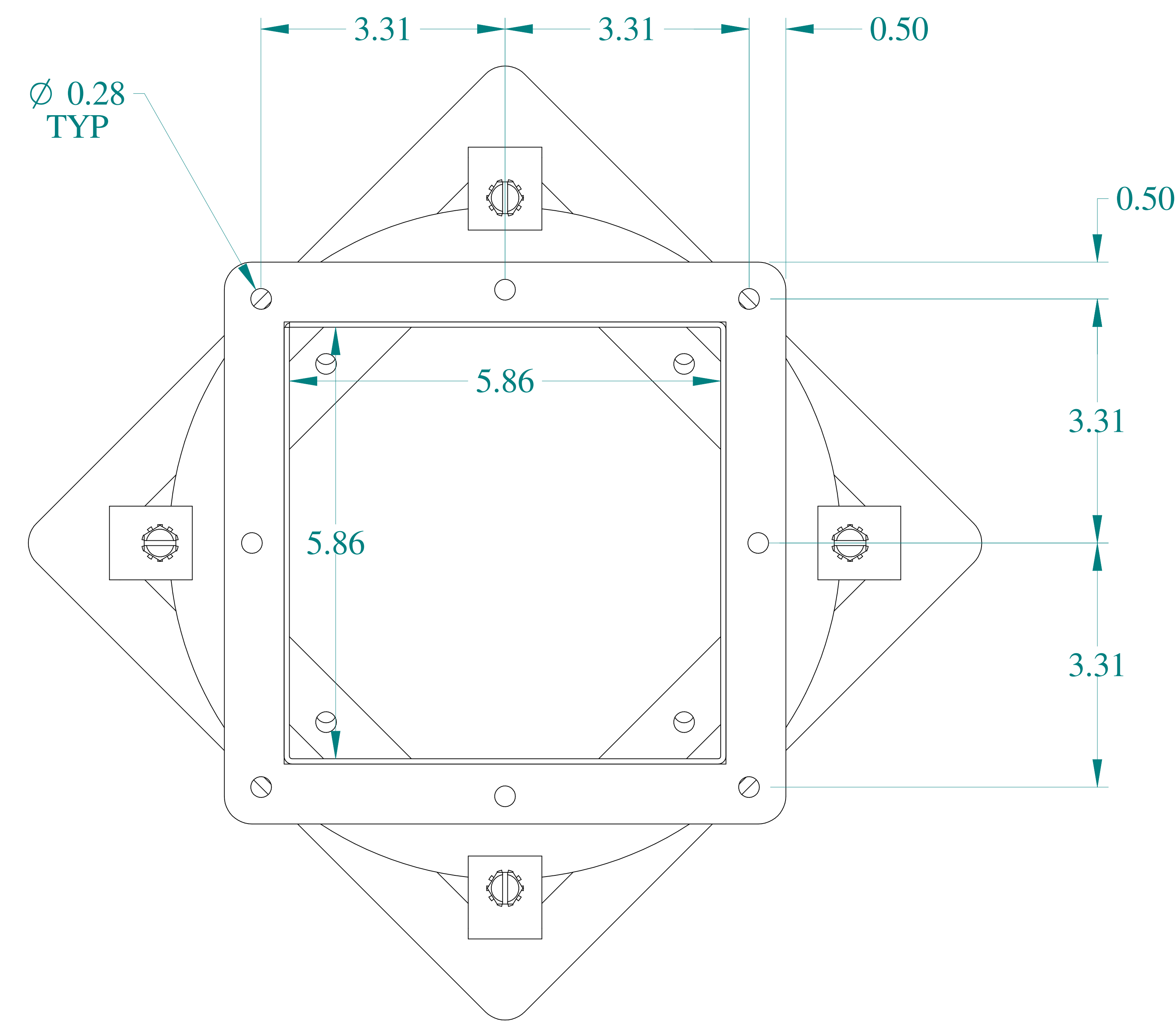
FRONT VIEW
