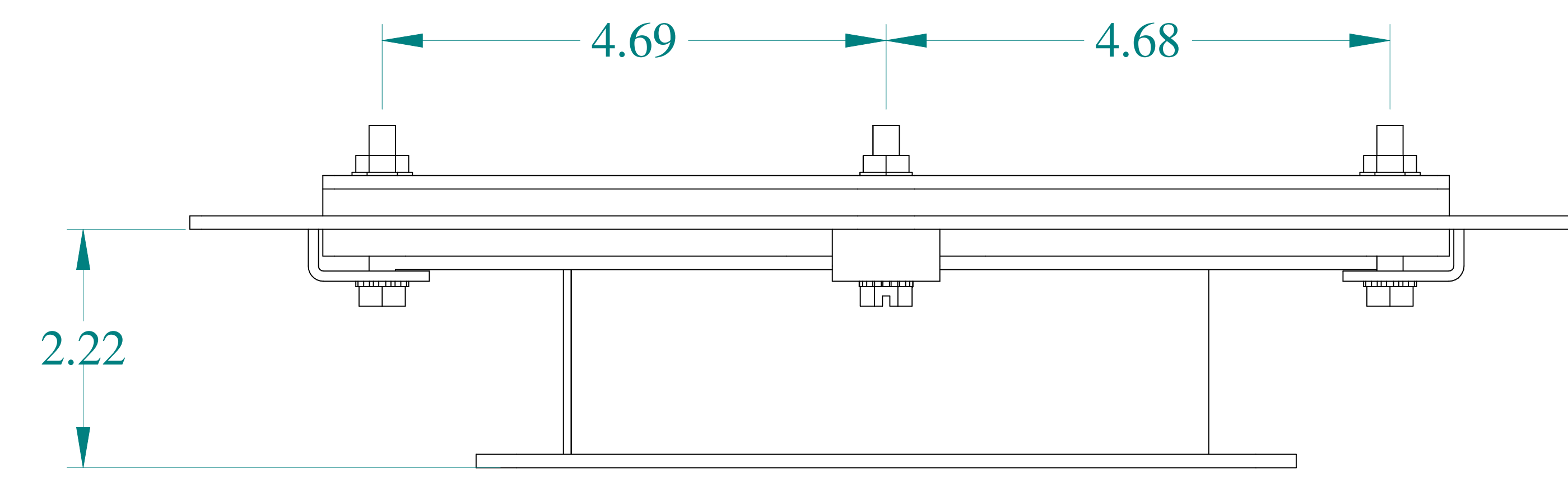
TOP VIEW
