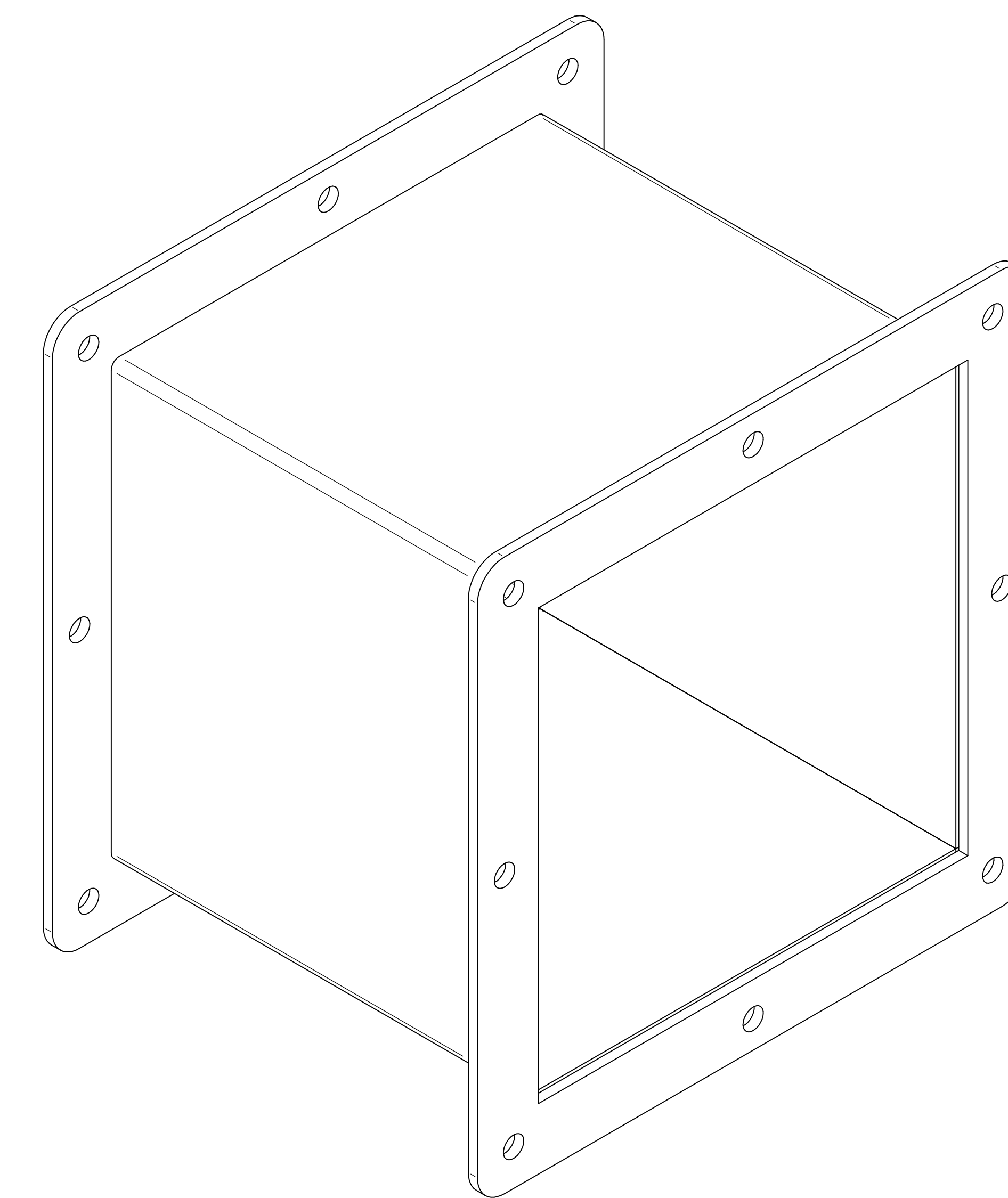
ISOMETRIC VIEWS
