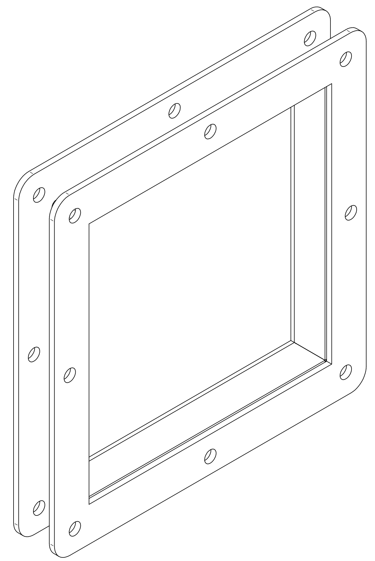
ISOMETRIC VIEWS
