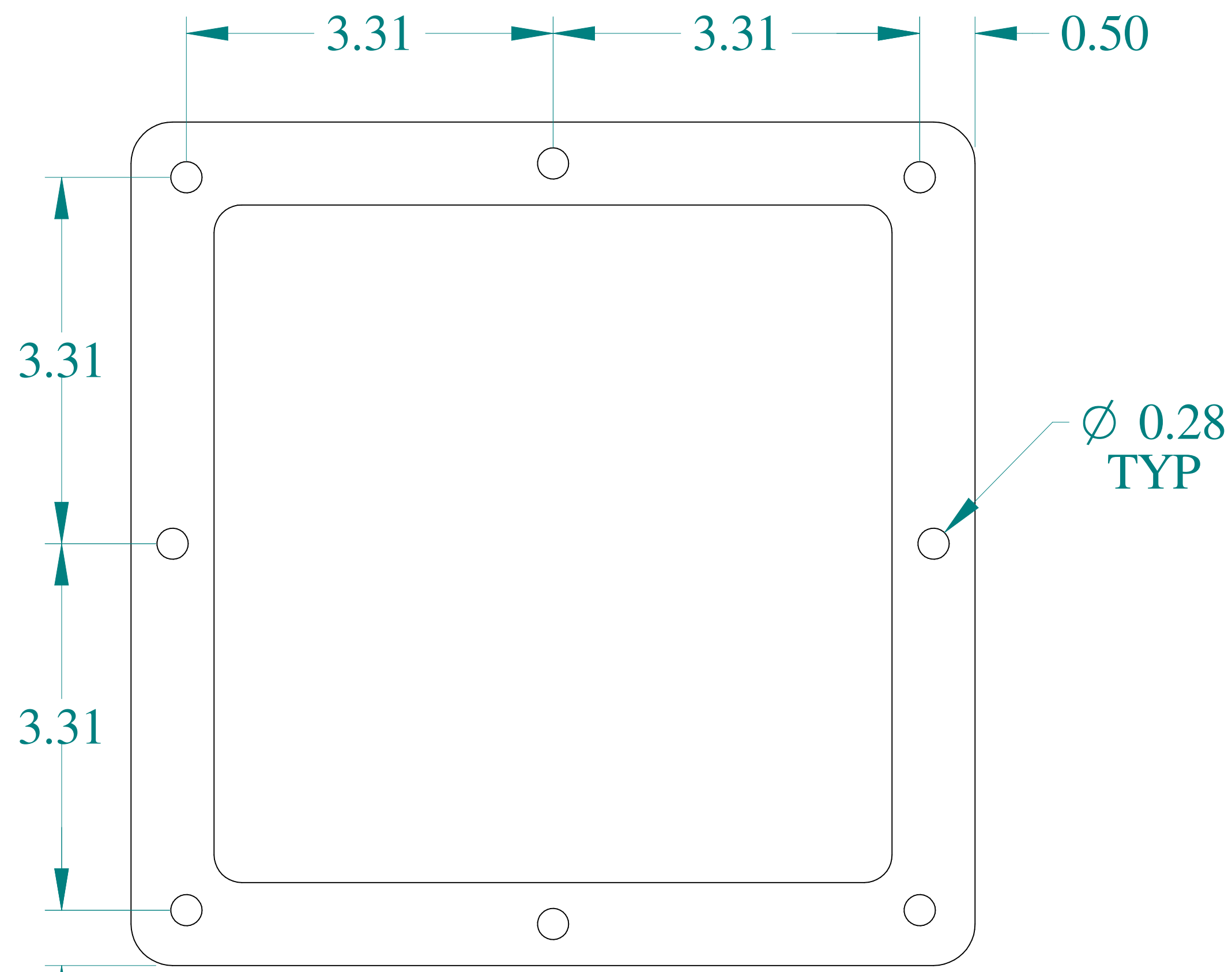
FRONT VIEW
