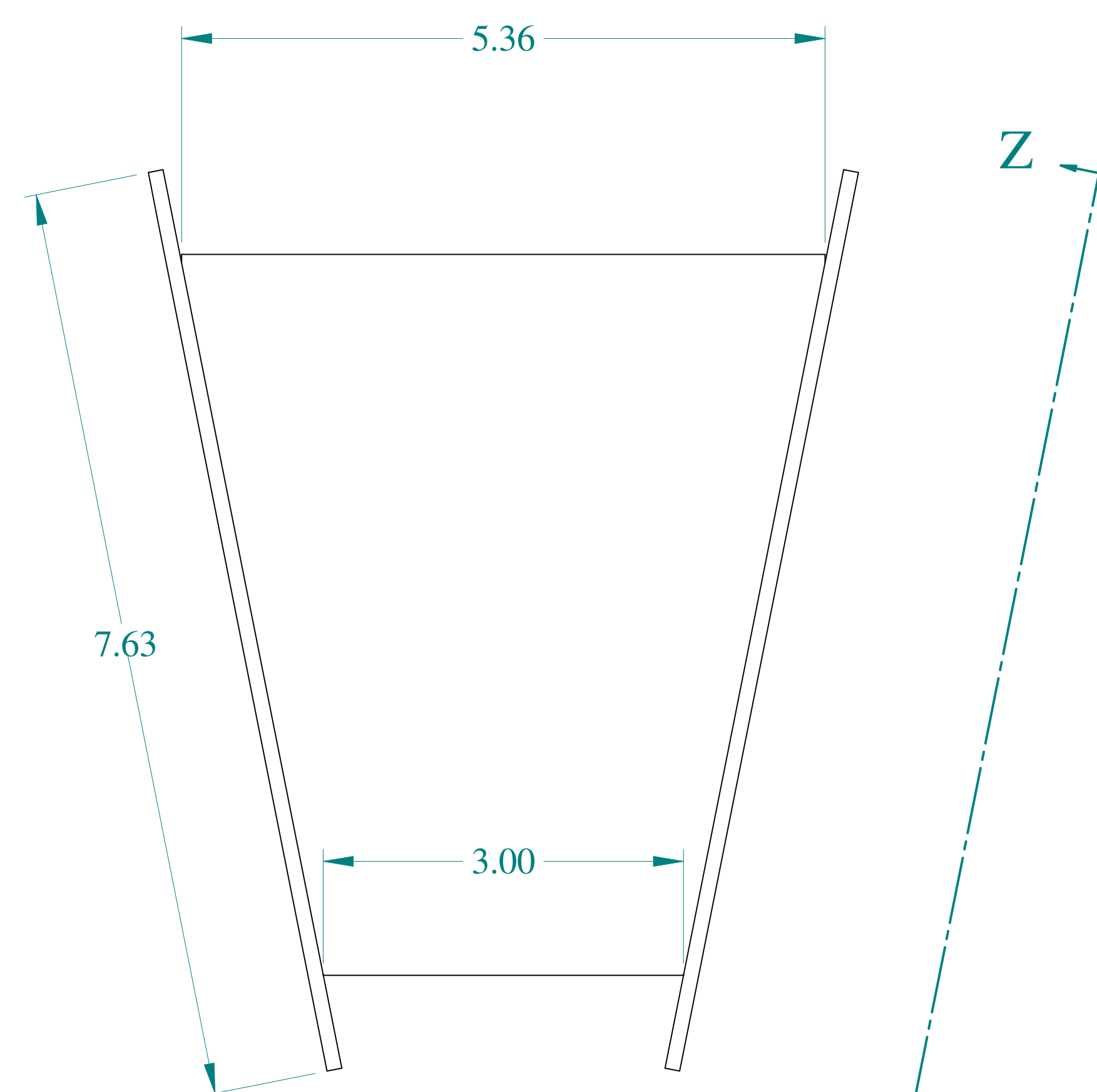
FRONT VIEW
