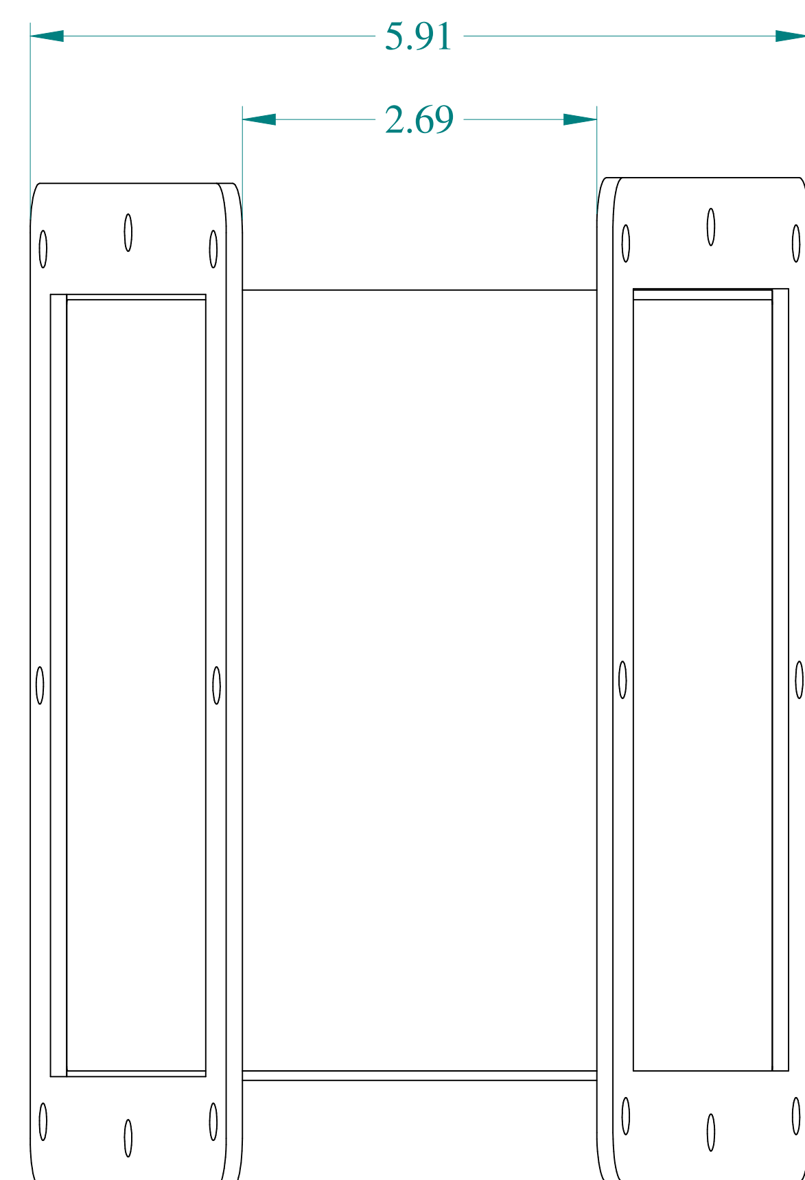
BOTTOM VIEW
