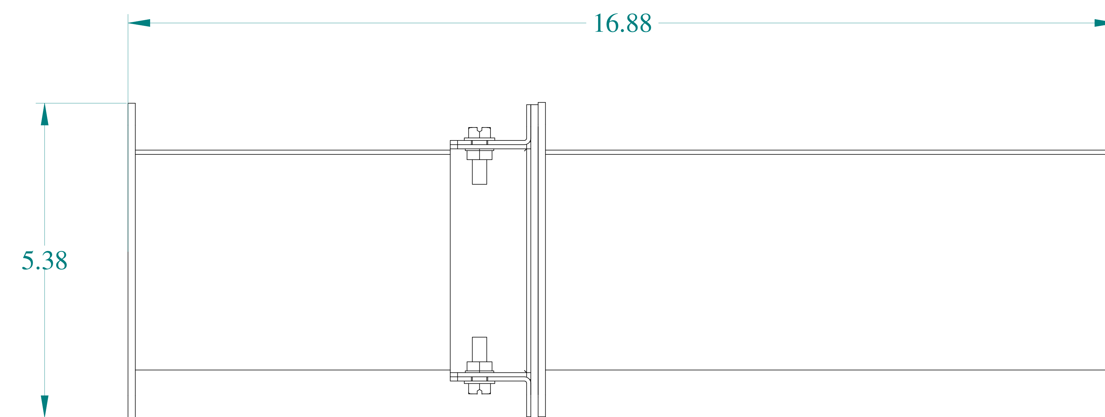
BOTTOM VIEW
