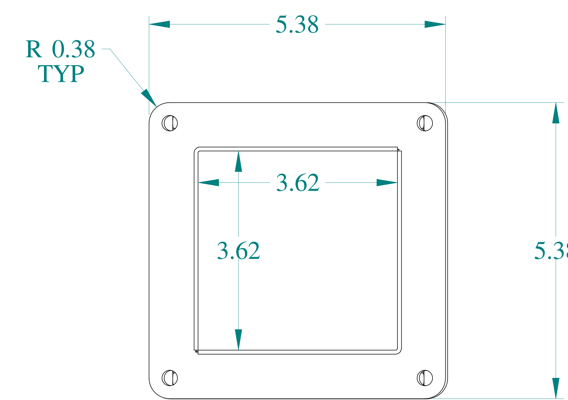
SIDE VIEW
