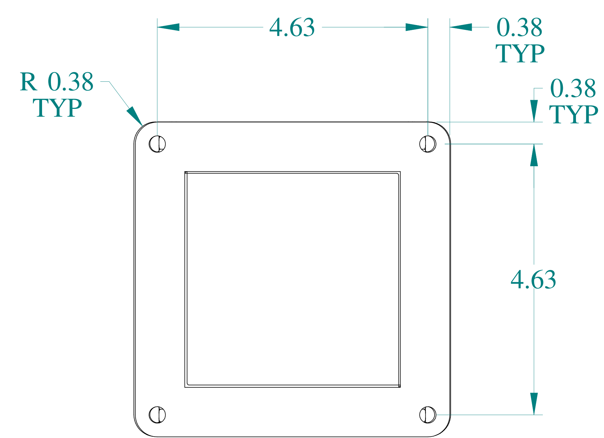
SIDE VIEW
