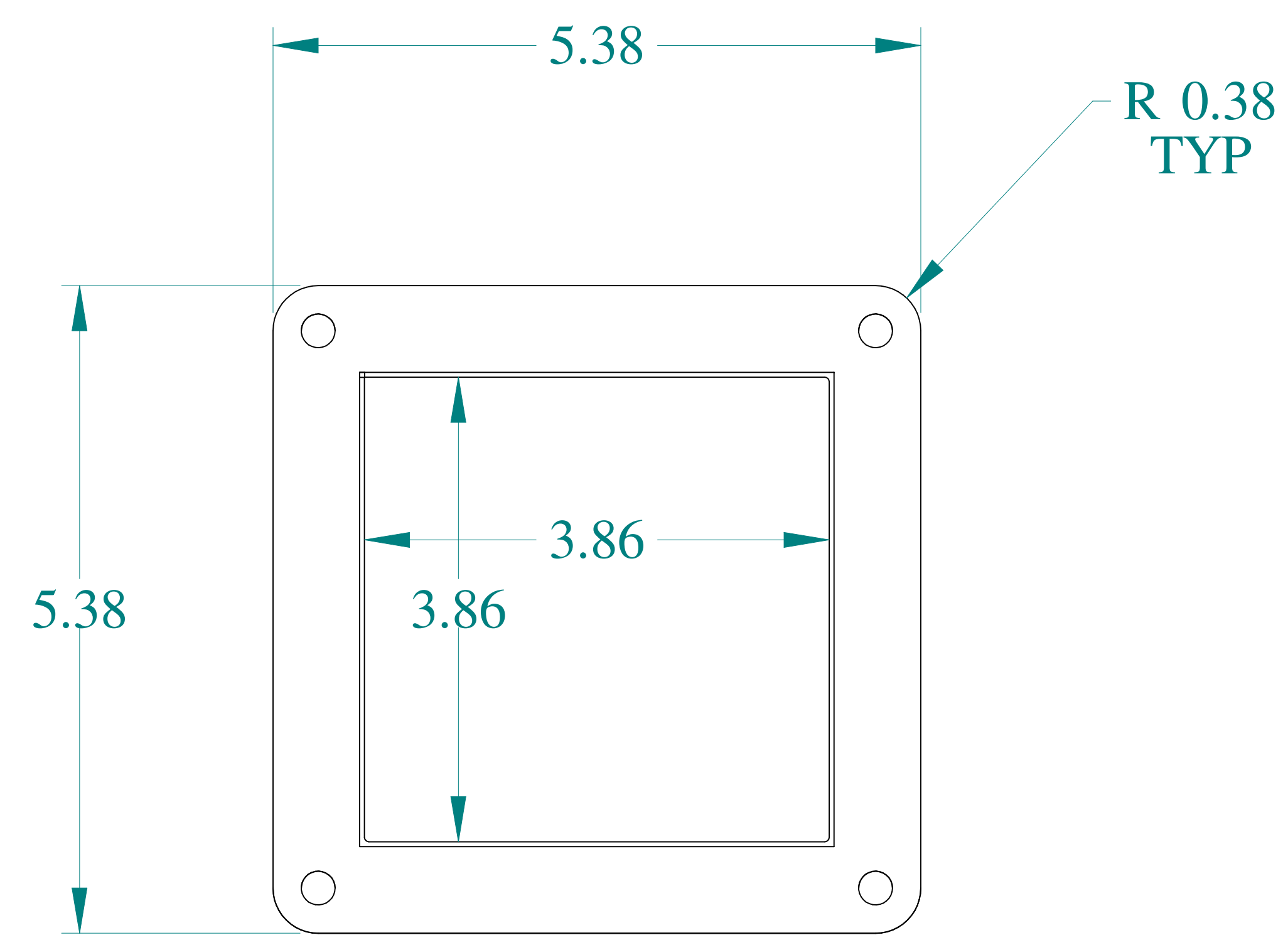
SIDE VIEW
