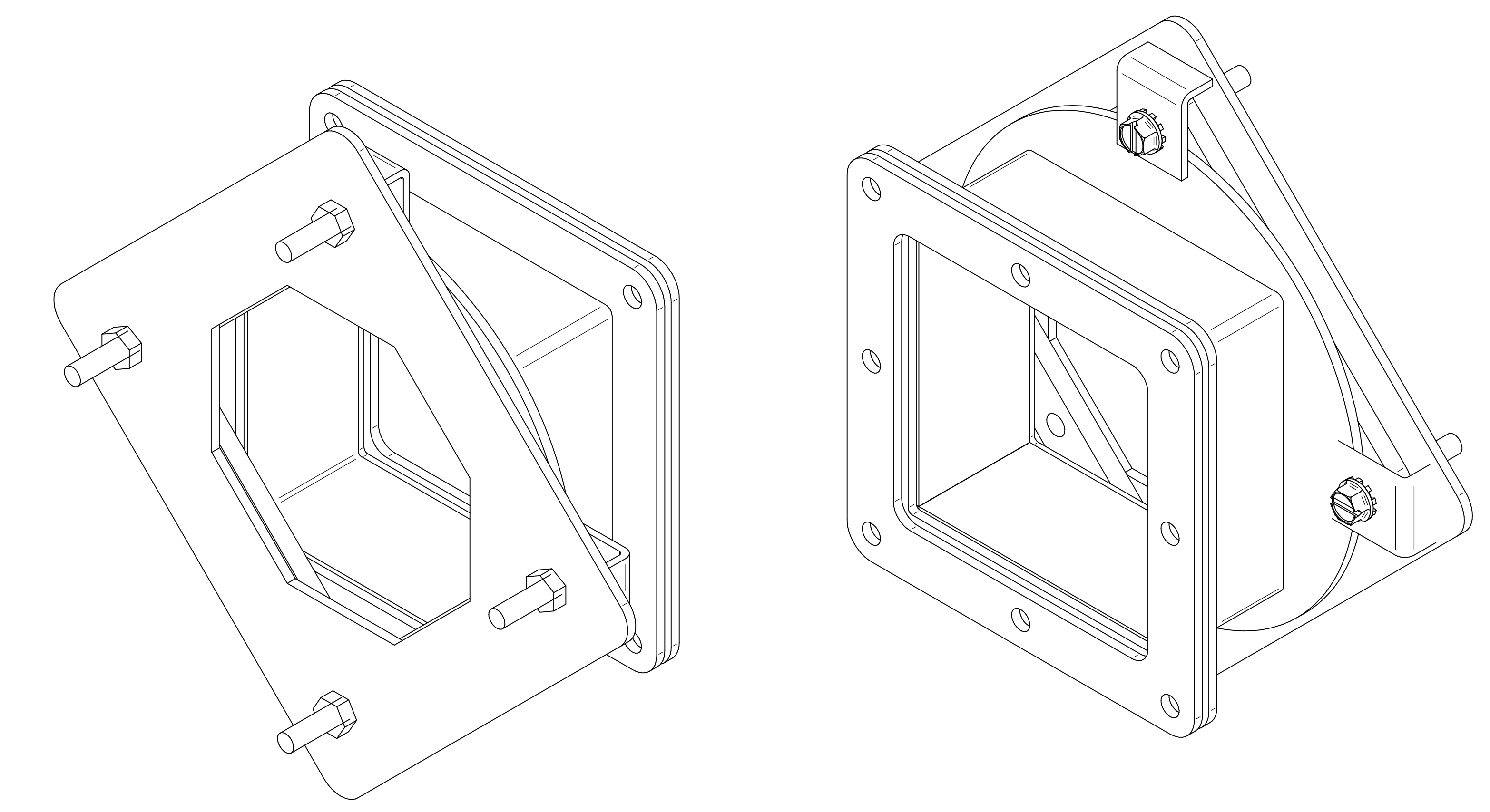
ISOMETRIC VIEWS
