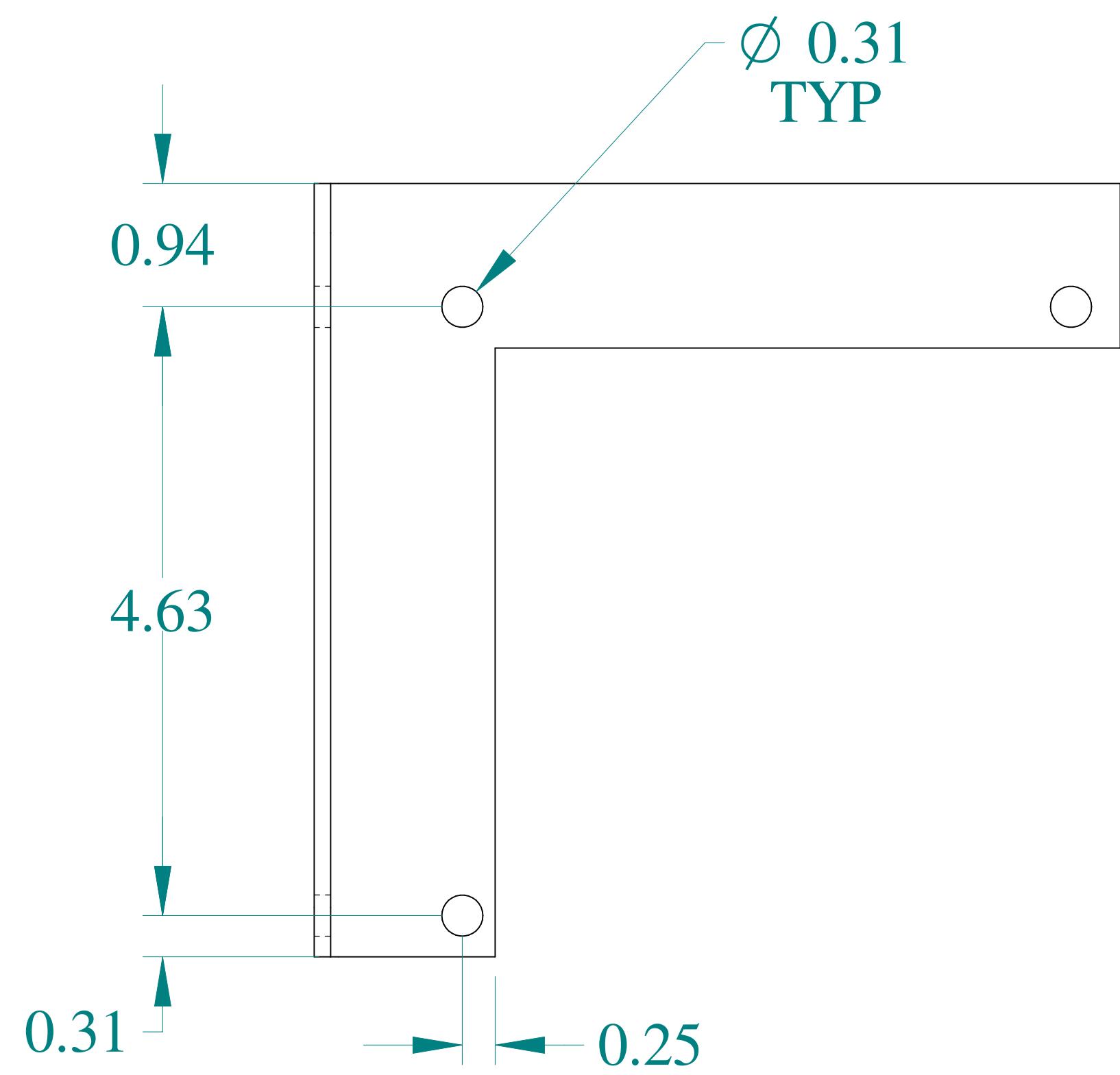
FRONT VIEW
