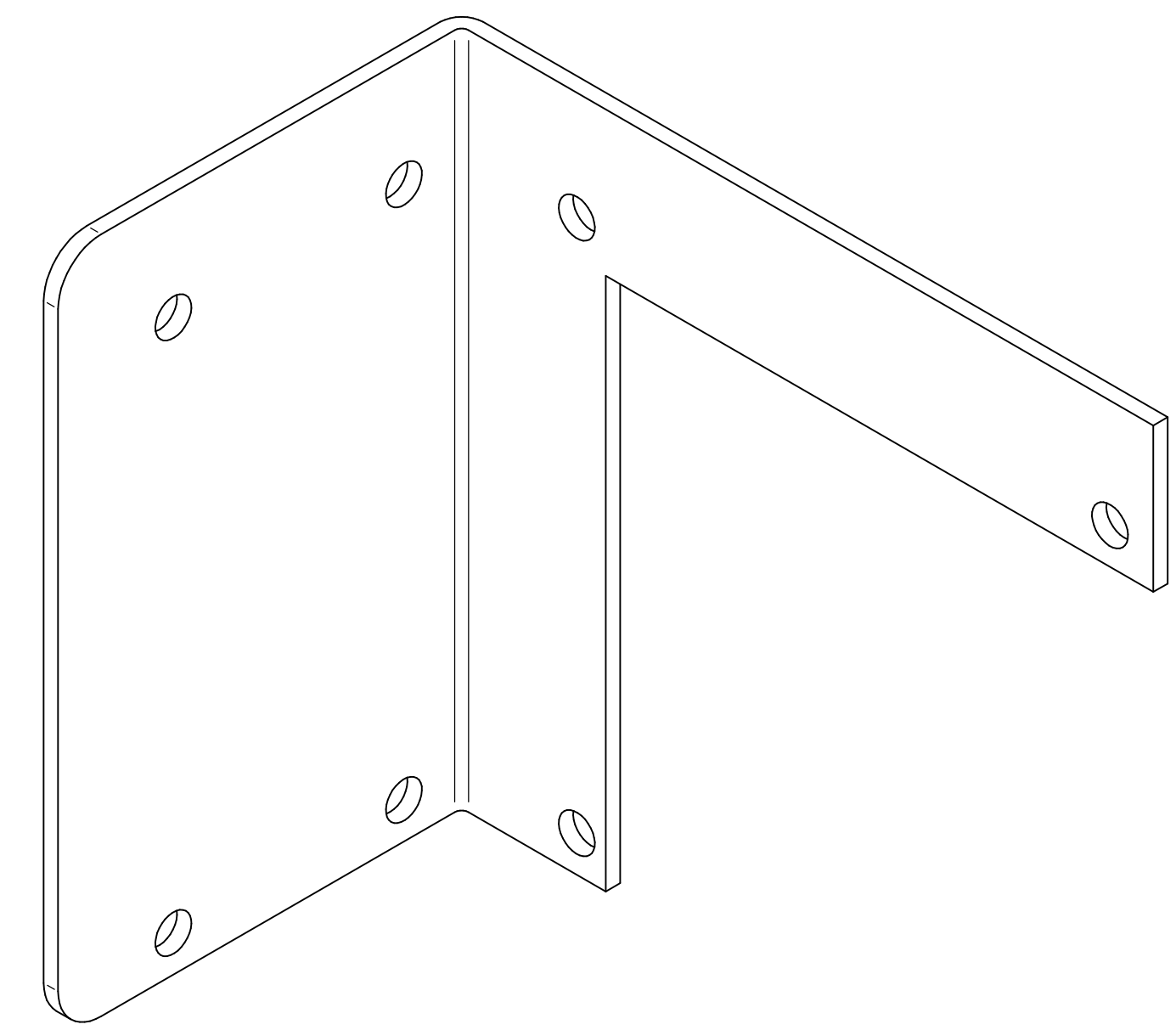
ISOMETRIC VIEWS
