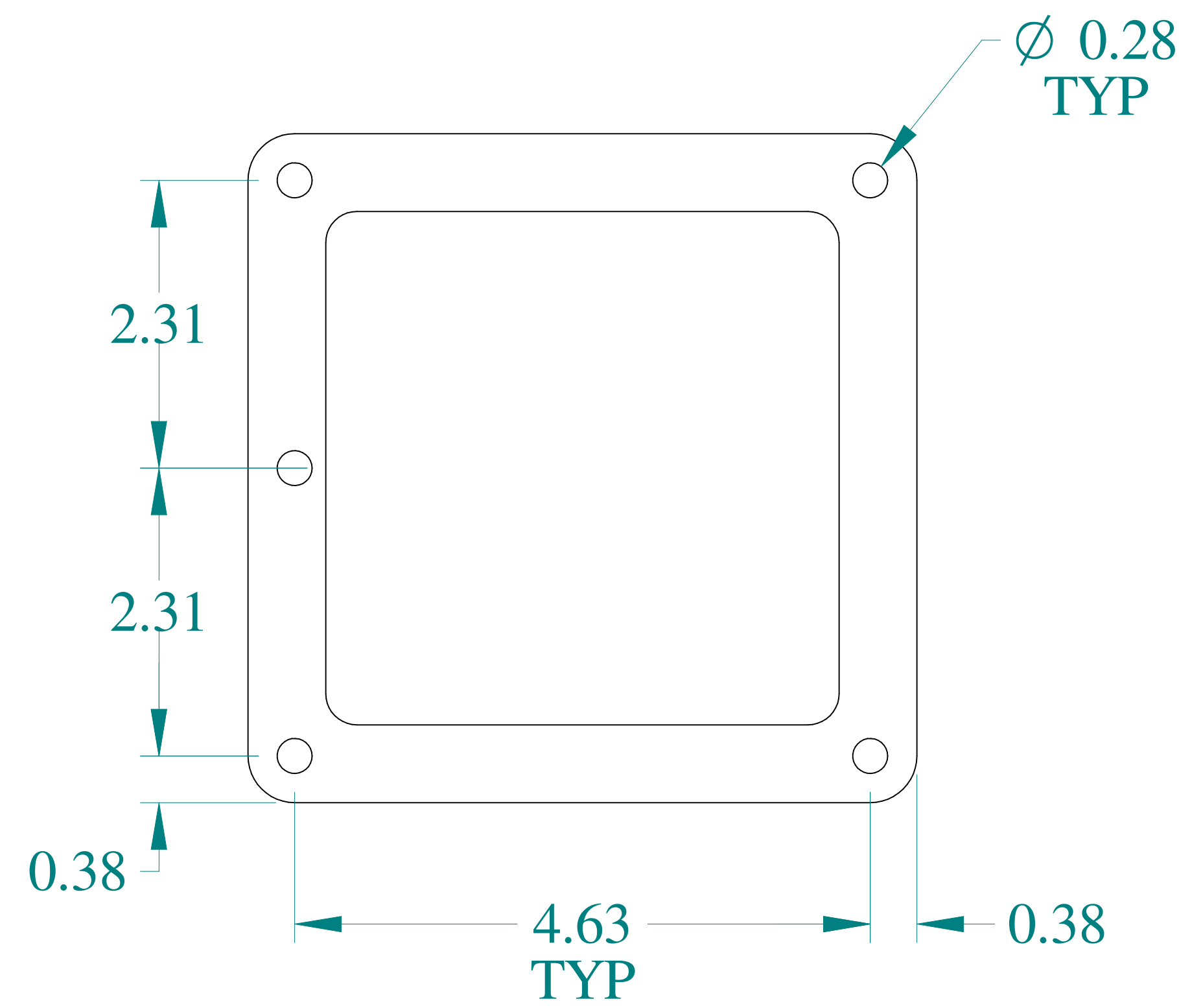
FRONT VIEW
