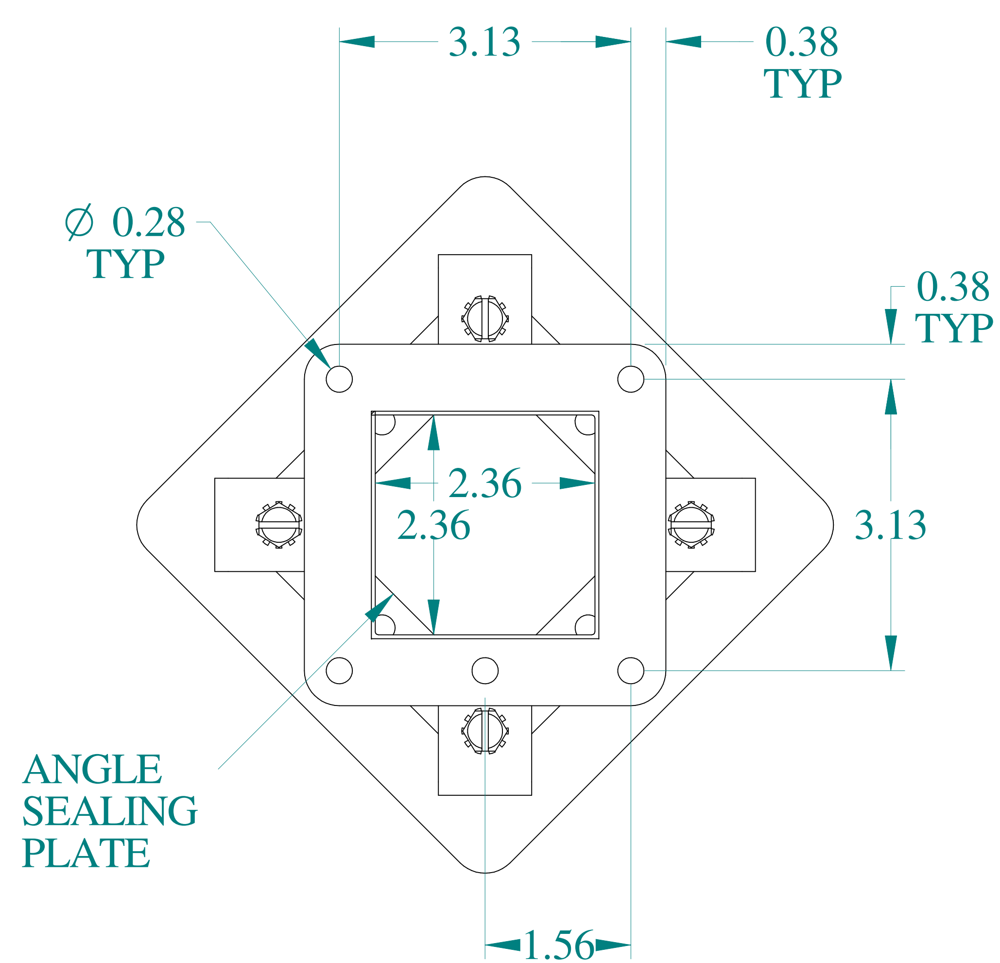
FRONT VIEW
