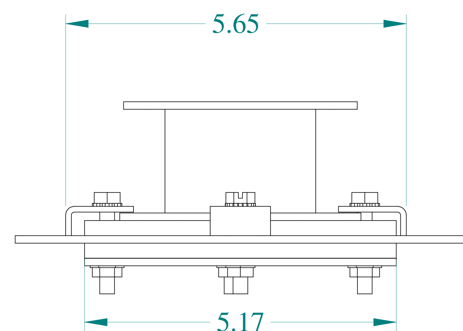
BOTTOM VIEW
