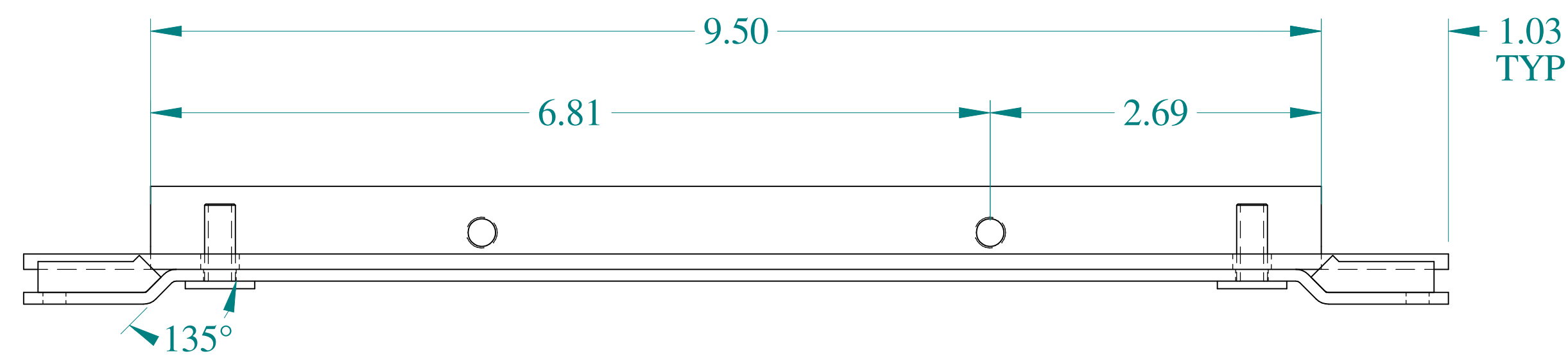
FRONT VIEW
