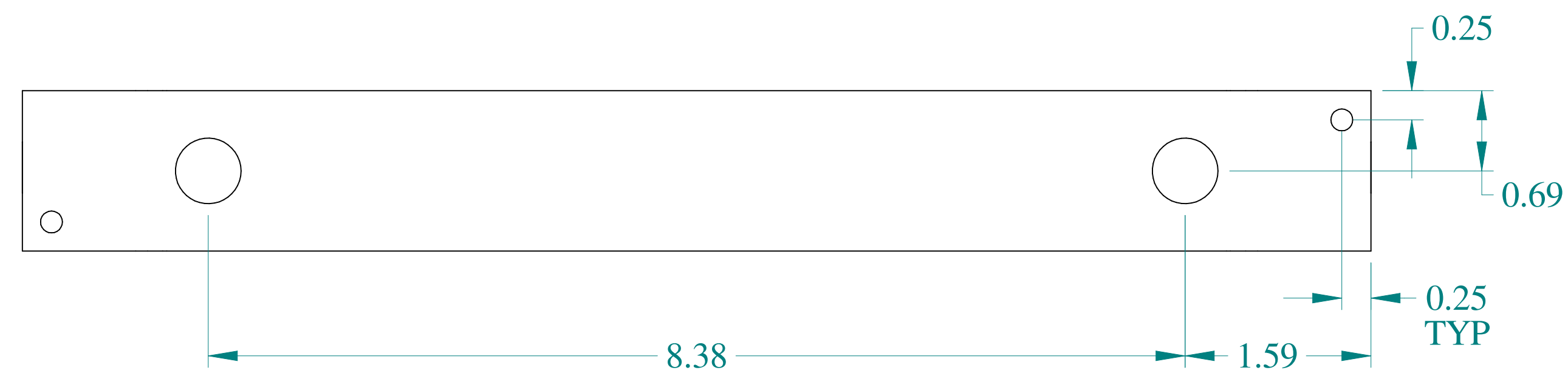
BOTTOM VIEW
