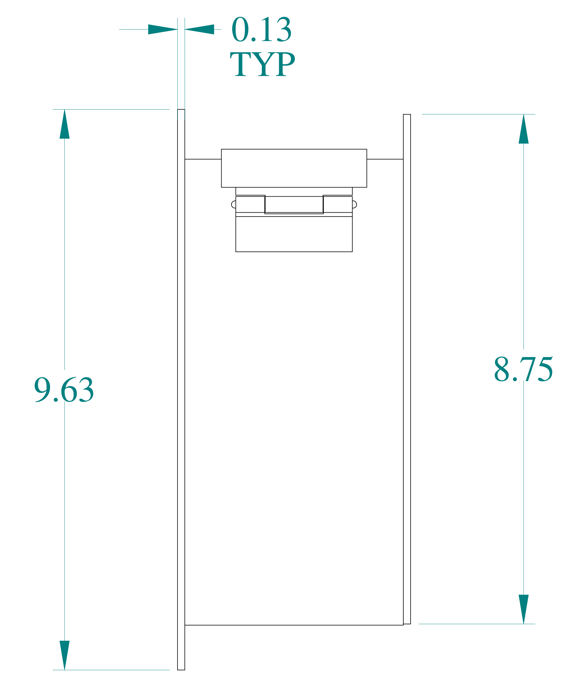
BACK VIEW
