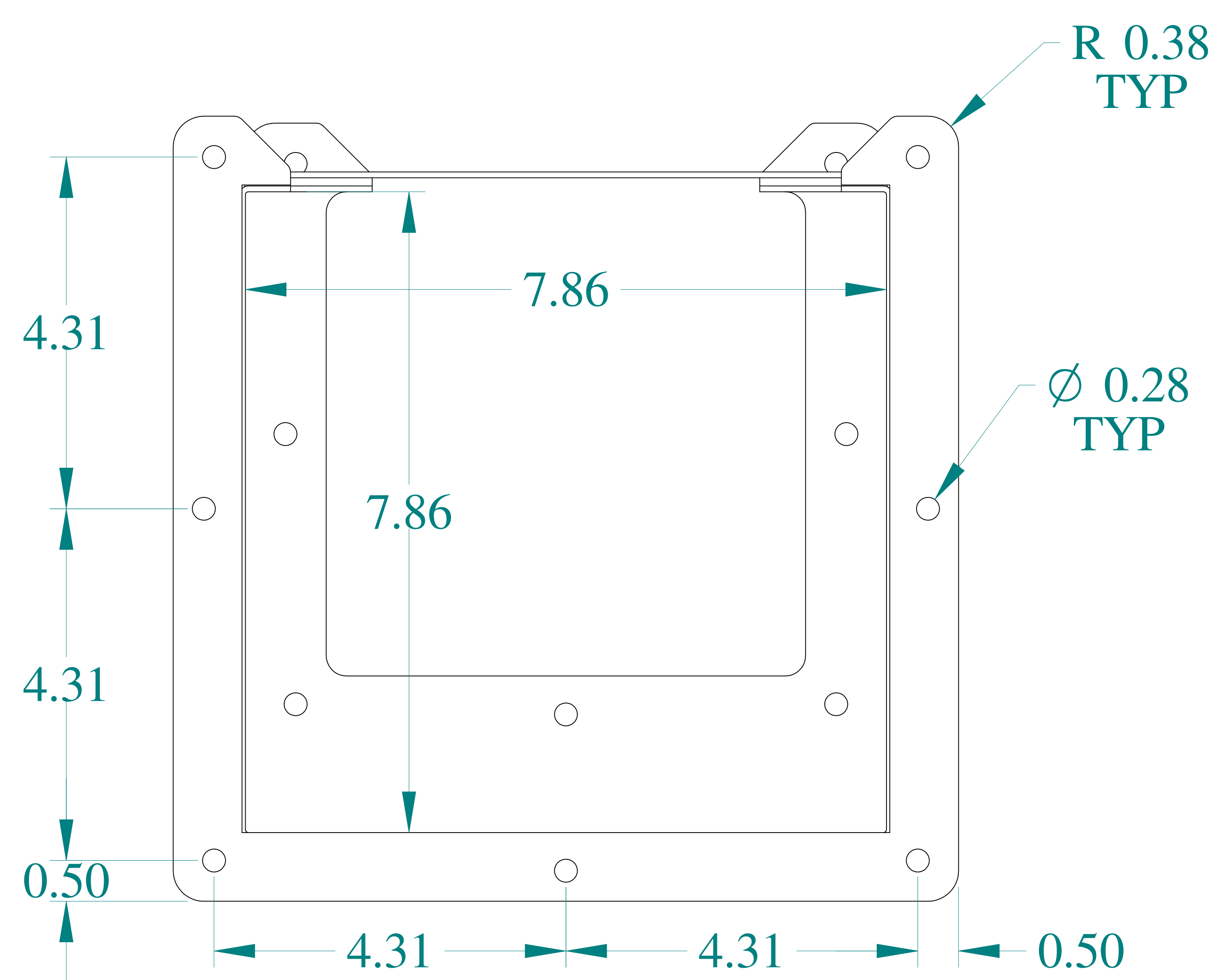
SIDE VIEW
