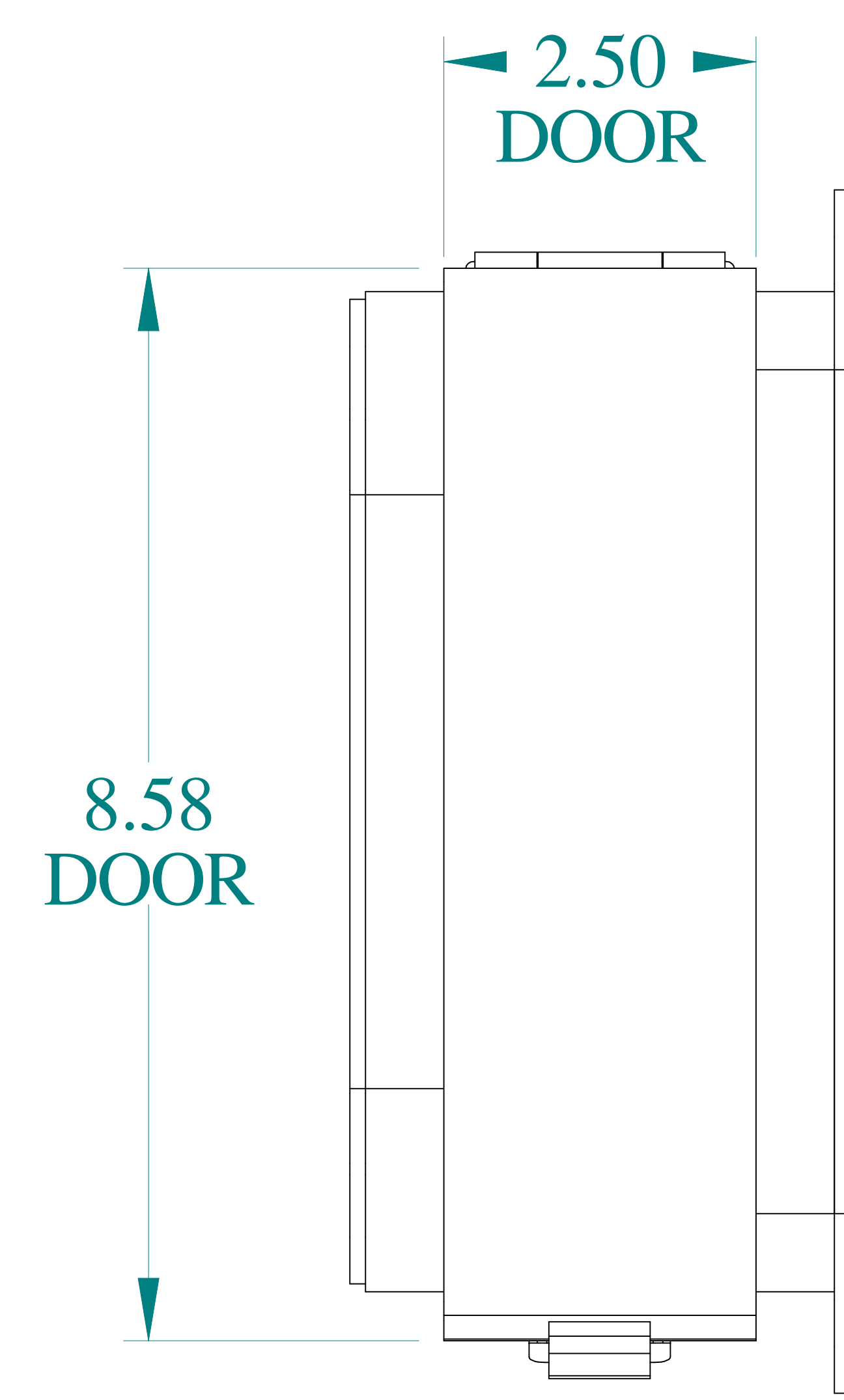
TOP VIEW
