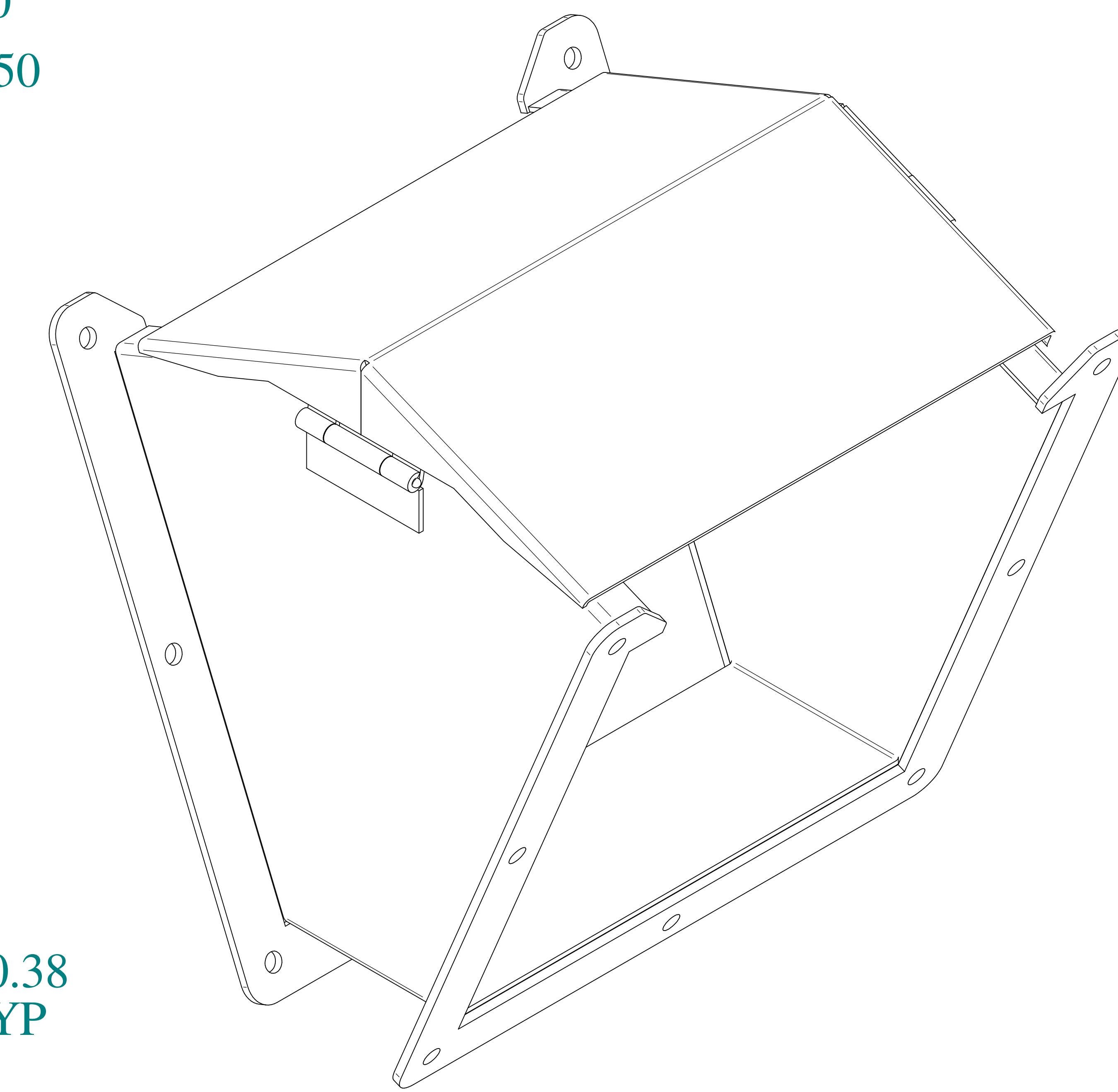
ISOMETRIC VIEWS
