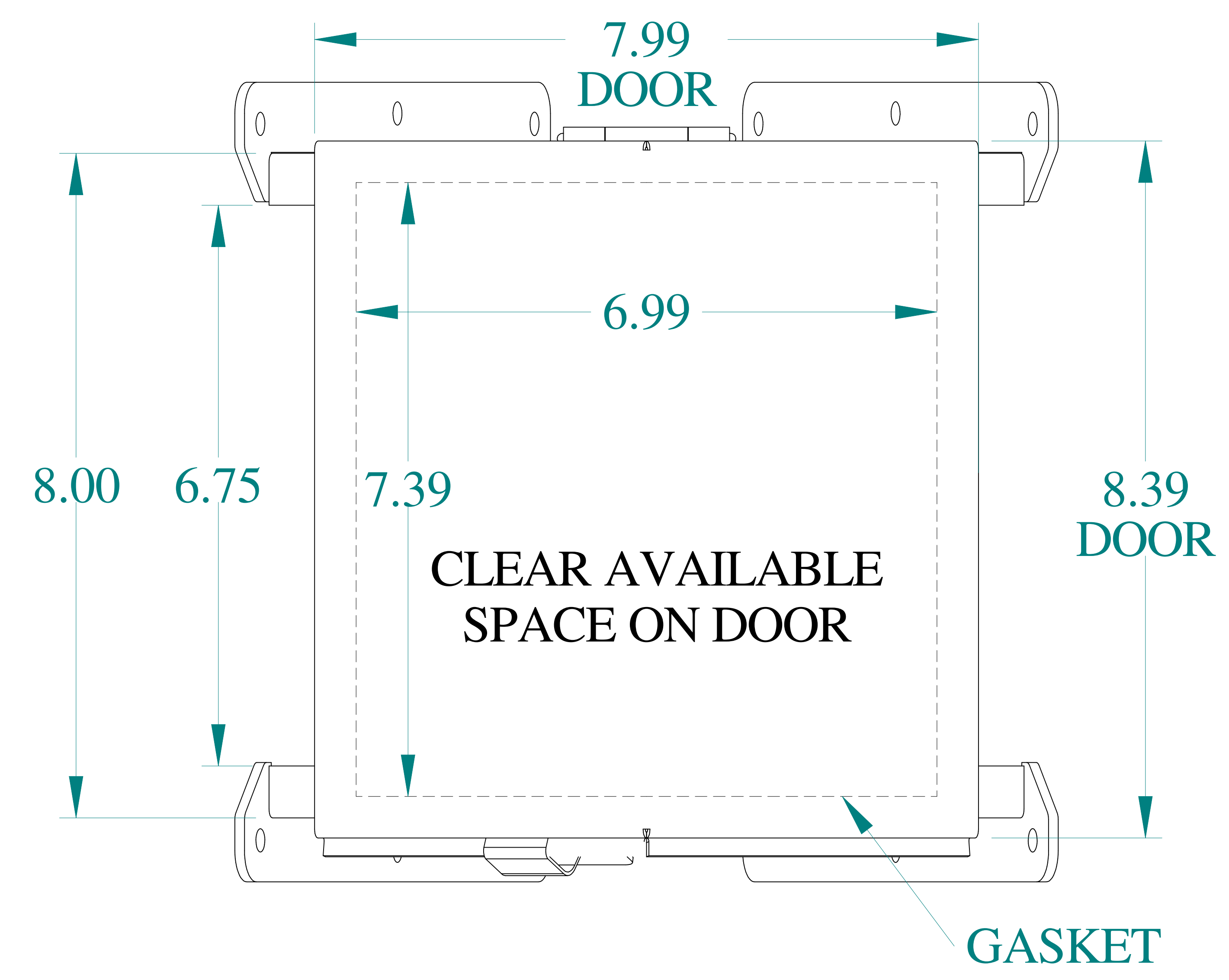
TOP VIEW
