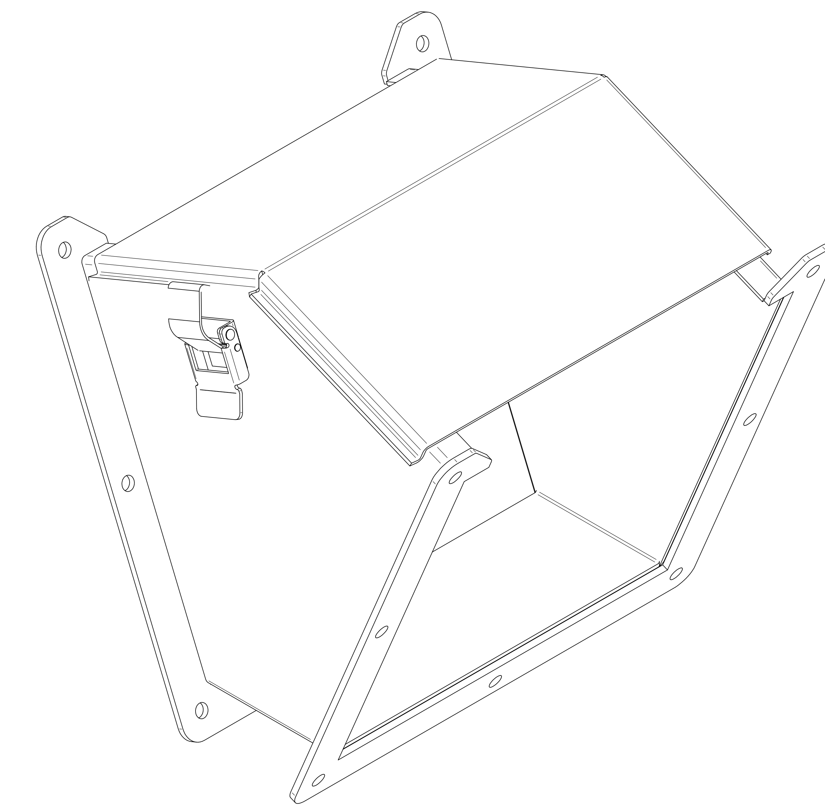
ISOMETRIC VIEWS
