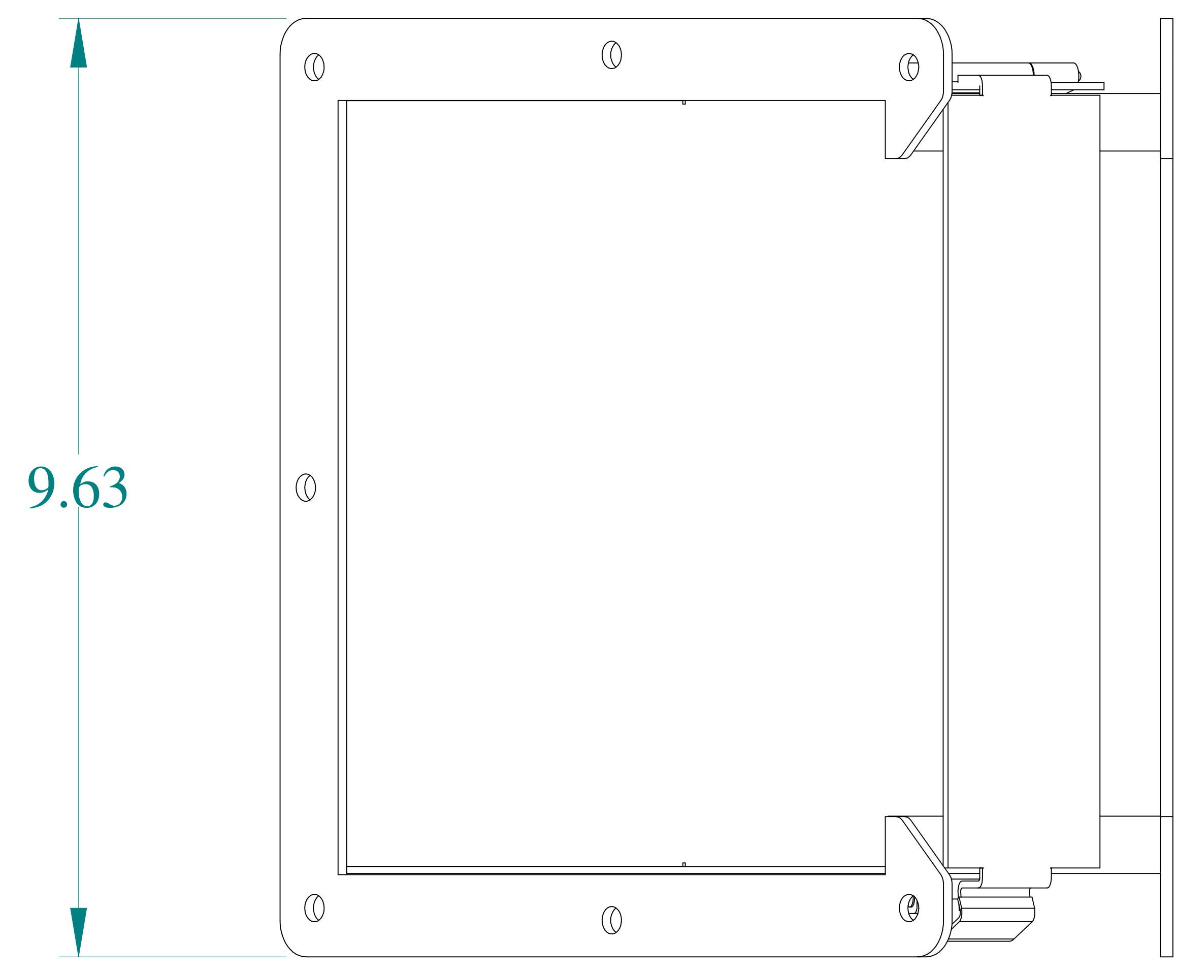
TOP VIEW
