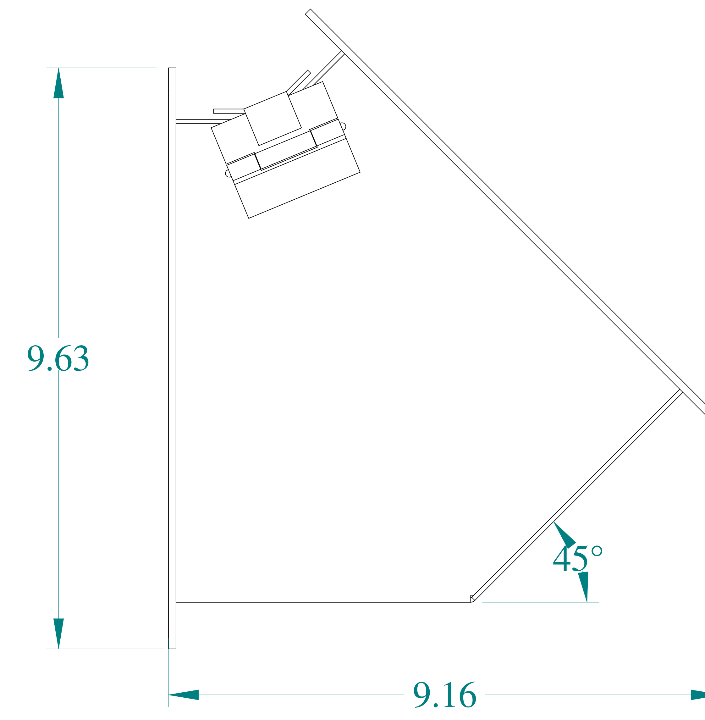
BACK VIEW
