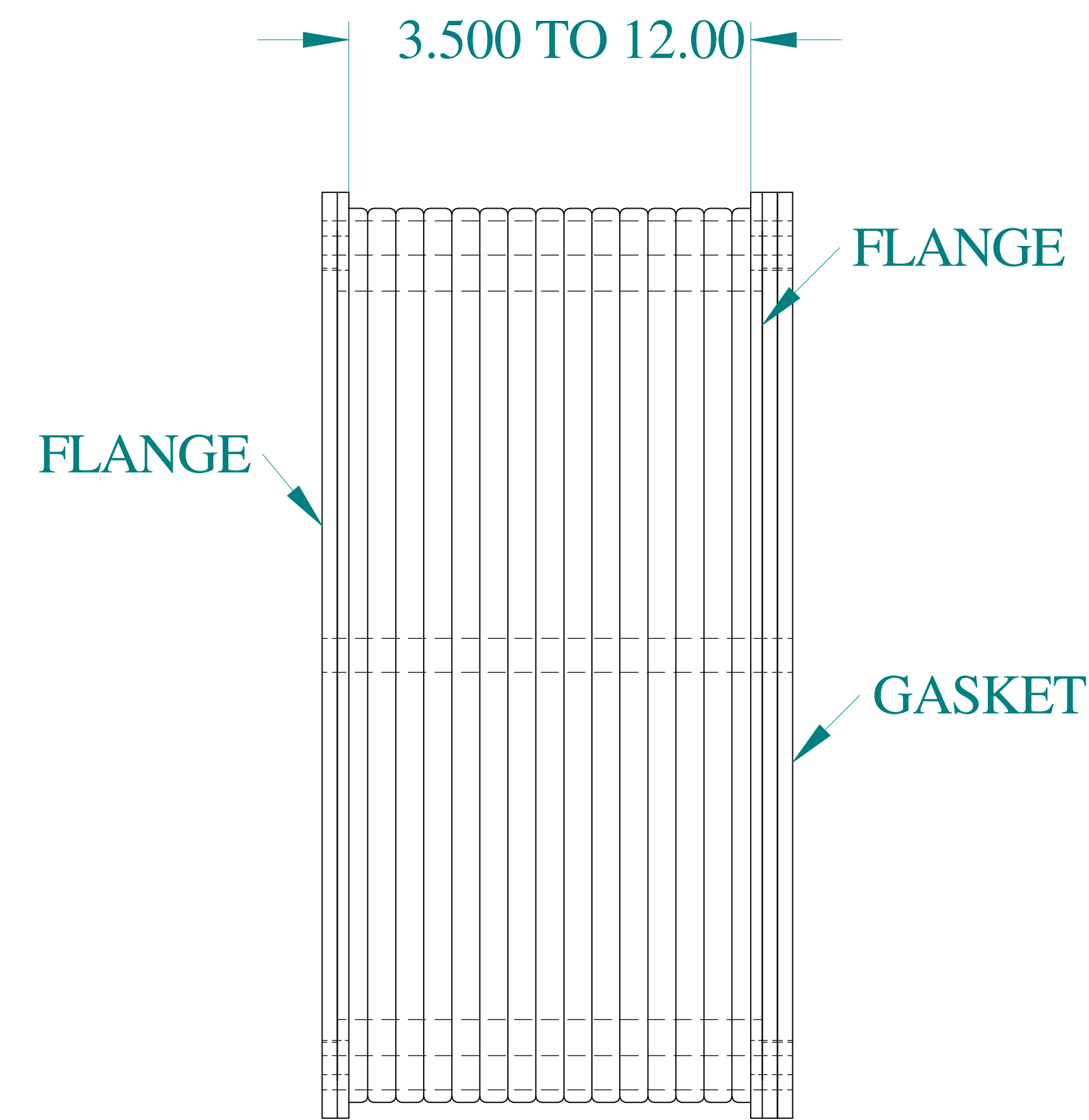
FRONT VIEW
