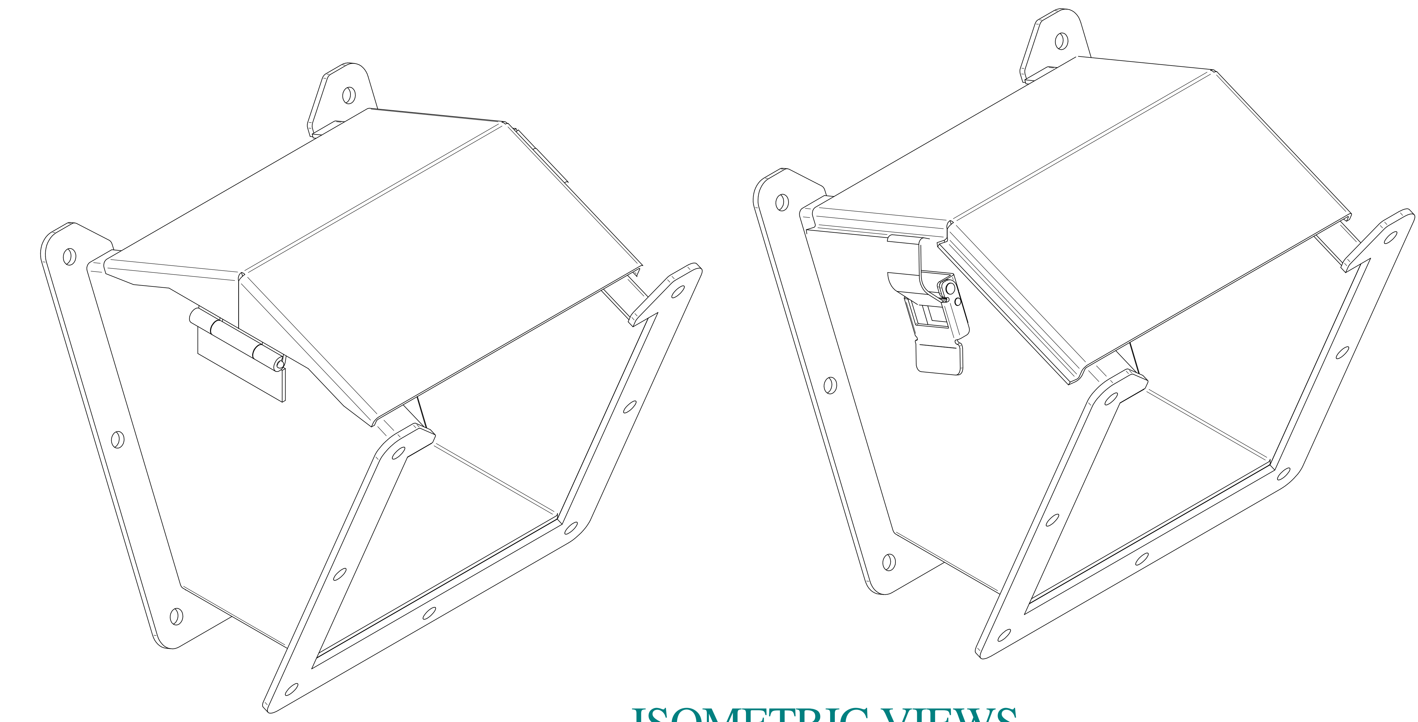
ISOMETRIC VIEWS
