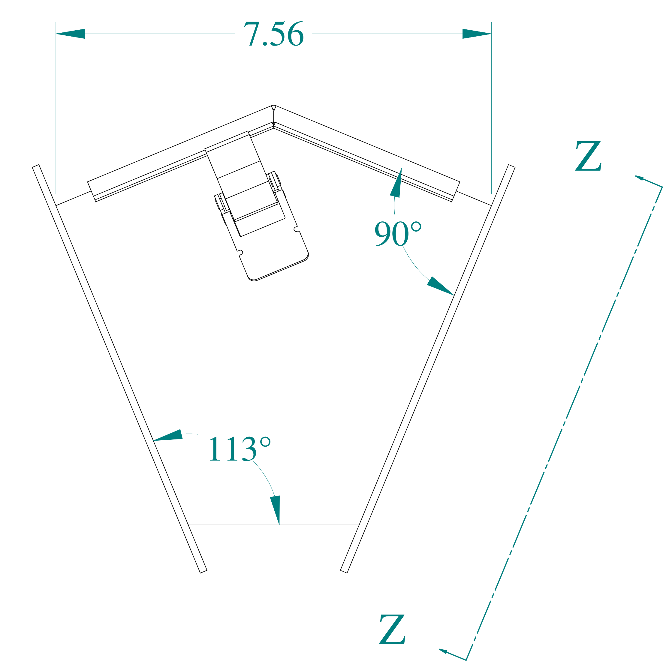
FRONT VIEW
