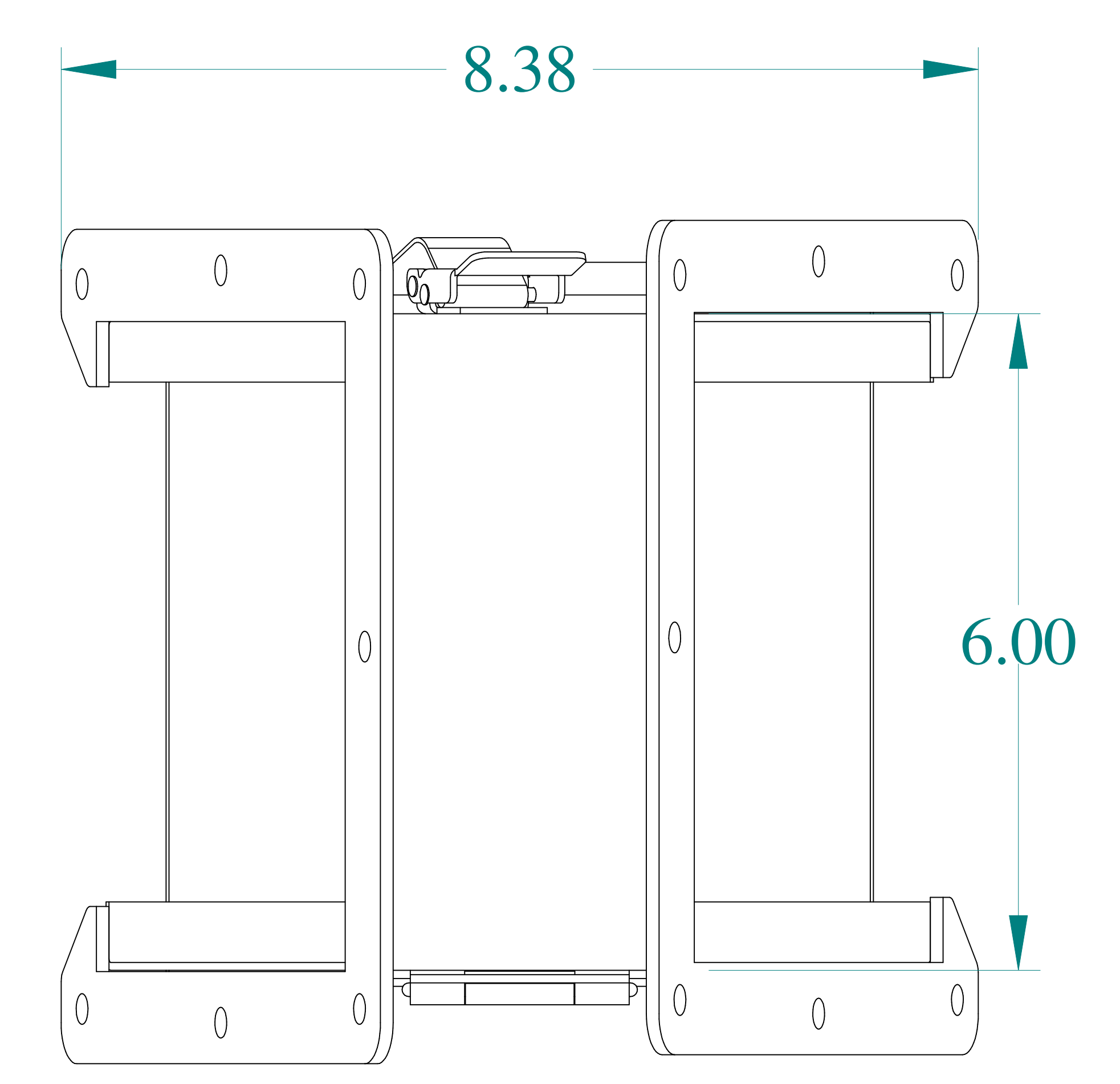
BOTTOM VIEW
