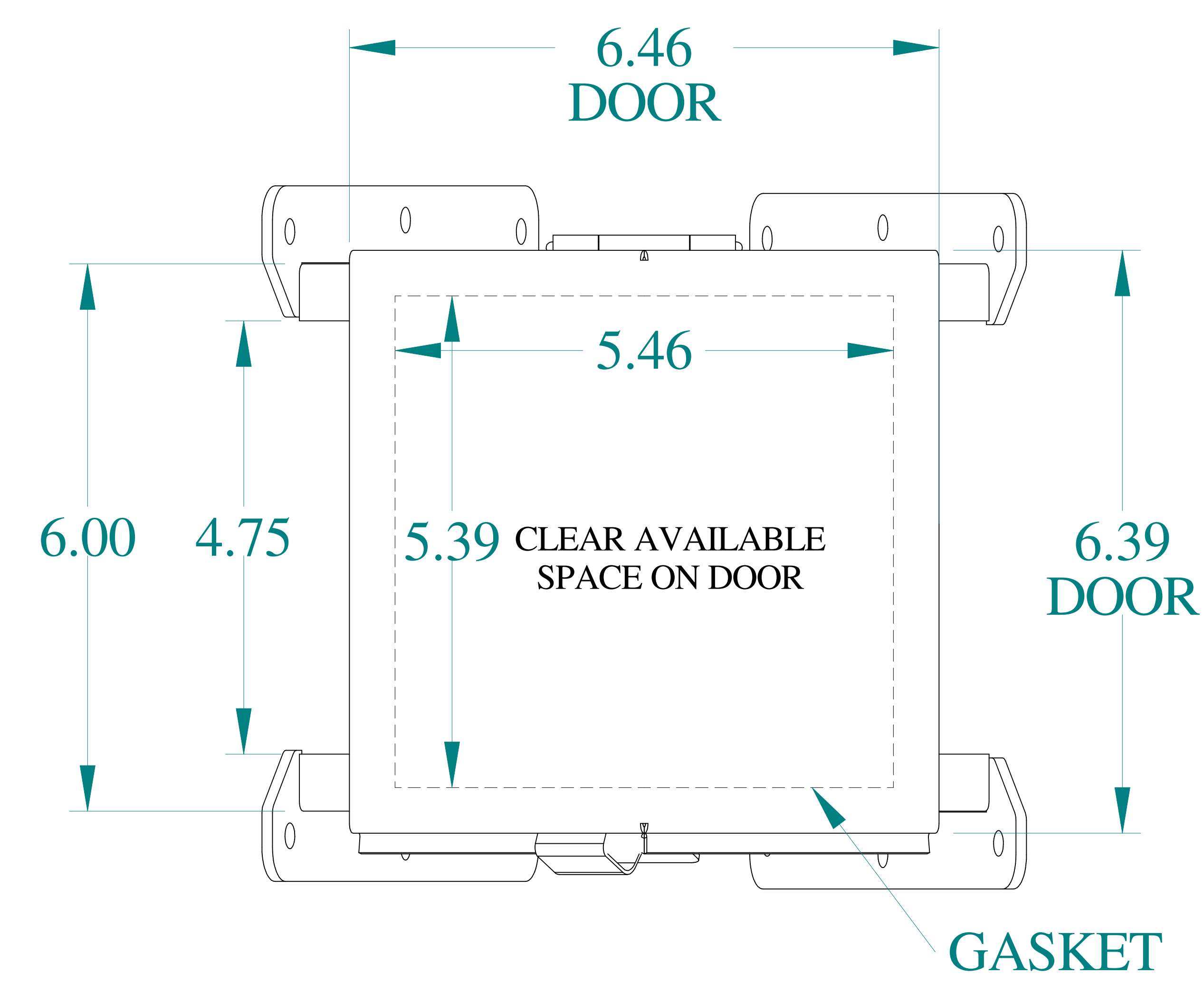
TOP VIEW
