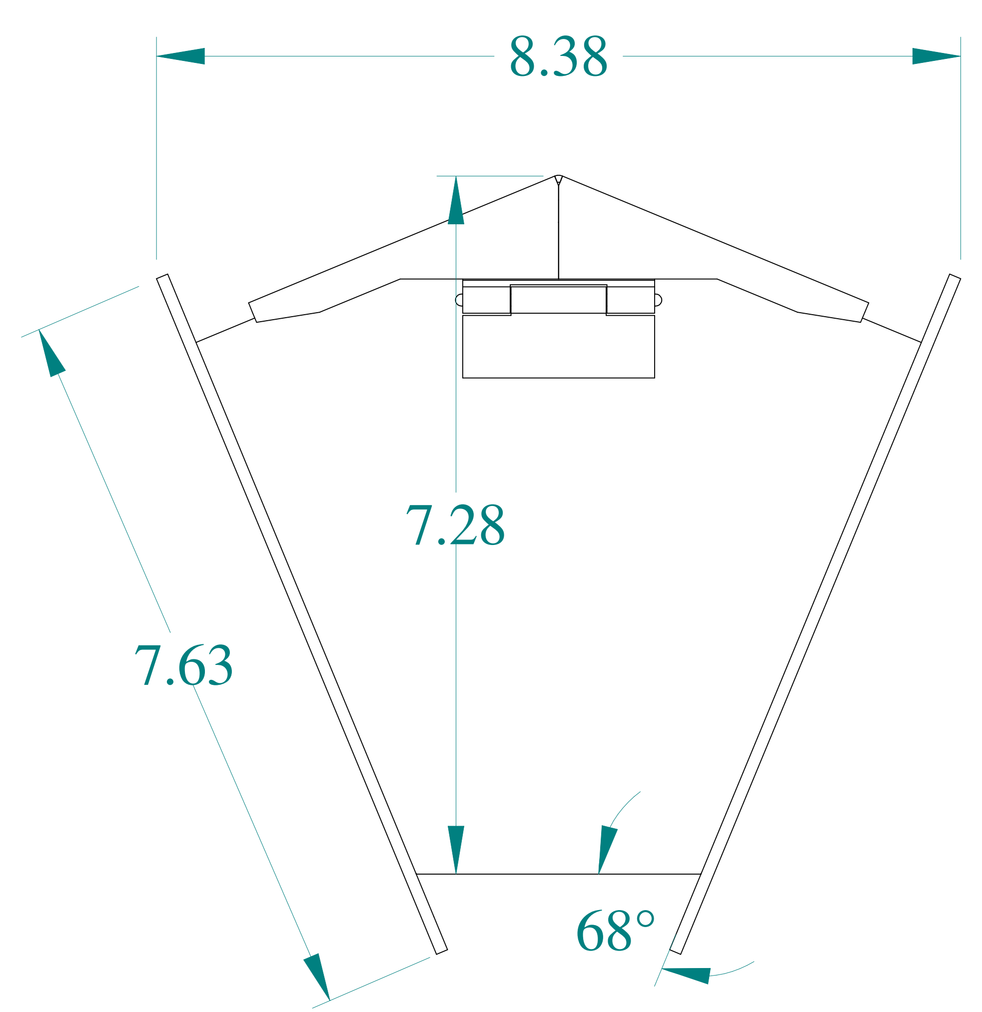
BACK VIEW
