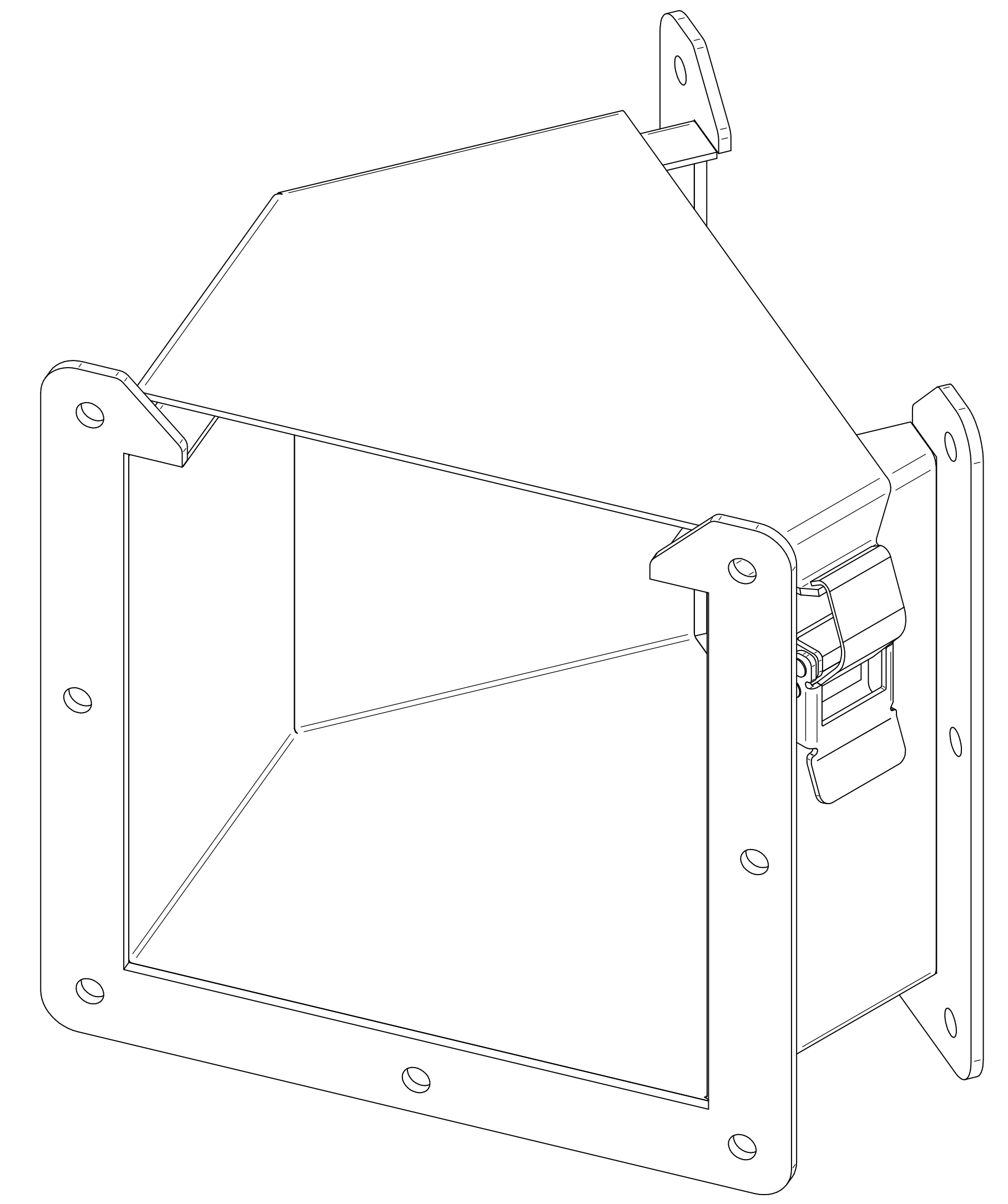
ISOMETRIC VIEWS
