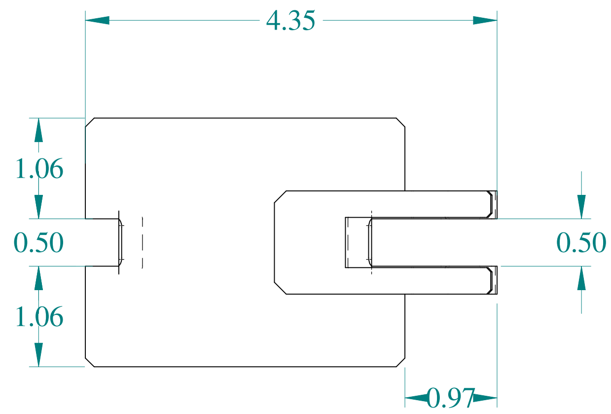
TOP VIEW
