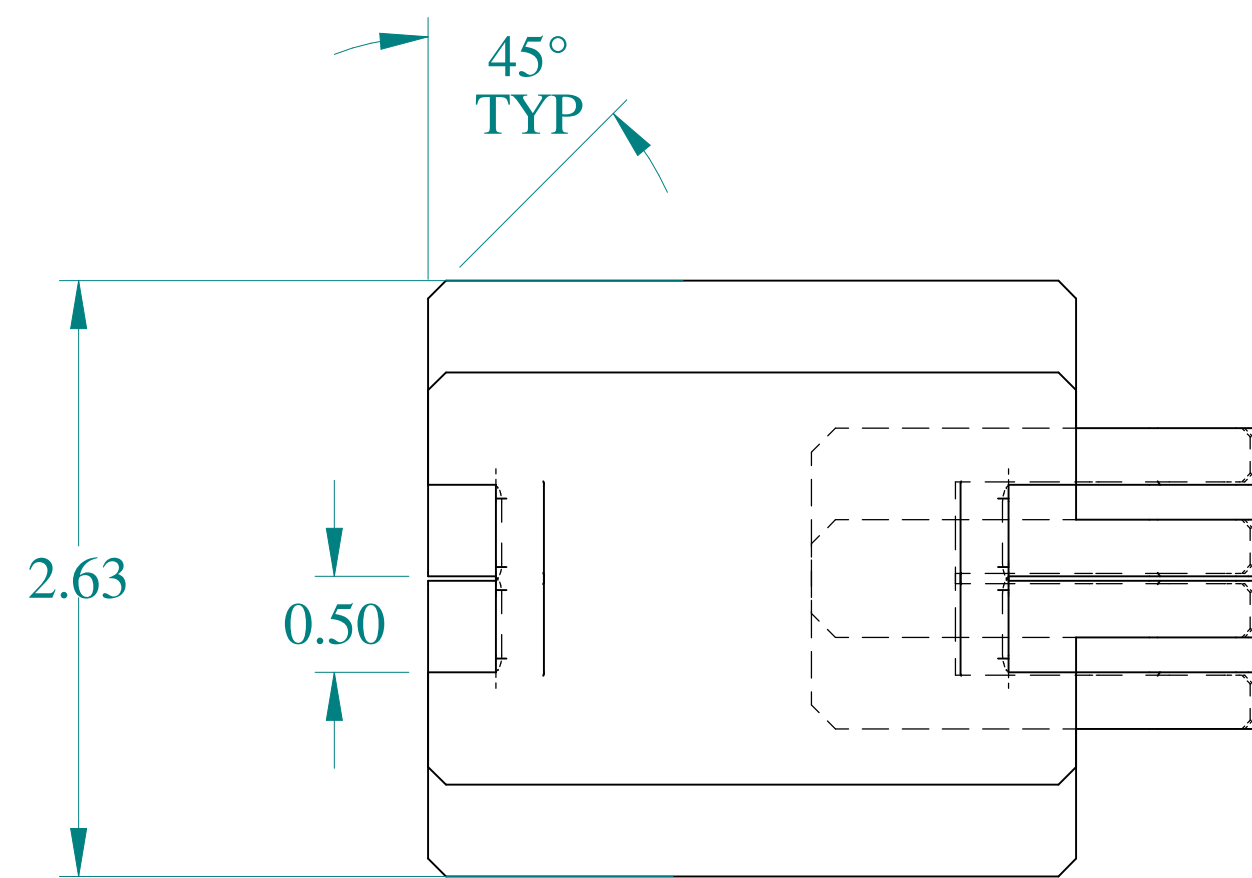
BOTTOM VIEW
