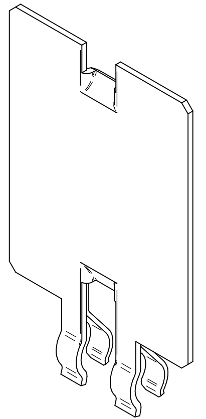
ISOMETRIC VIEWS
