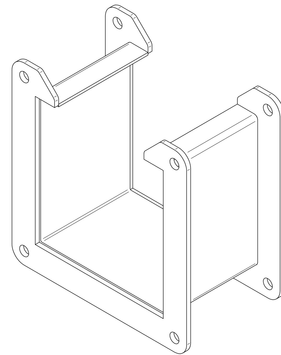
ISOMETRIC VIEWS
