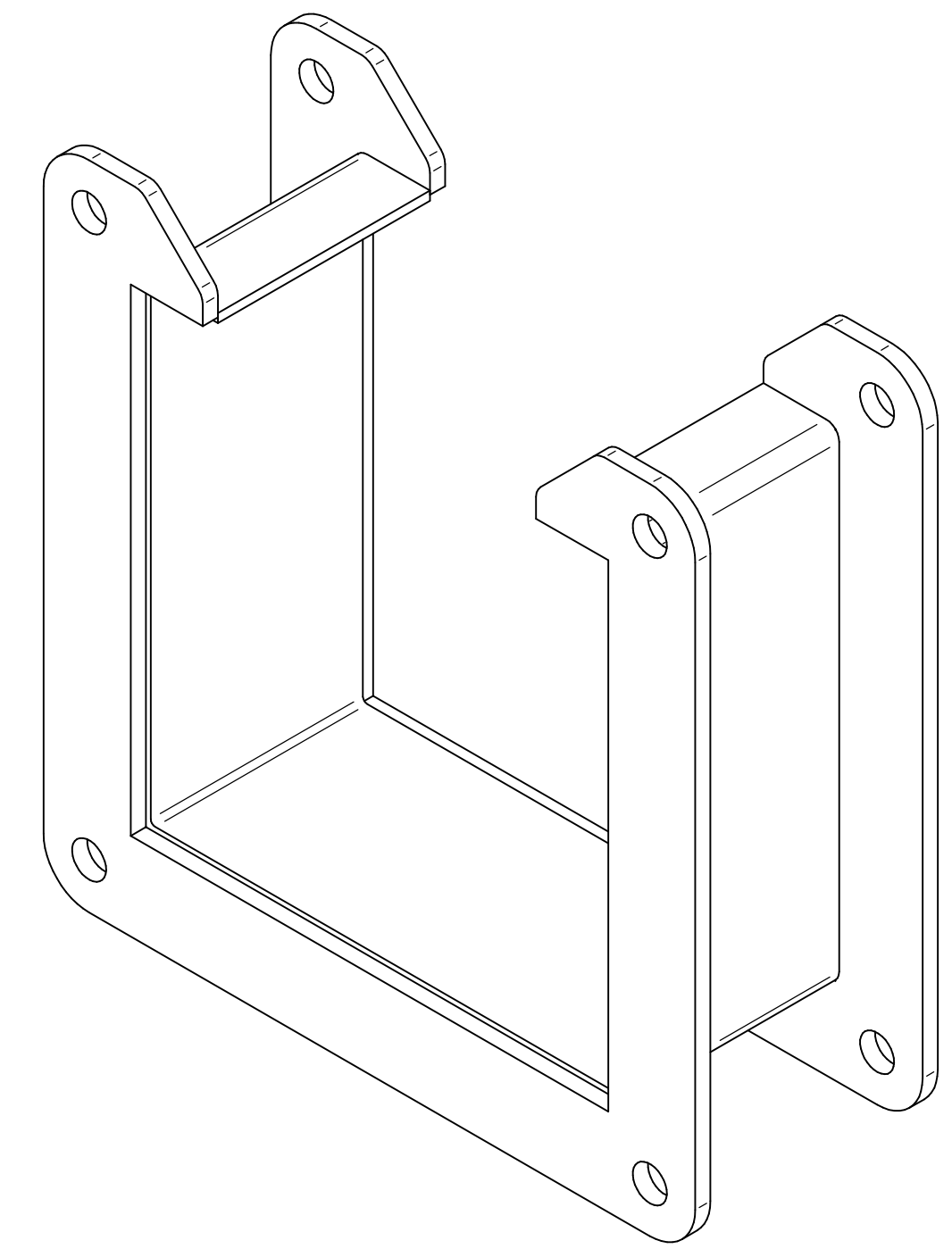
ISOMETRIC VIEWS
