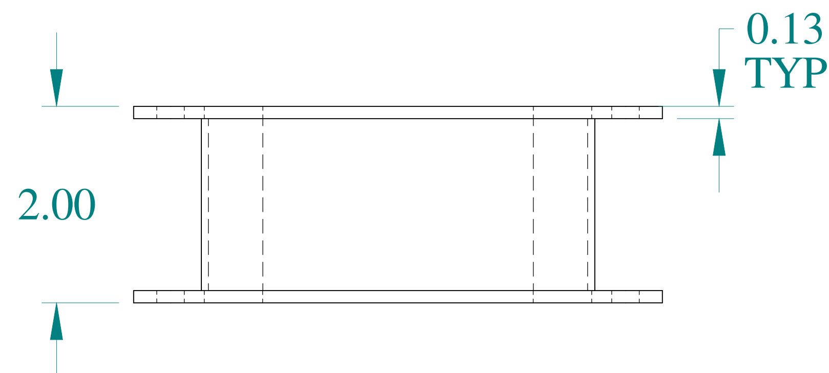
BOTTOM VIEW
