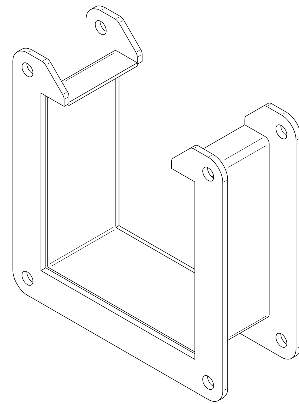
ISOMETRIC VIEWS
