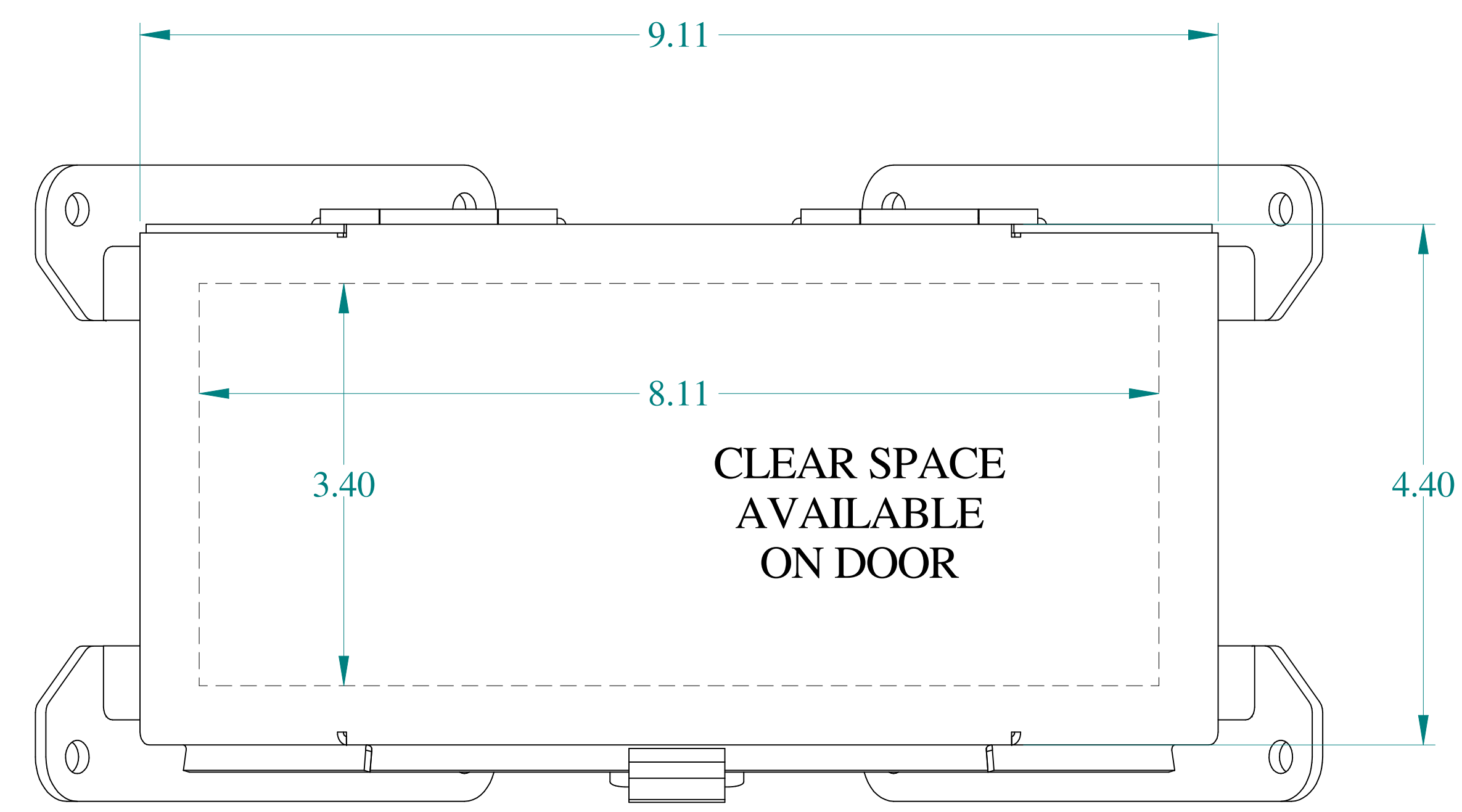
TOP VIEW
