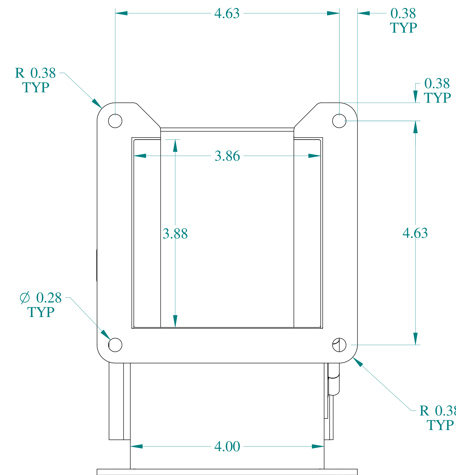
VIEW Z-Z
