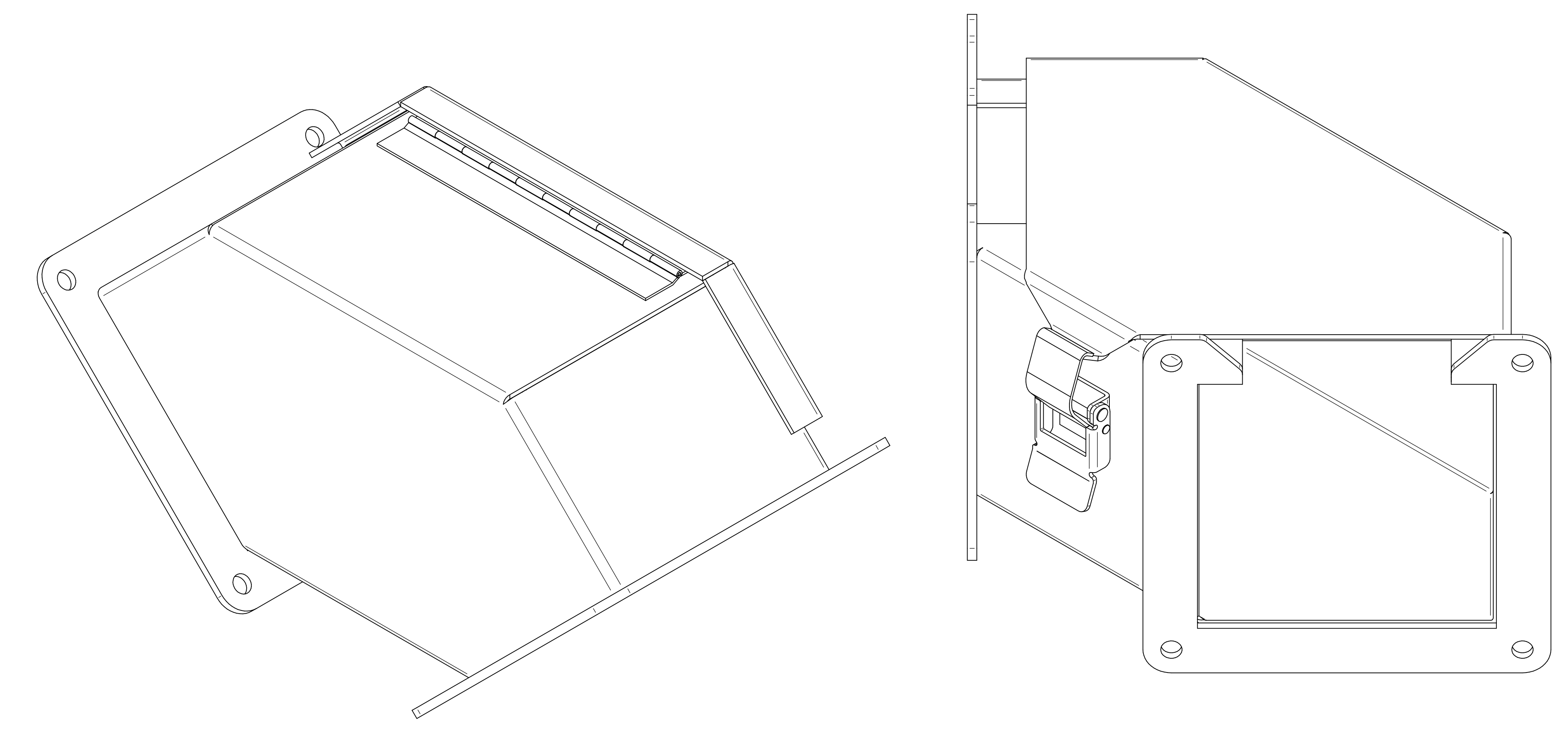
ISOMETRIC VIEWS
