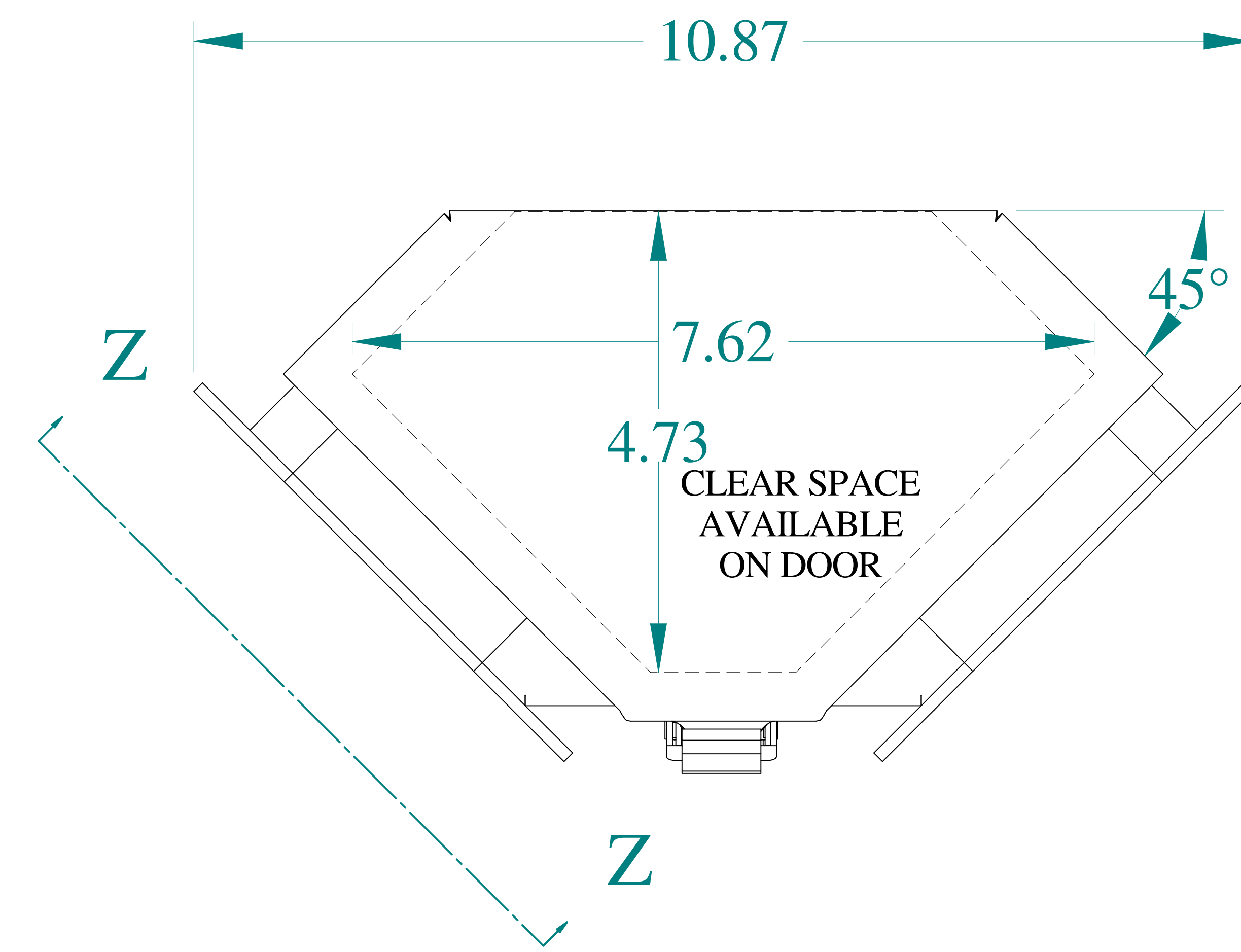
TOP VIEW
