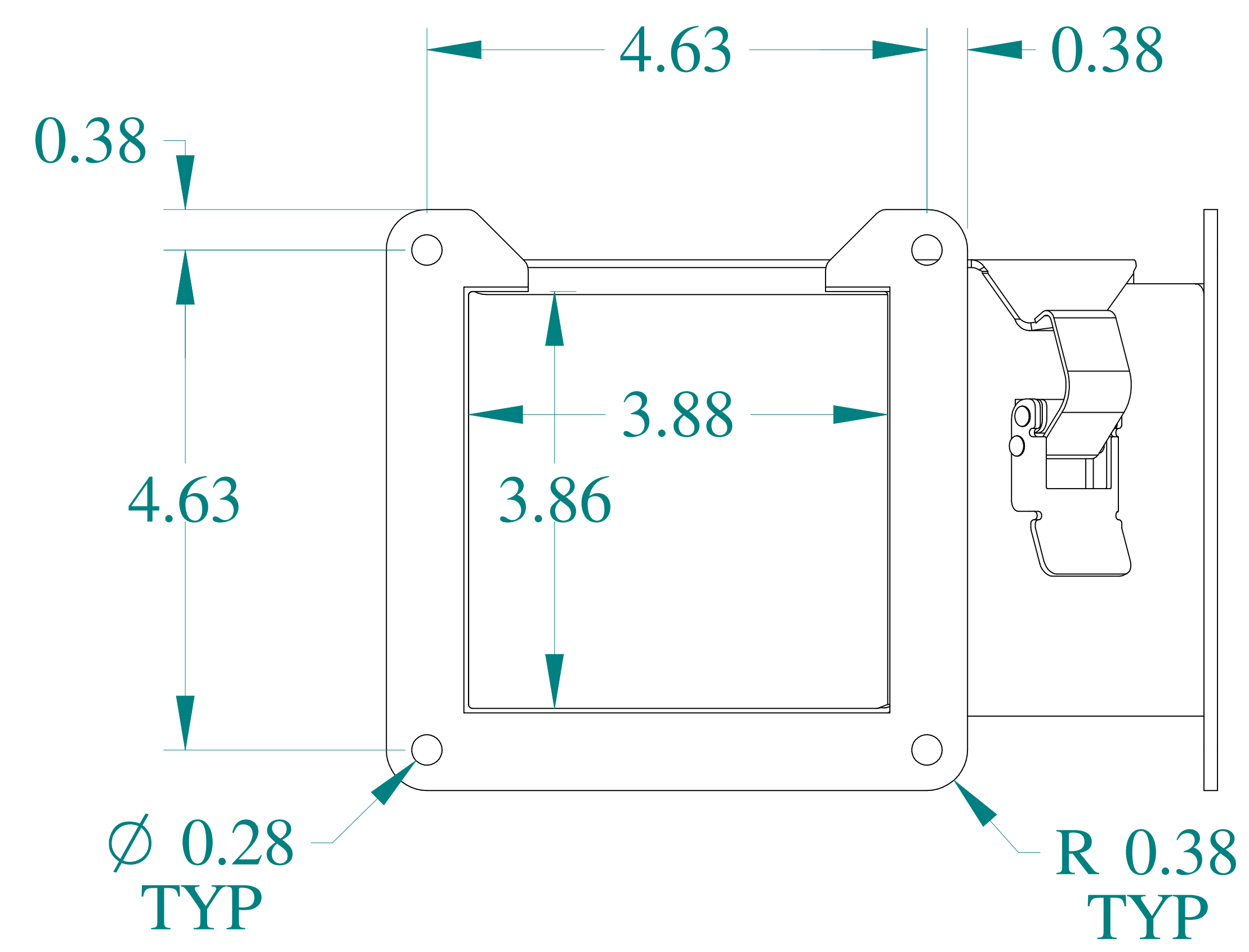
VIEW Z-Z
