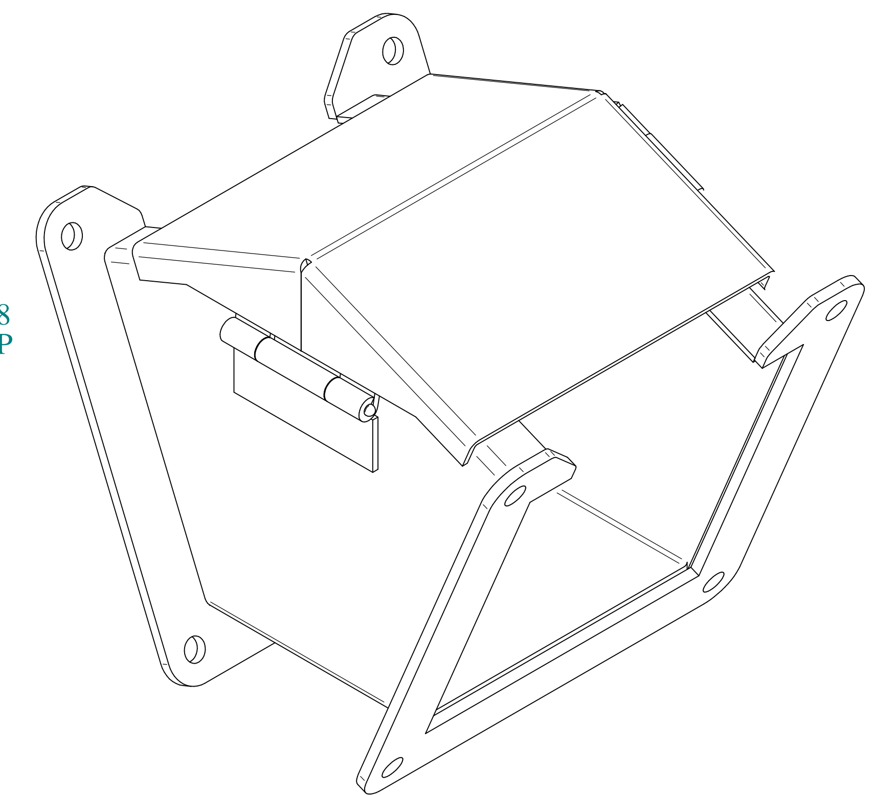
ISOMETRIC VIEWS
