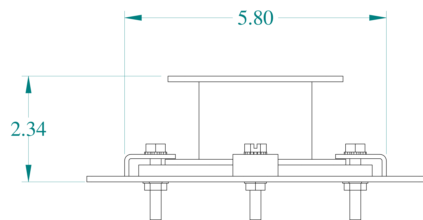
BOTTOM VIEW
