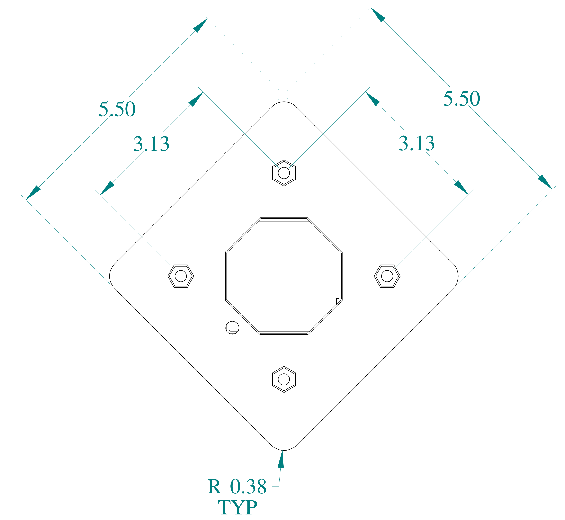
BACK VIEW
