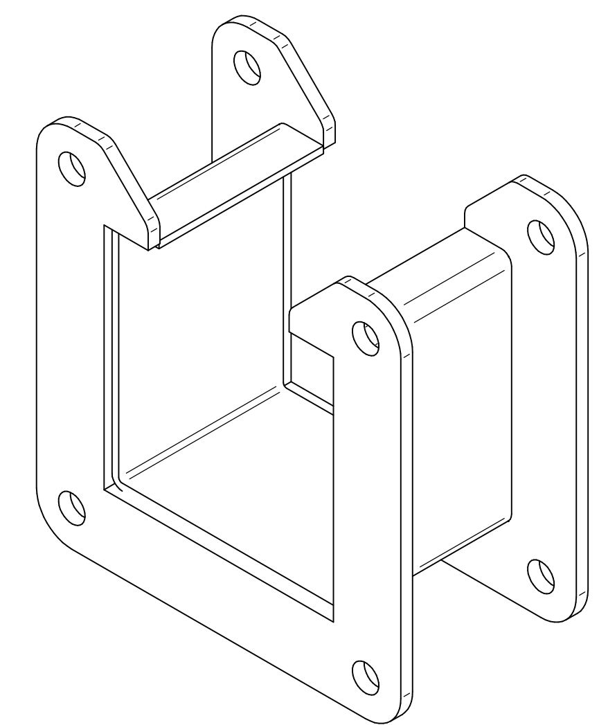
ISOMETRIC VIEWS
