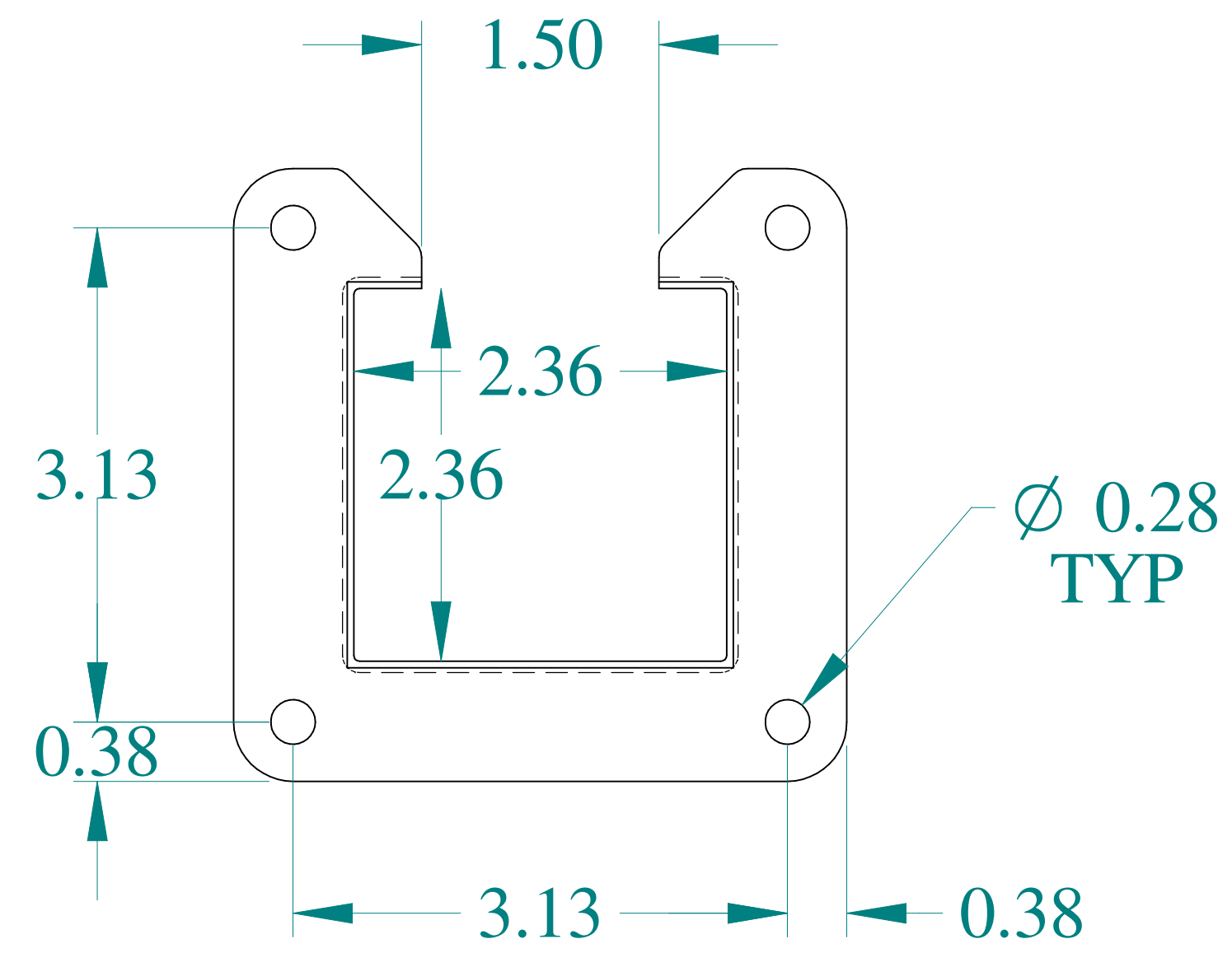
FRONT VIEW
