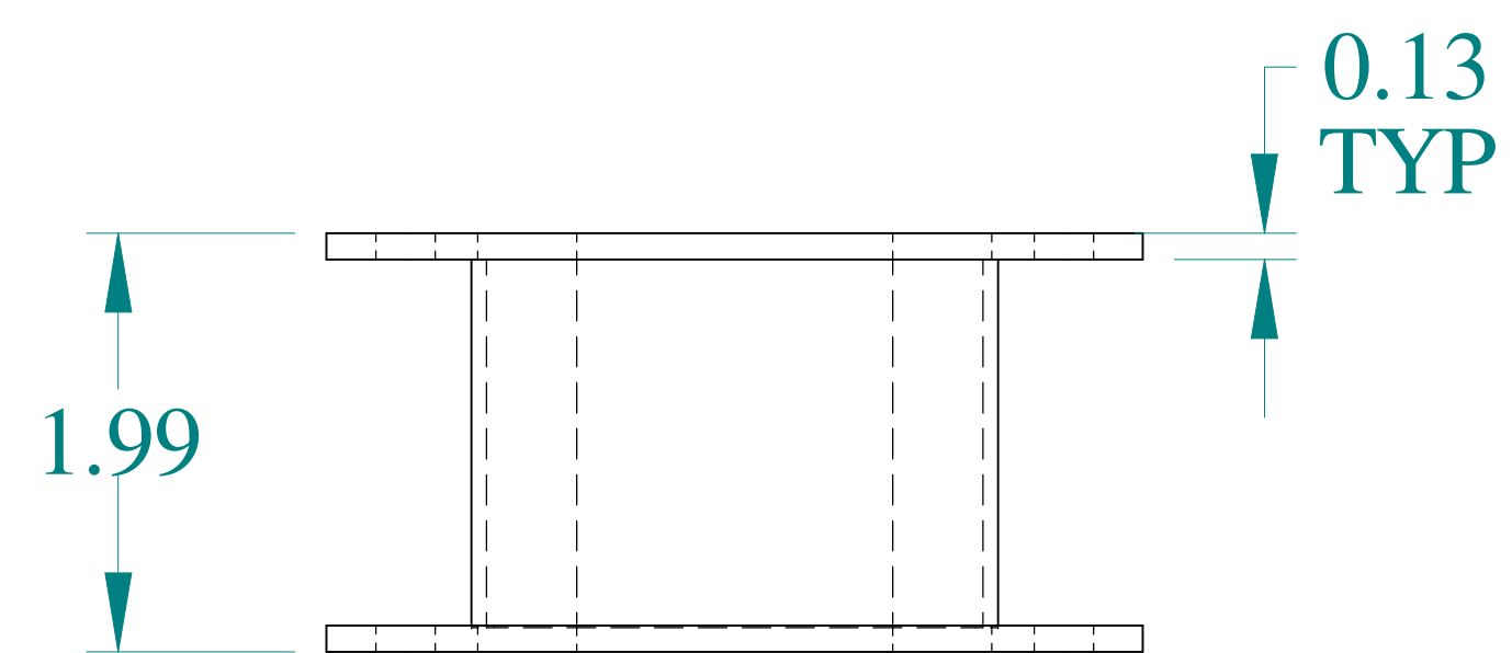
BOTTOM VIEW
