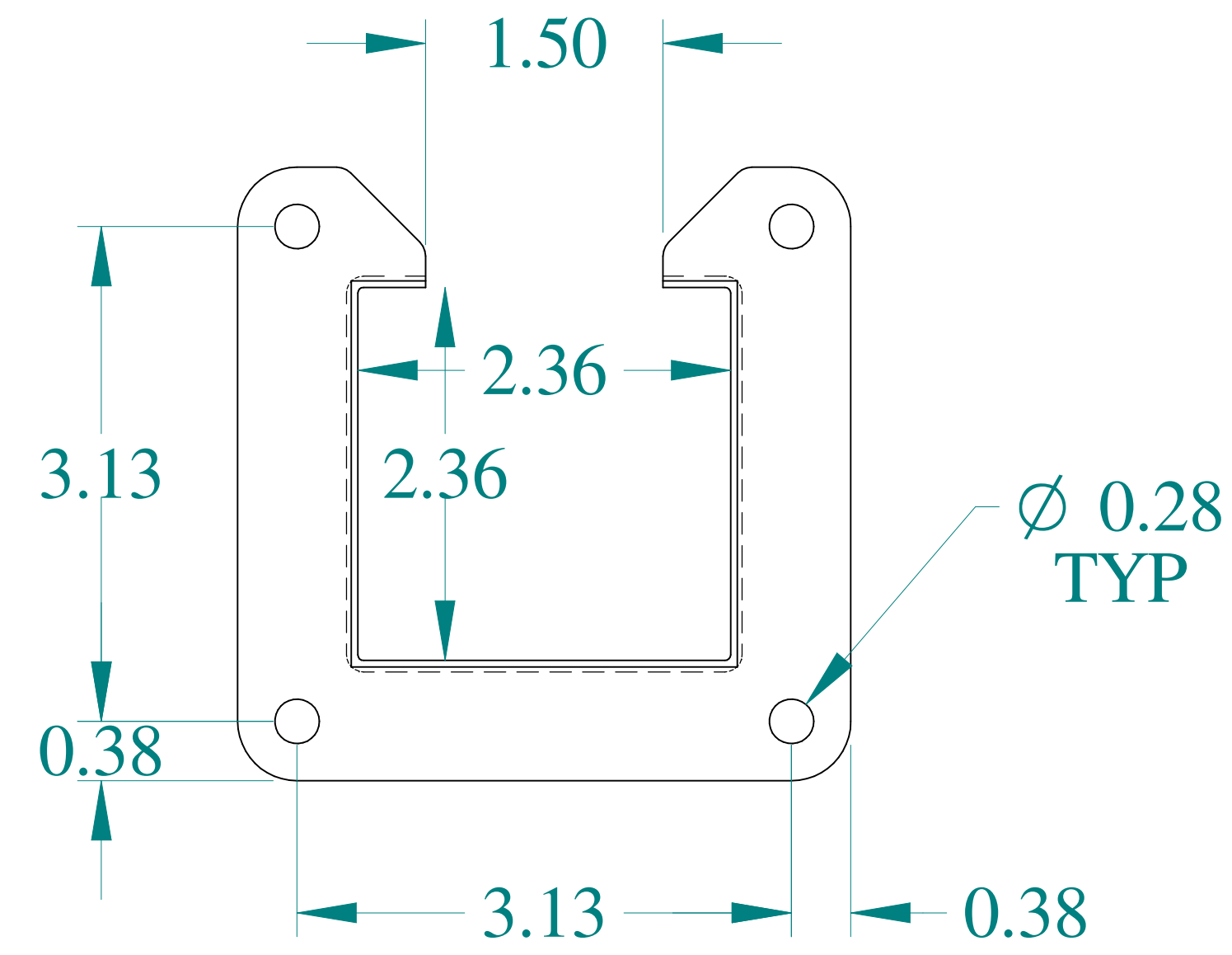
FRONT VIEW
