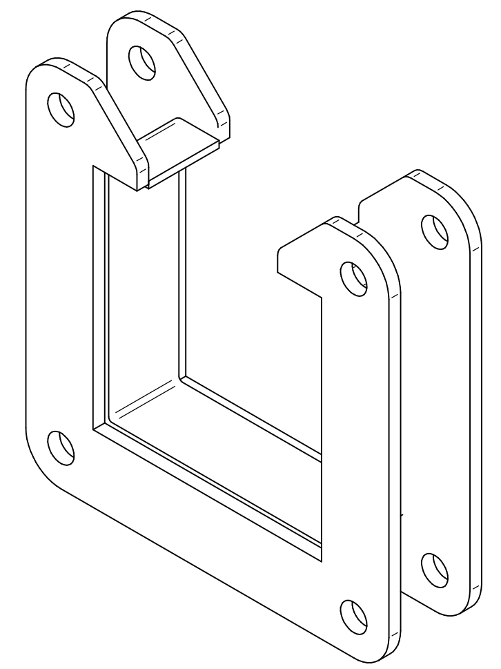
ISOMETRIC VIEWS
