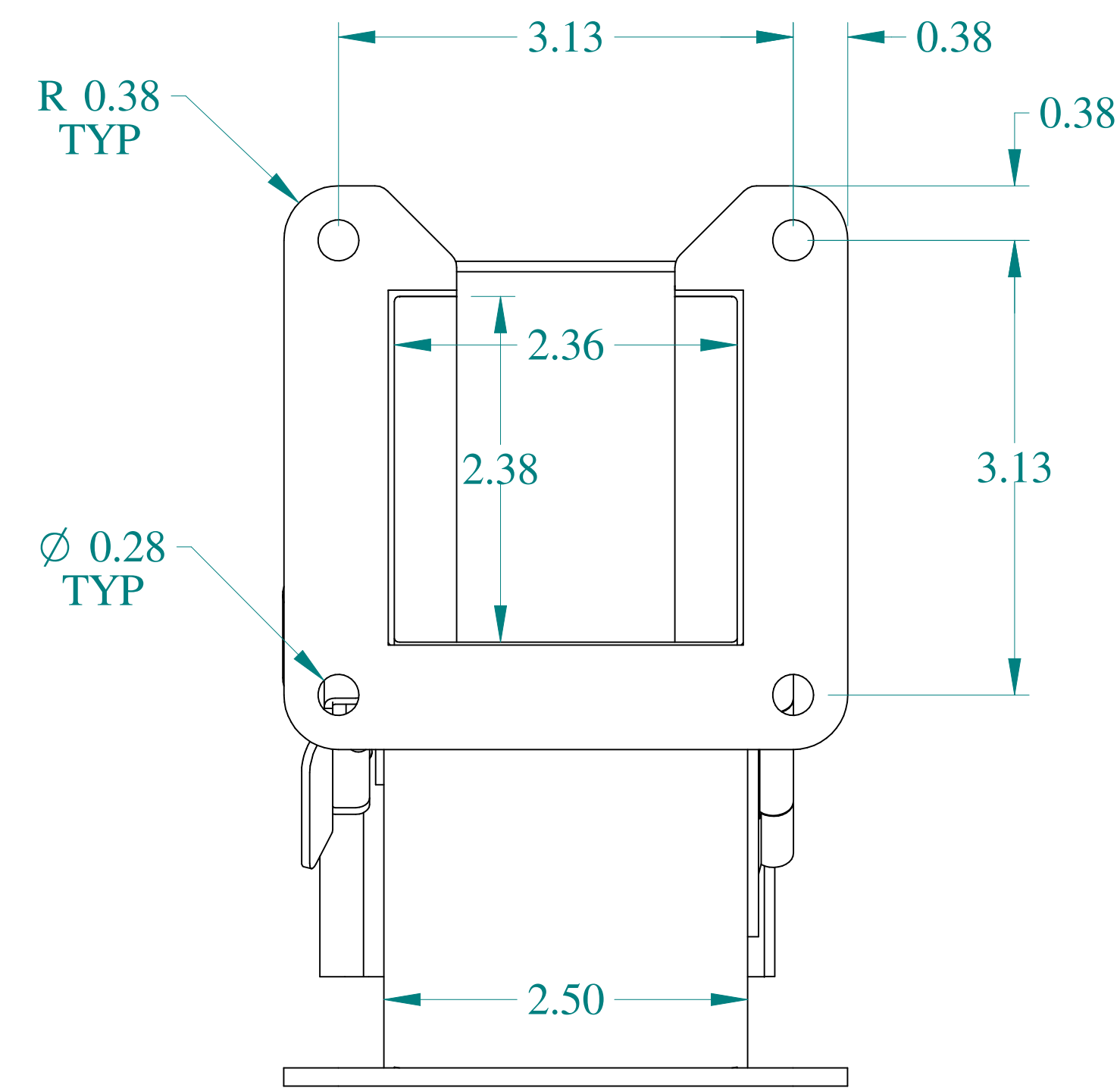
VIEW Z-Z
