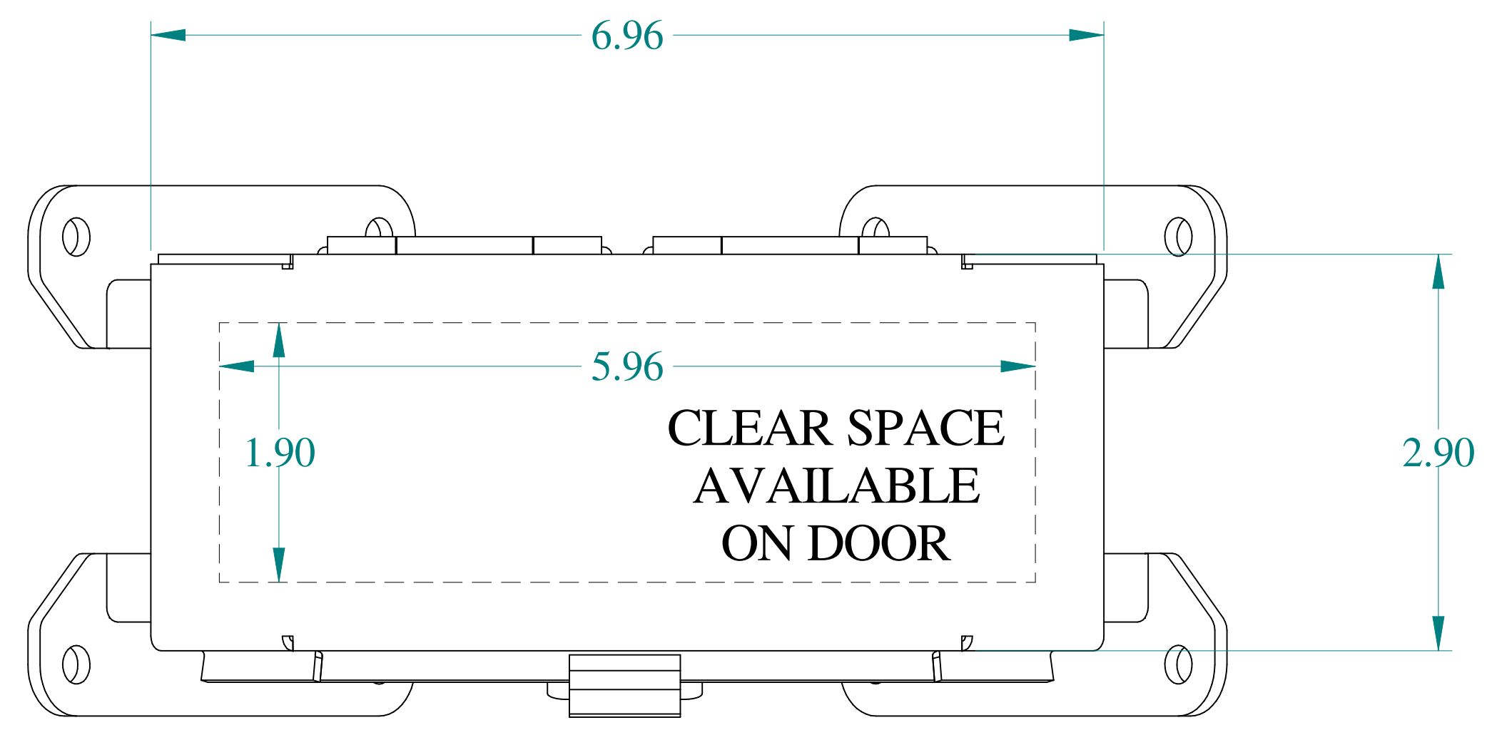
TOP VIEW
