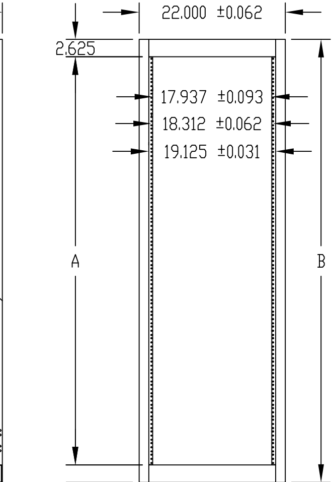
FRONT VIEW
