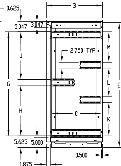
SECTION 'A-A' (LESS PANEL MTG. RAILS)
