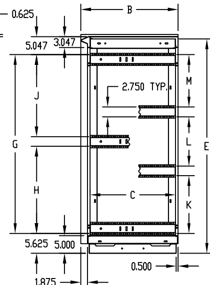
SECTION 'A-A' (LESS PANEL MTG. RAILS)
