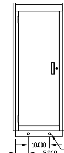
REAR VIEW
