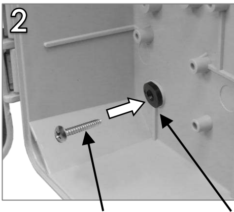
Mounting Screw
