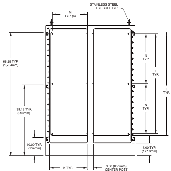
FRONT VIEW WITH DOORS REMOVED
