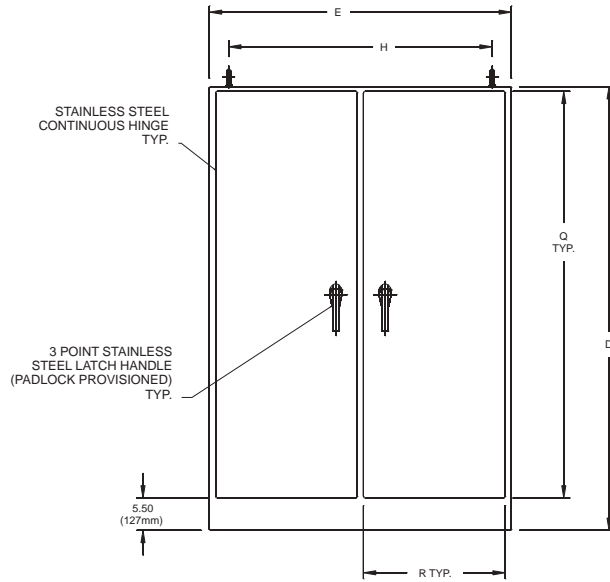
FRONT VIEW WITH DOORS
