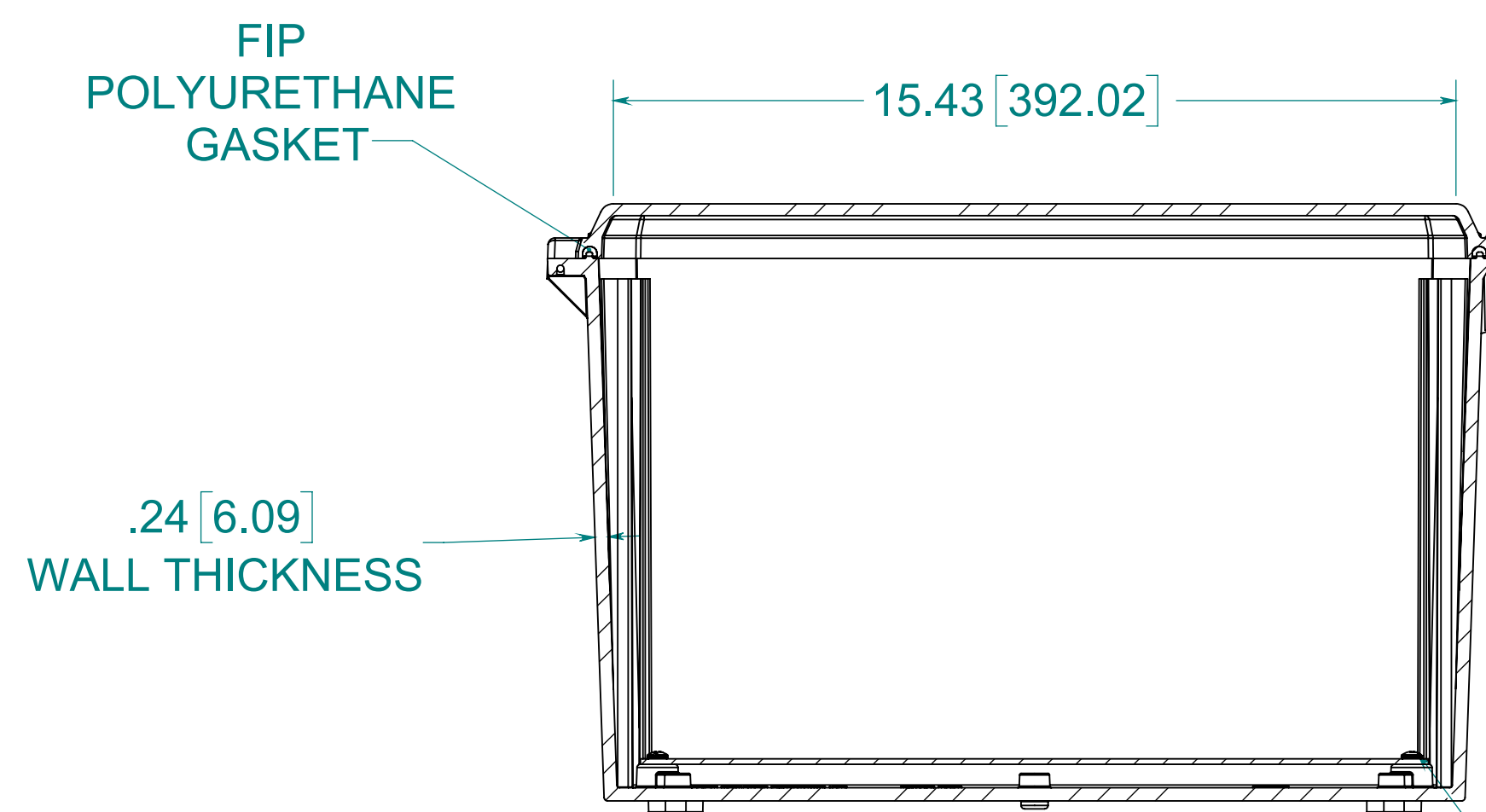
SECTION B-B
